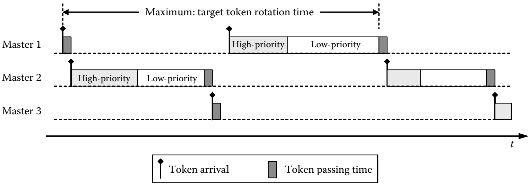
FIGURE 20.16 Token passing in PROFIBUS.
