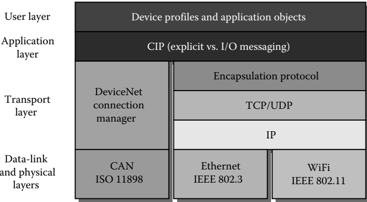
FIGURE 26.2 Protocol stack of CIP-based networks.
