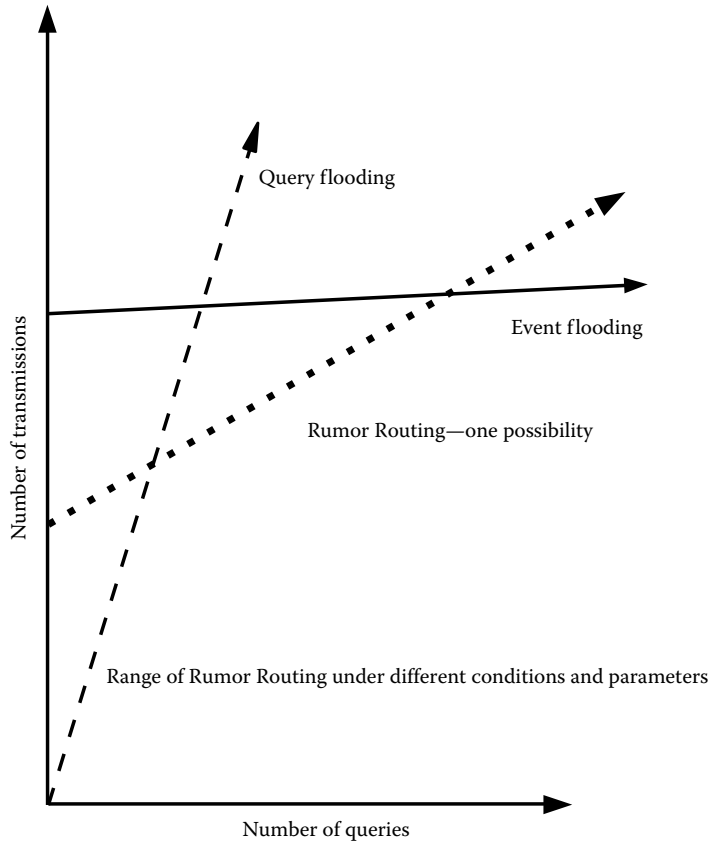
FIGURE 7.3 Rumor Routing compared to query flooding and event flooding. (Redrawn from Braginsky, D. and Estrin, D., Rumor algorithm for sensor networks, in Proceedings of the First Workshop on Sensor Networks and Applications (WSNA) , Atlanta, GA, October 2002.)
