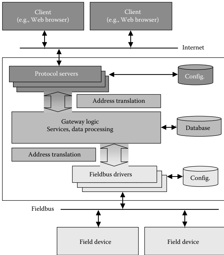
FIGURE 20.28 Network topology for a gateway-based interconnection and general architecture of a gateway.
