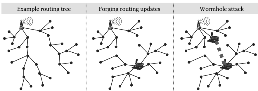
FIGURE 10.3 Attacks on breadth first search routing.
