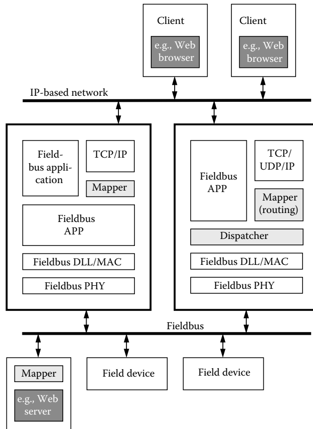
FIGURE 20.26 Protocol and software structure for IP tunneling over a fieldbus.
