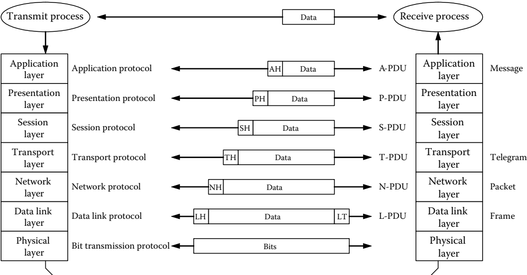
FIGURE 20.4 Layer structure of the OSI model and data frame formation.
