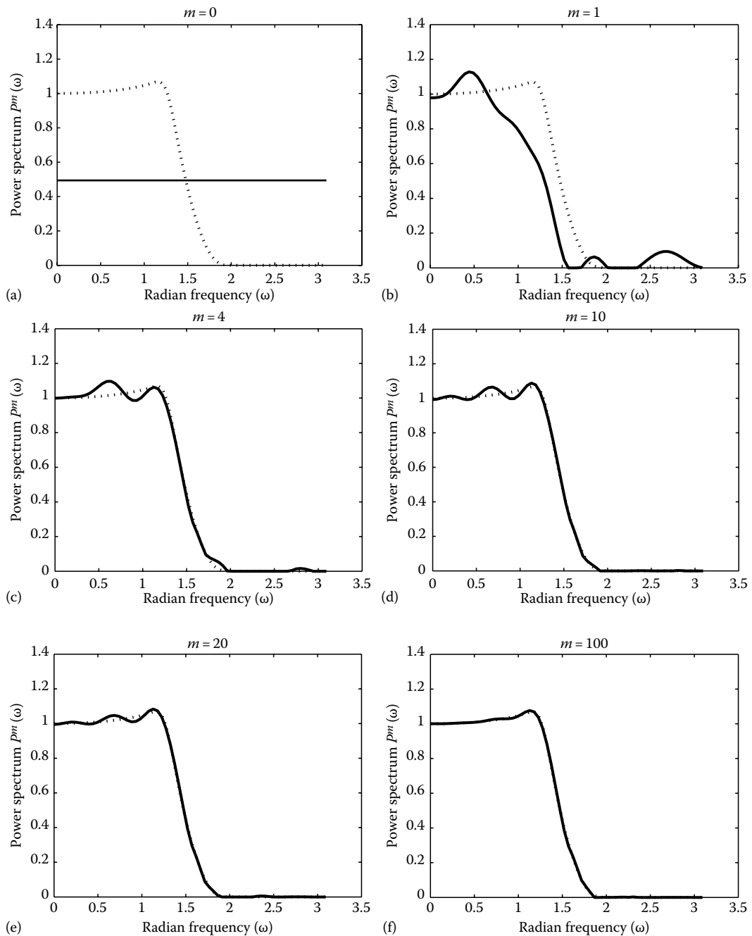
FIGURE 9.7 Ring Algorithm convergence results. In each figure, the dashed curve shows the source signal's actual power spectrum while the solid curve is the estimate obtained by the Ring Algorithm after m rounds. A “round” means projections have been passed through all the nodes in the network.
