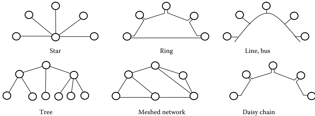
FIGURE 20.12 Topological network structures typically used in fieldbus systems.
