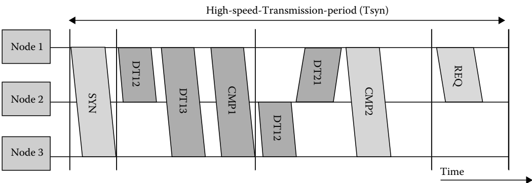
FIGURE 21.3 TCnet timing.
