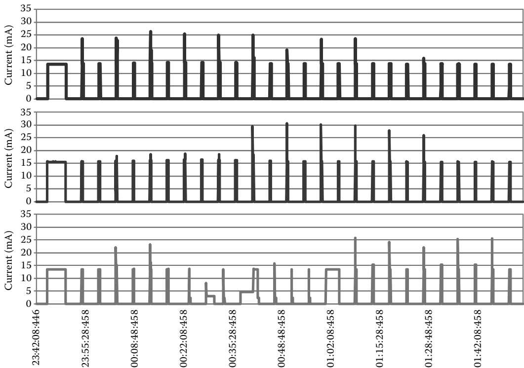
FIGURE 11.16 Current consumption of three independent nodes running a TDM protocol. The bottom node can be seen losing sync and re synchronizing after a number of iterations.
