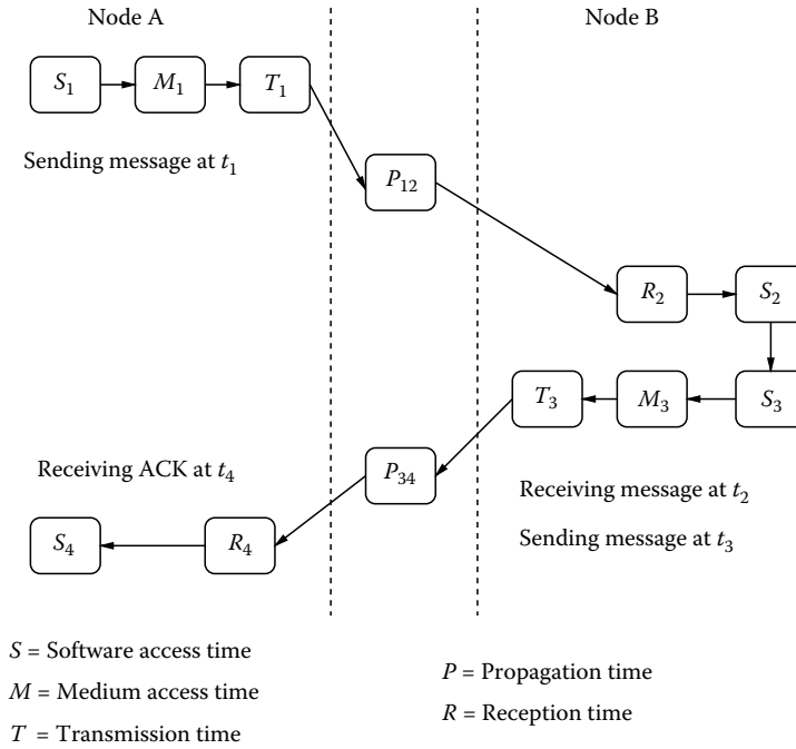
FIGURE 5.2 Round-trip time.
