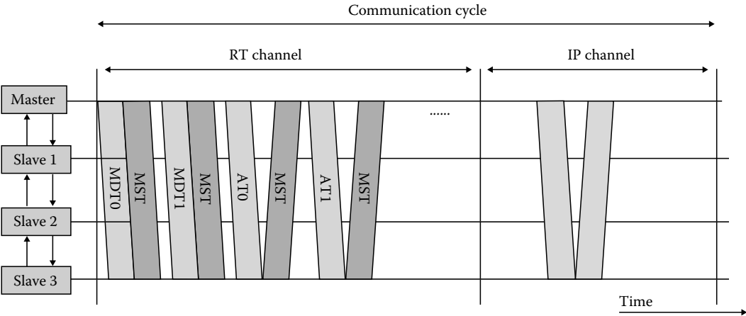
FIGURE 21.5 SERCOS timing.
