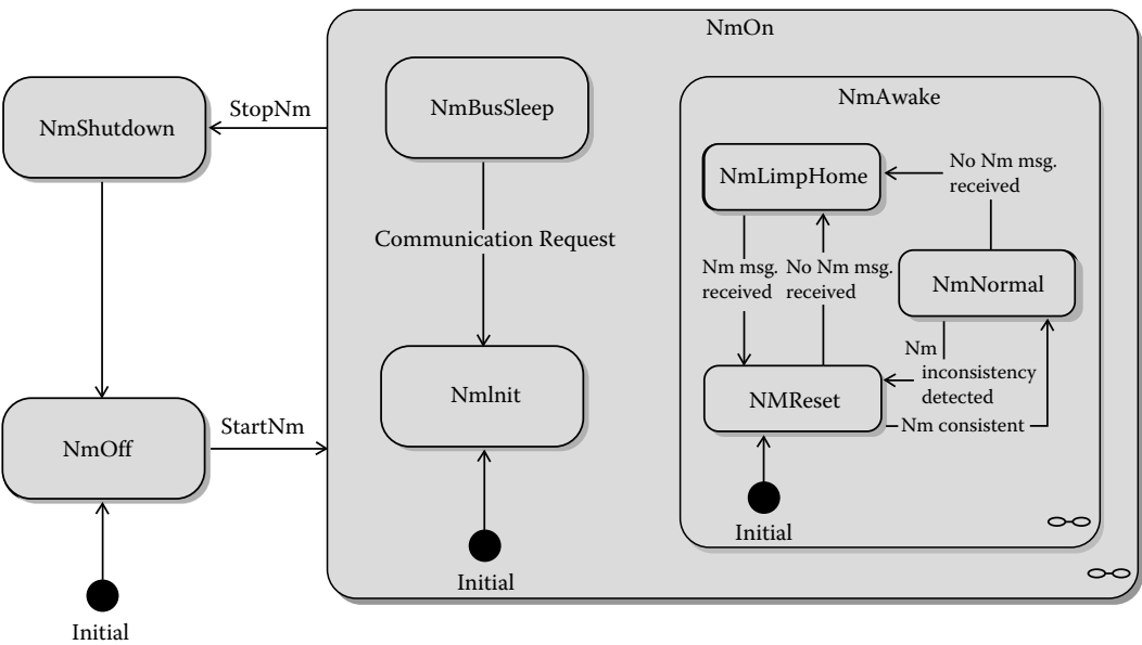
FIGURE 18.4 OSEK NM state automaton.
