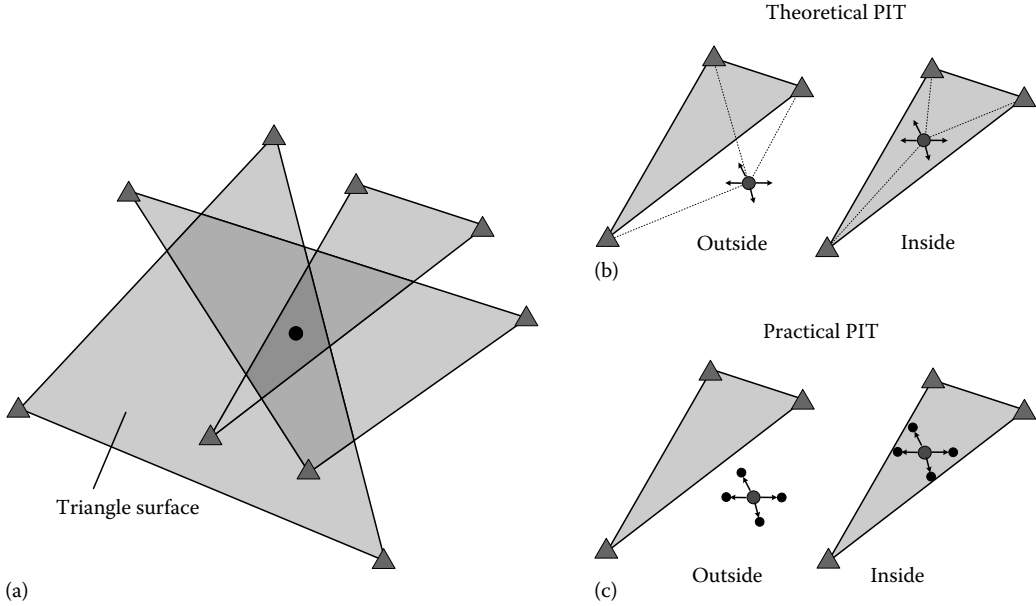
FIGURE 6.18 (a) Overlapping of triangles are basis of APIT, (b) theoretical PIT test with distances and a moveable sensor node, and (c) practical PIT test with neighbors and RSSI values. (From Reichenbach, F., Born, A., Bill, R., and Timmermann, D., Lokalisierung in Ad Hoc Geosensornetzwerken mittels geodatischer Ausgleichungstechnik, GIS: Zeitschrift für Geo Informationssysteme , ABC Verlag GmbH, Heidelberg, Germany, 2008, pp. 4–16. With permission; Reichenbach, F., Resource aware algorithms for exact localization in wireless sensor networks , PhD thesis, University of Rostock, Rostock, Germany, December 2007. With permission.)
