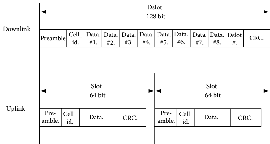
FIGURE 28.4 WISA slot format: downlink double slot duration = 128 \mu s, uplink slot duration = 64 \mu s. Double slots may be used on the uplink for higher payload data profiles. (From Scheible, G., Dzung, D., Endresen, J., and Frey, J.-E., IEEE Ind. Electron. Mag. , 1, 25, 2007. With permission.)
