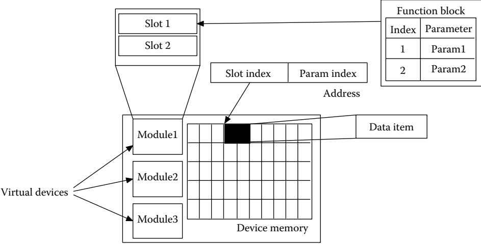
FIGURE 22.6 Mapping of function blocks to physical device in PROFIBUS DP. (From Pitzek, S. and Elmenreich, W., Configuration and management of fieldbus systems. In R. Zurawski, ed., The Industrial Communication Technology Handbook . CRC Press, Boca Raton, 2005. With permission.)
