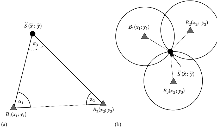
FIGURE 6.14 Localization with (a) angulation and (b) lateralation. (From Reichenbach, F., Resource aware algorithms for exact localization in wireless sensor networks, PhD thesis, University of Rostock, Rostock, Germany, December 2007. With permission.)
