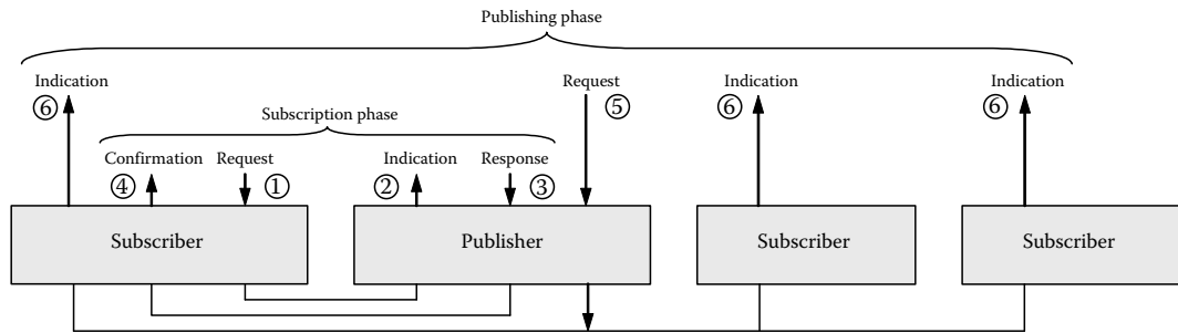
FIGURE 20.23 Push-type publisher-subscriber model.
