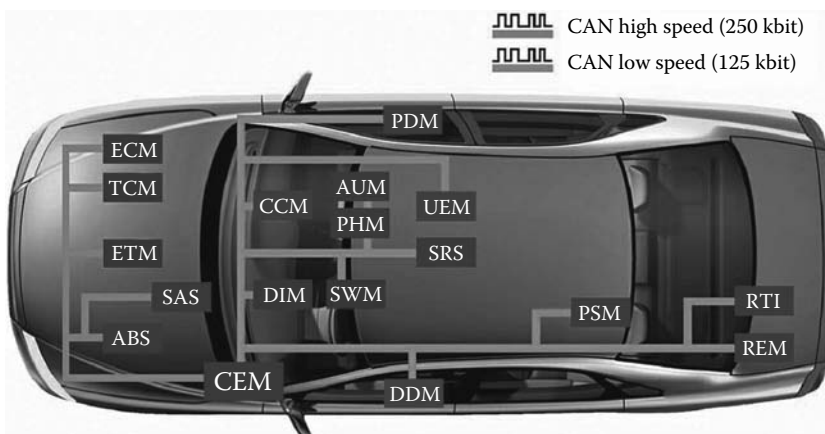
FIGURE 19.1 Volvo S80 main networks.
