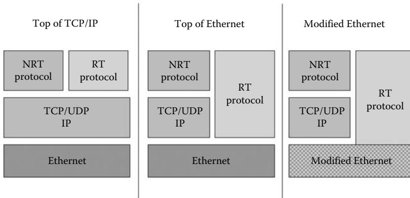
FIGURE 21.1 Possible structures for RTE.
