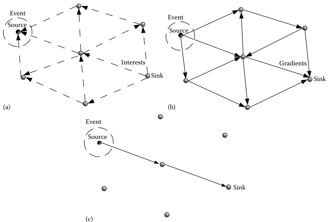
FIGURE 7.2 Directed Diffusion protocol operations. (a) Interest propagation. (b) Initial gradients setup. (c) Data delivery along reinforced path. (Redrawn from Intanagonwiwat, C., Govindan, R., and Estrin, D., Directed diffusion: A scalable and robust communication paradigm for sensor networks, in Proceedings of the 6th Annual ACM/IEEE International Conference on Mobile Computing and Networking , pp. 56–67, 2000.)
