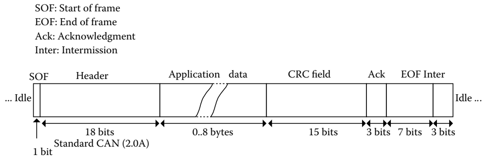
FIGURE 13.1 Format of the CAN 2.0A data frame. (From Navet, N., Song, Y.Q., Simonot-Lion, F., and Wilwert, C., Proc. IEEE , 93(6), 1204, 2005. With permission.)
