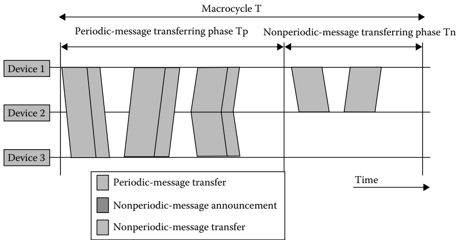
FIGURE 21.4 EPA timing.
