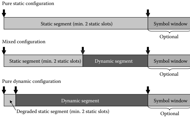
FIGURE 16.5 FlexRay configurations.
