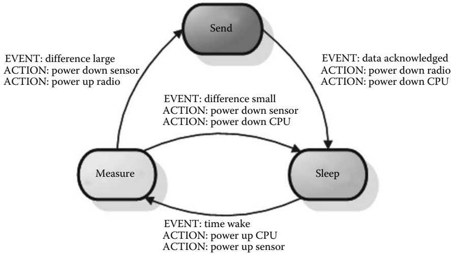
FIGURE 27.13 Sensor node state diagram. (From Aakvaag, N. and Frey, J.-E., ABB Rev. , 2, 2006. With permission.)
