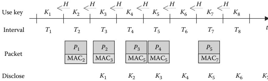
FIGURE 10.7 Example of TESLA operation.
