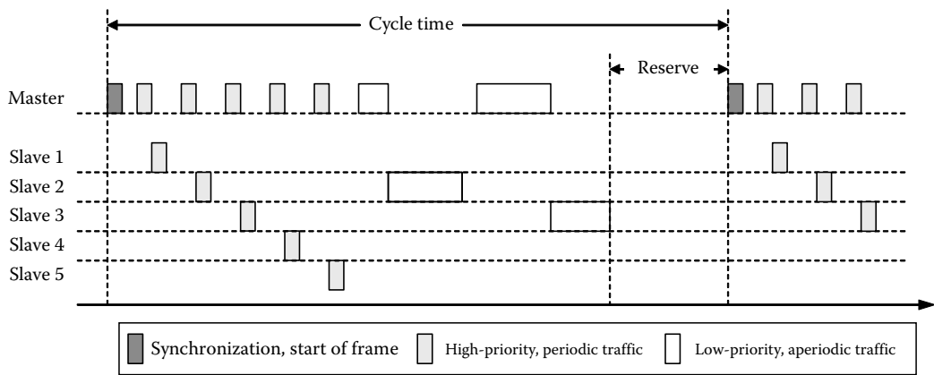
FIGURE 20.14 Bus cycle with cyclic polling and room for aperiodic traffic (PROFIBUS-DP V2).
