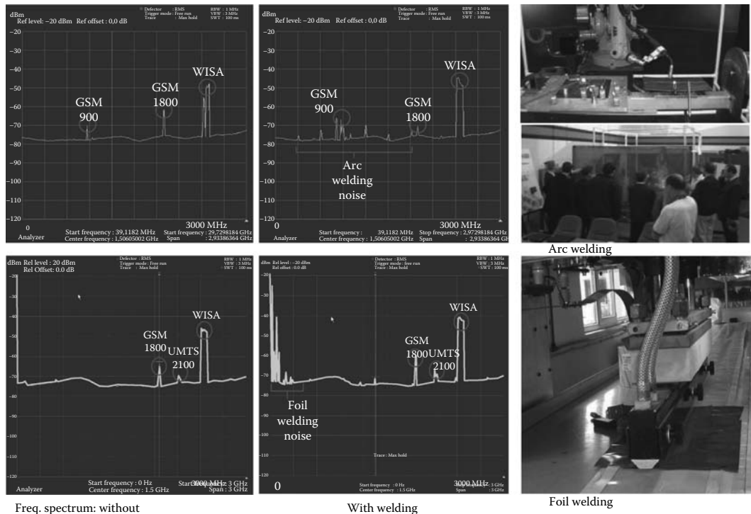
FIGURE 28.10 Frequency spectrum plots of electromagnetic noise of industrial welding equipment.
