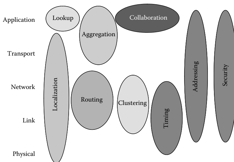
FIGURE 4.3 Relationship between building blocks/OSI layers.
