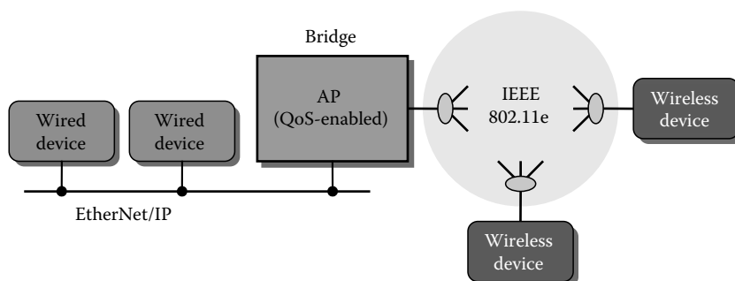
FIGURE 26.9 Extension of EtherNet/IP via an AP.
