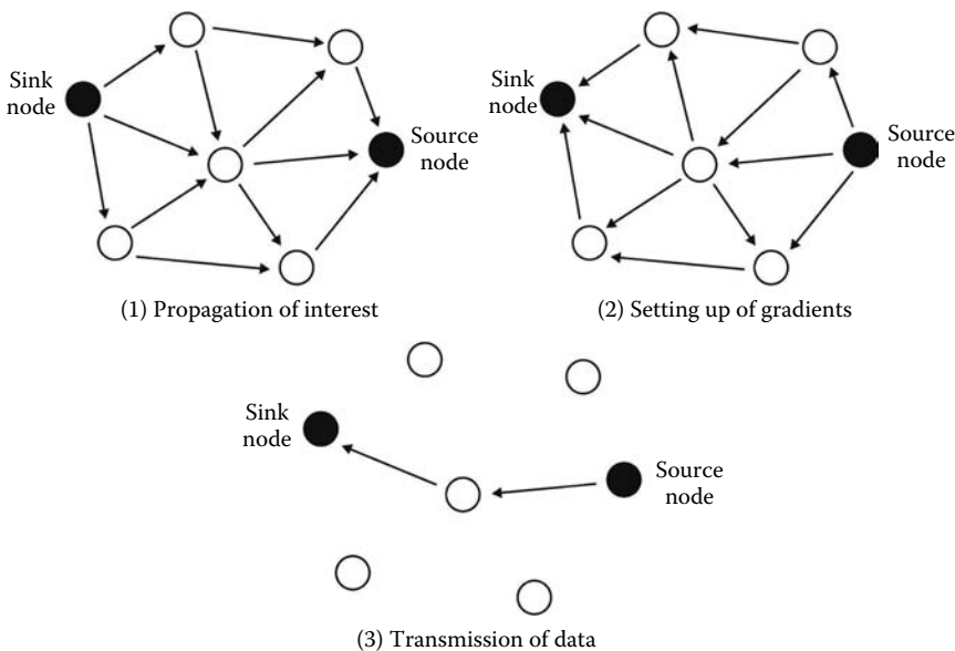
FIGURE 4.12 Setting up of gradients in directed diffusion.
