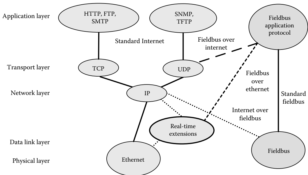
FIGURE 20.29 Structures of Ethernet and fieldbus combinations.
