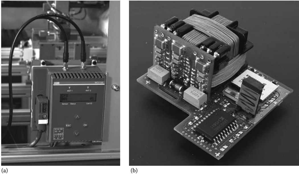
FIGURE 28.7 WISA implementation: (a) WISA base station with antenna connectors and field bus plug (FBP) connection to controller. (b) WISA sensor module with receiver coil for wireless power supply and communication transceiver, controller, and antenna. (From Scheible, G., Dzung, D., Endresen, J., and Frey, J.-E., IEEE Ind. Electron. Mag. , 1, 25, 2007. With permission.)
