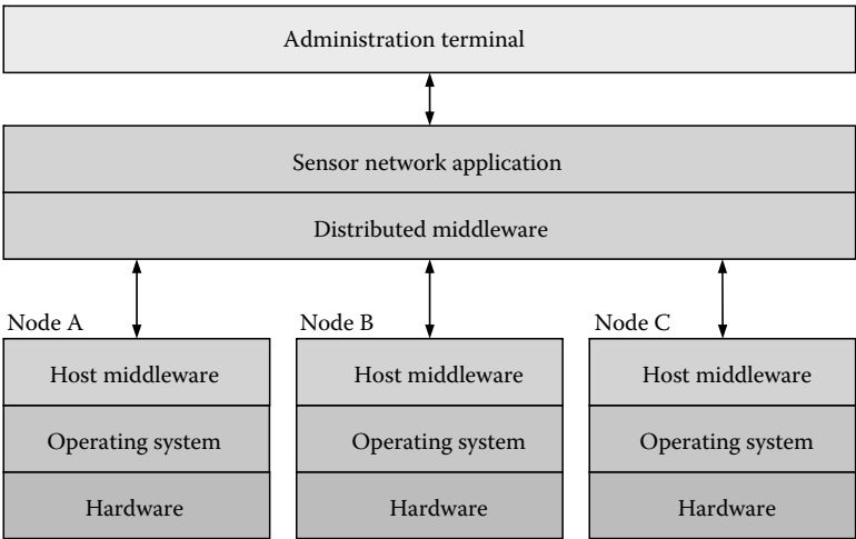
FIGURE 12.13 Structure of a sensor network.
