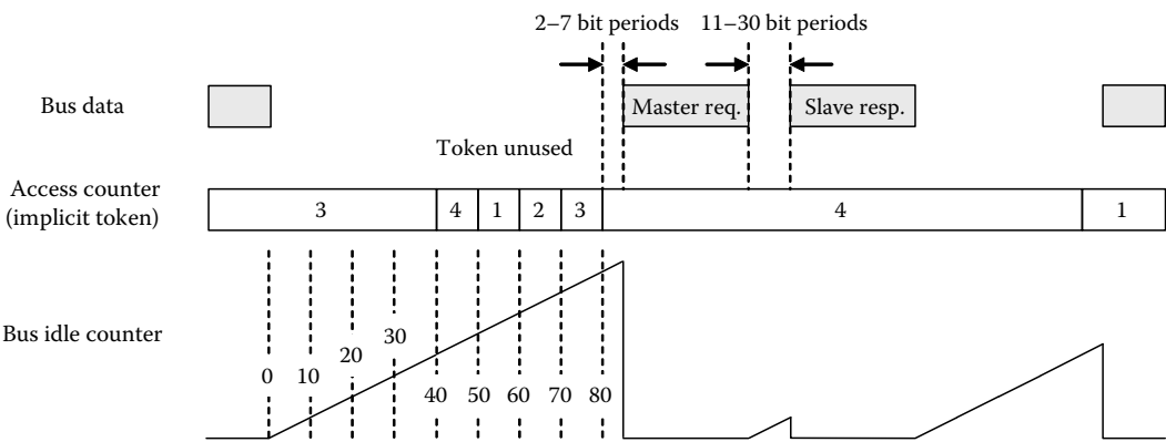
FIGURE 20.17 P-NET token passing and polling mechanism.
