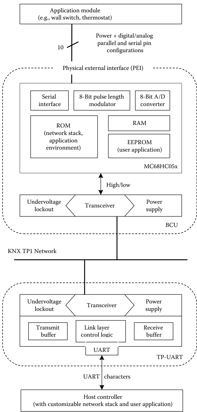
FIGURE 29.7 Typical KNX/EIB node architectures.
