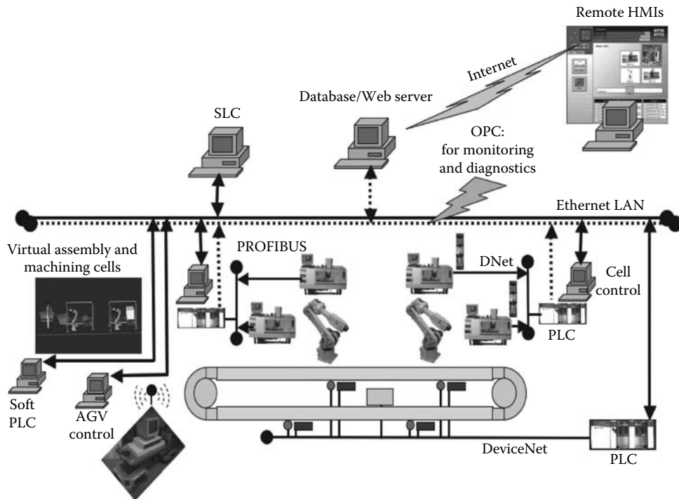
FIGURE 23.18 Networks on the RFT: control networks are indicated by solid lines and diagnostics networks are indicated by dashed lines.
