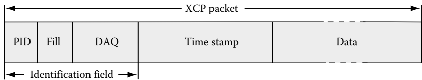
FIGURE 18.10 Structure of an XCP packet.
