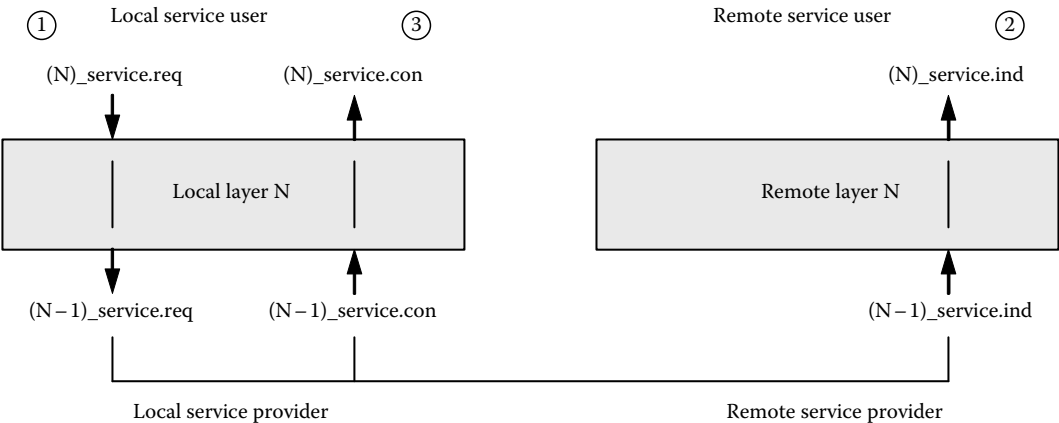
FIGURE 20.6 Locally confirmed service.
