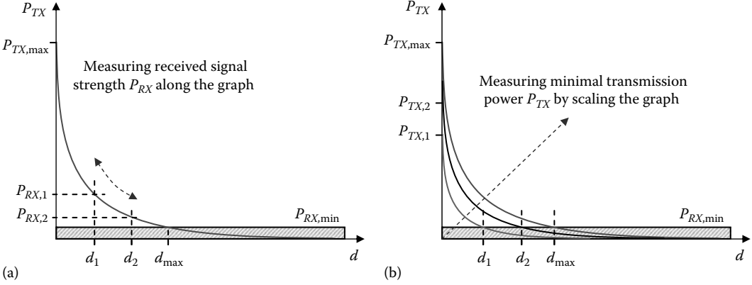
FIGURE 6.10 Distance estimation between sender and receiver with (a) RSS and (b) MTP.
