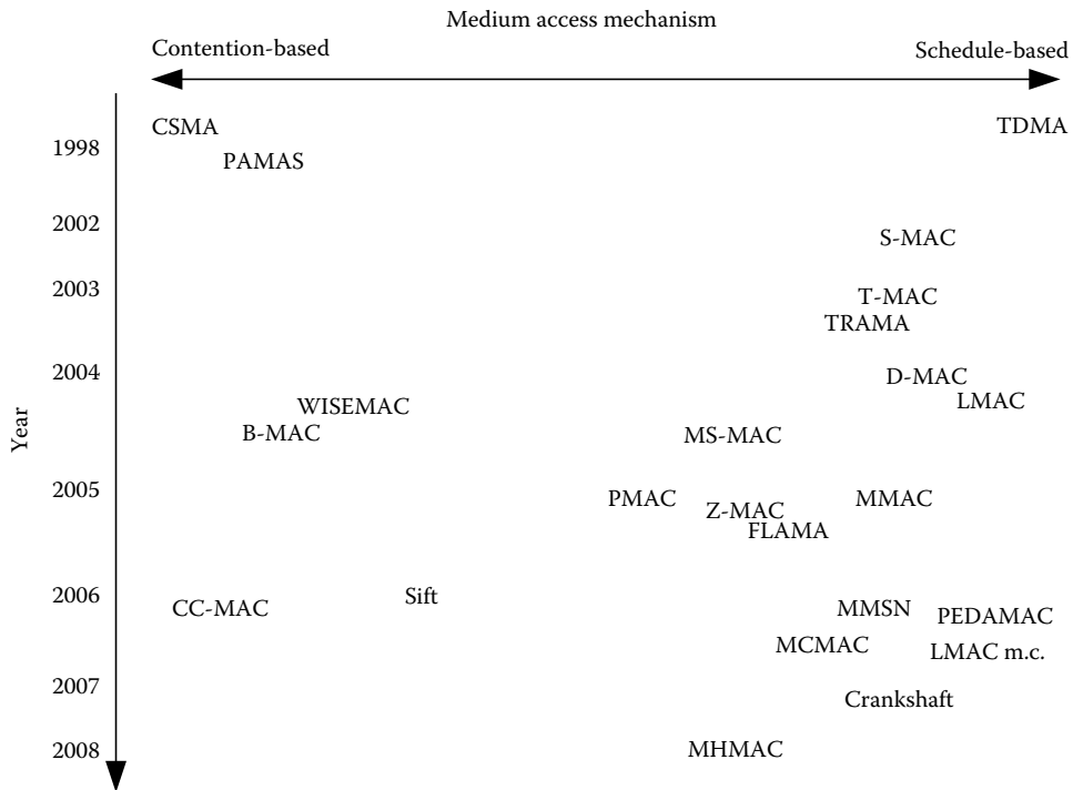
FIGURE 8.1 Classification of MAC protocols for WSNs.
