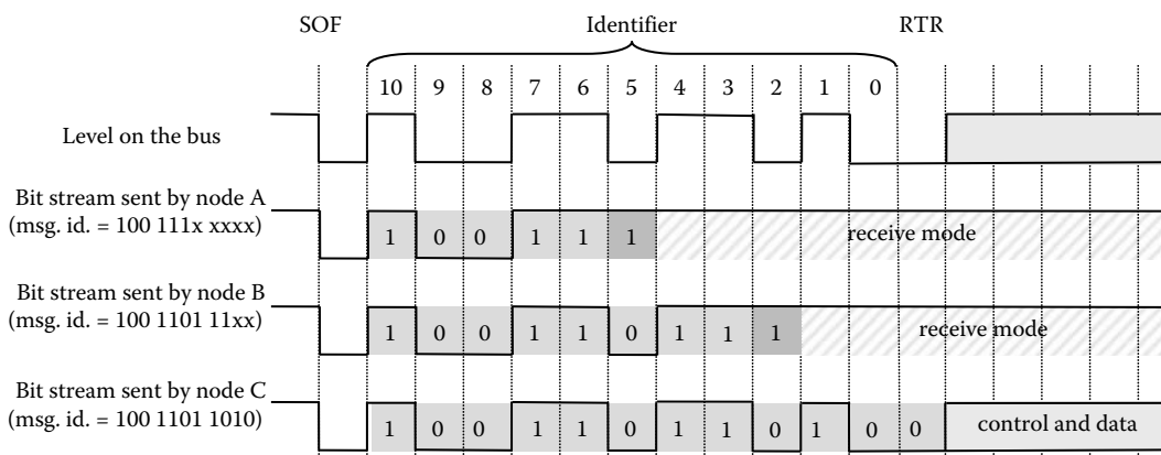
FIGURE 15.4 Arbitration phase in CAN.
