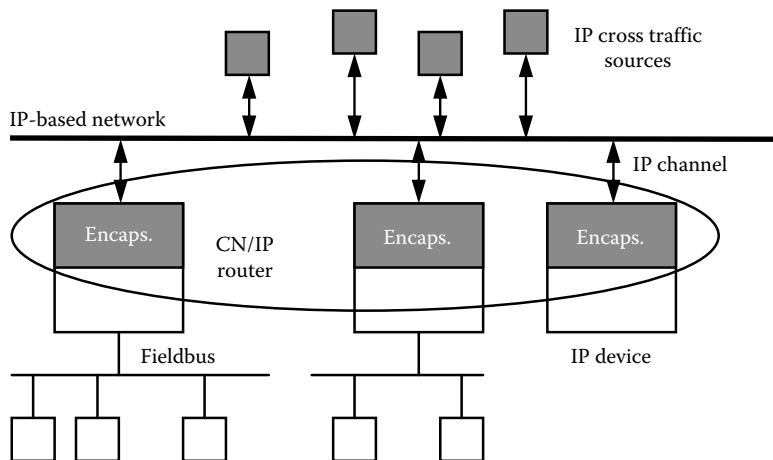
FIGURE 20.27 Structure of an IP channel for fieldbus data tunneling over the Internet.
