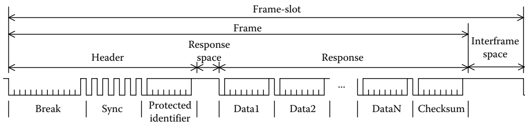
FIGURE 13.7 Format of the LIN frame. A frame is transmitted during its frame-slot, which corresponds to an entry of the schedule table. (From Navet, N., Song, Y.Q., Simonot-Lion, F., and Wilwert, C., Proc. IEEE , 93(6), 1204, 2005. With permission.)
