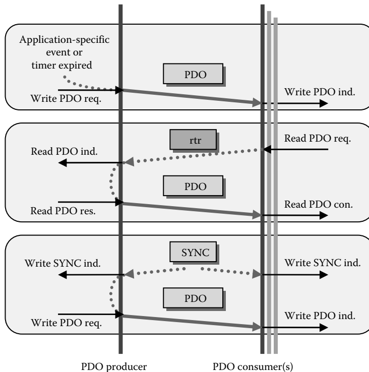
FIGURE 15.12 Transmission modes.
