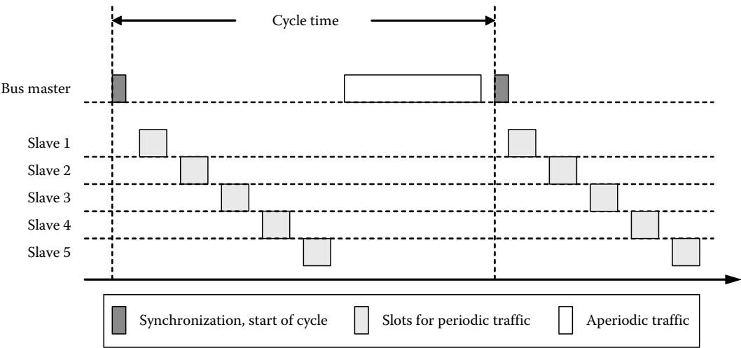
FIGURE 20.18 Centralized TDMA scheme (e.g., SERCOS).
