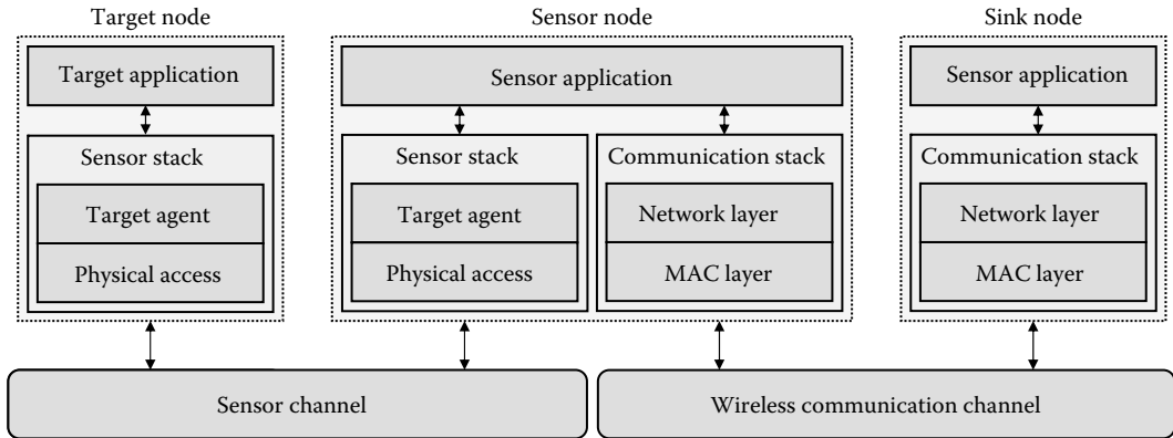
FIGURE 12.27 Model of a sensor network using SensorSim in J-Sim.
