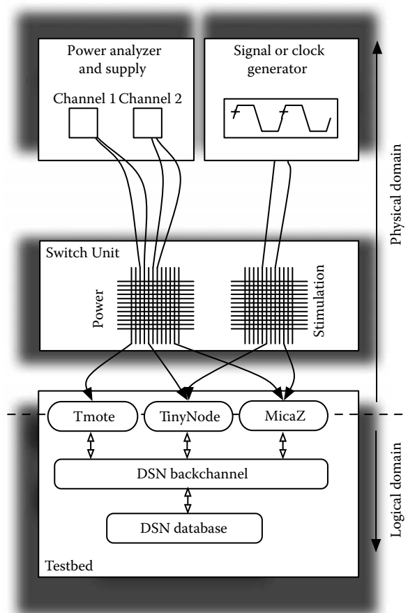
FIGURE 11.11 Logical and physical domain of the test architecture control apparatus used.
