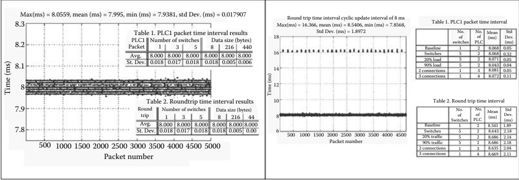
FIGURE 23.10 Sample plots of round-trip timing measurements for PROFINET (5a) and EtherNet/IP (5b). Here, the round-trip times for packets between two PLCs are plotted for a large number of packets to obtain a time distribution. The embedded tables represent the consolidation of a number of these graphs, where the testing environment is modified in terms of switches between sender and receiver, data size transmitted, and network loading (the plots shown represent the “Baseline” case).
