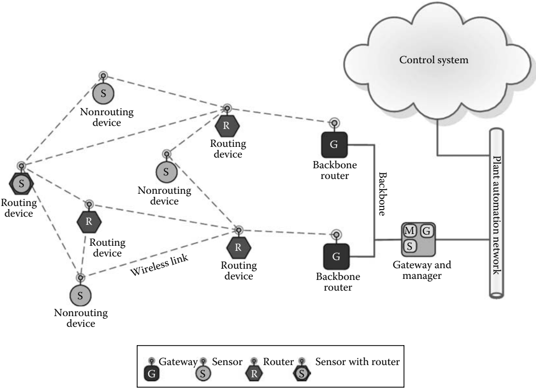
FIGURE 27.11 ISA100.11a network.
