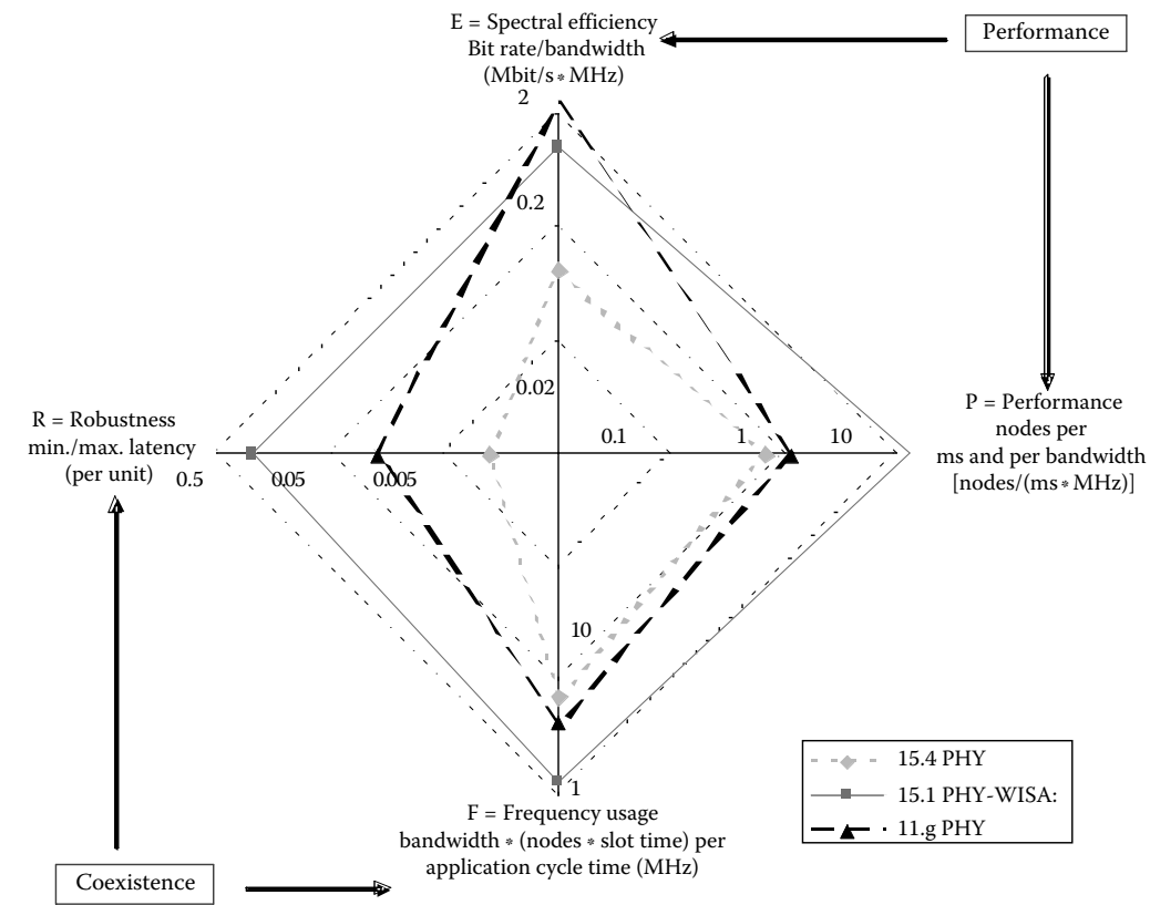
FIGURE 28.17 Characteristic figures for coexistence and performance according to Table 28.5.
