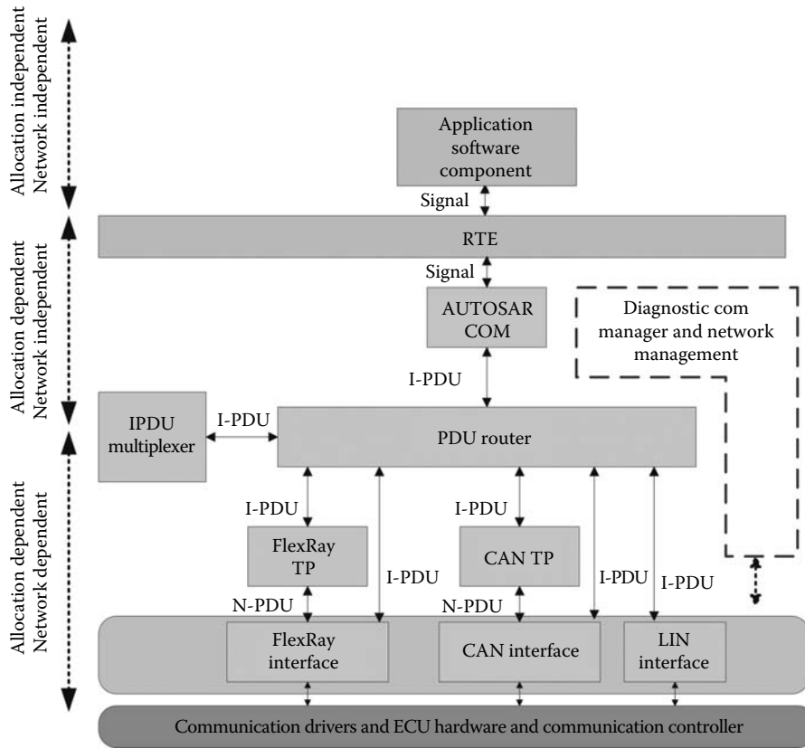
FIGURE 13.9 Communication software components and architecture.
