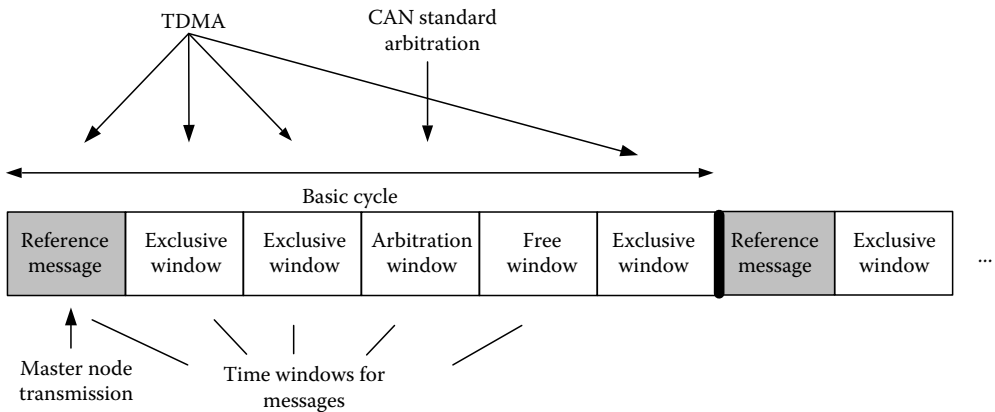
FIGURE 13.6 Example of a TTCAN basic cycle. (From Navet, N., Song, Y.Q., Simonot-Lion, F., and Wilwert, C., Proc. IEEE , 93(6), 1204, 2005. With permission.)
