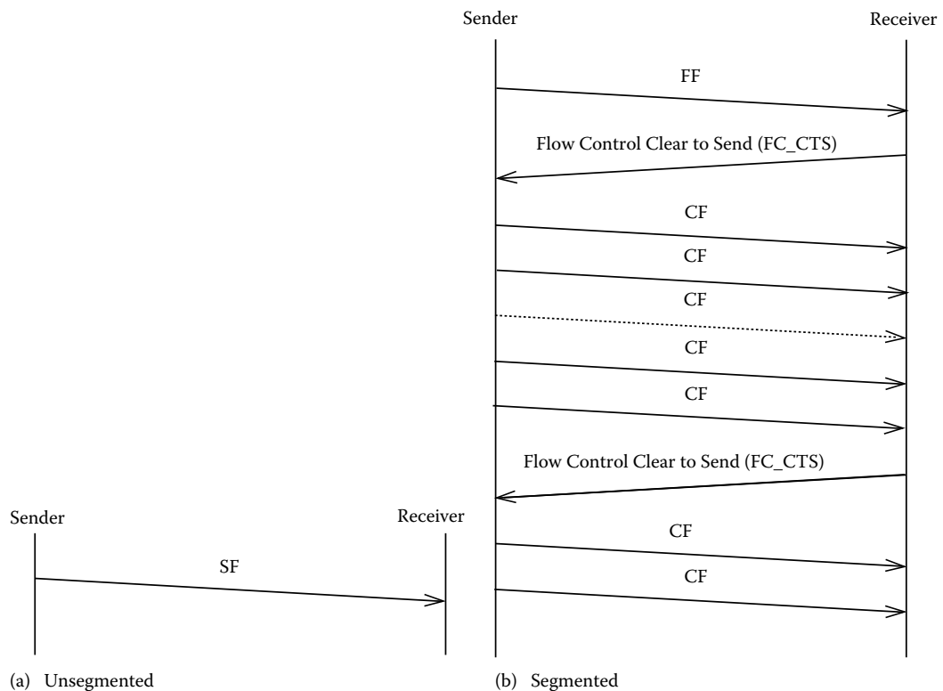
FIGURE 18.7 ISO transport layer—transmission sequence.
