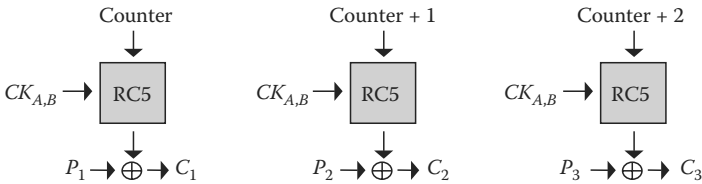
FIGURE 10.5 Encryption in counter mode.
