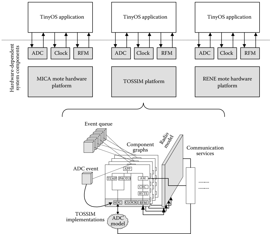
FIGURE 12.20 Comparison of TinyOS and TOSSIM system architecture.
