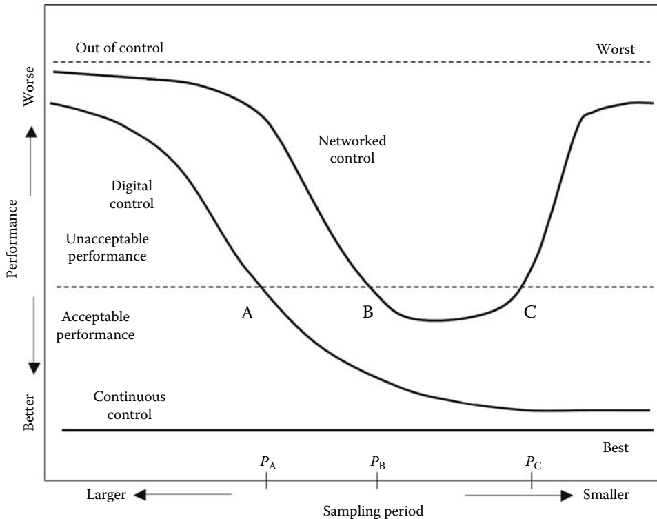
FIGURE 23.6 Performance comparison of continuous control, digital control, and networked control, as a function of sampling frequency.
