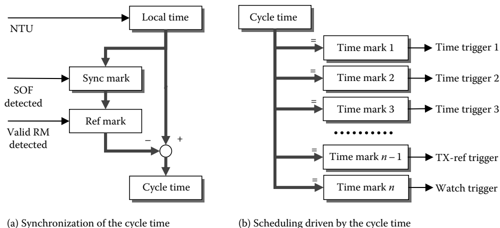
FIGURE 15.9 Time-triggered operation in TTCAN.
