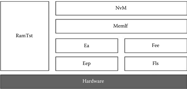
FIGURE 18.15 AUTOSAR—memory substack.
