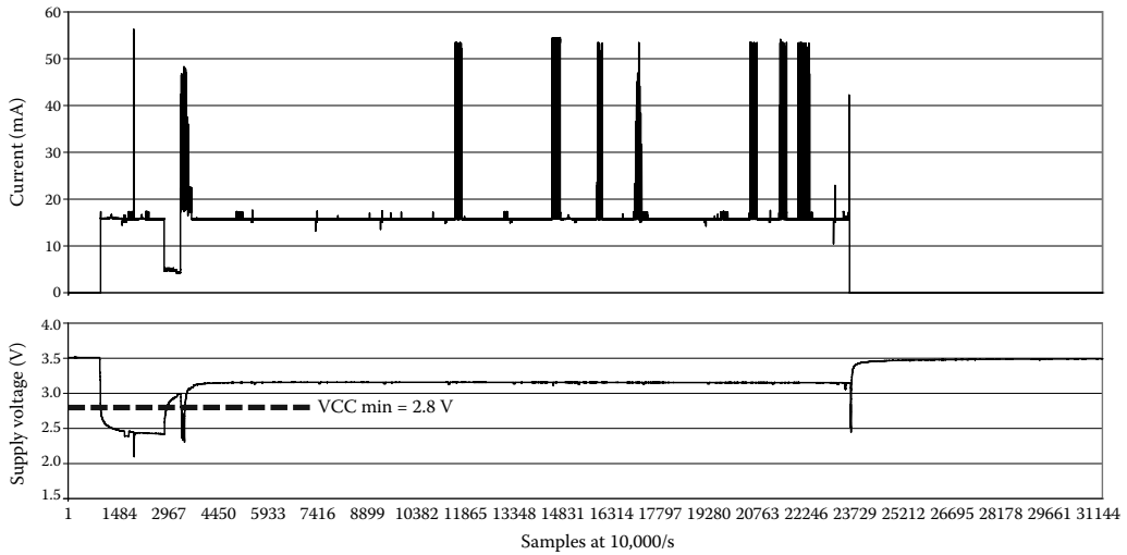
FIGURE 11.15 Current trace for one communication round at 10,000 samples/s.
