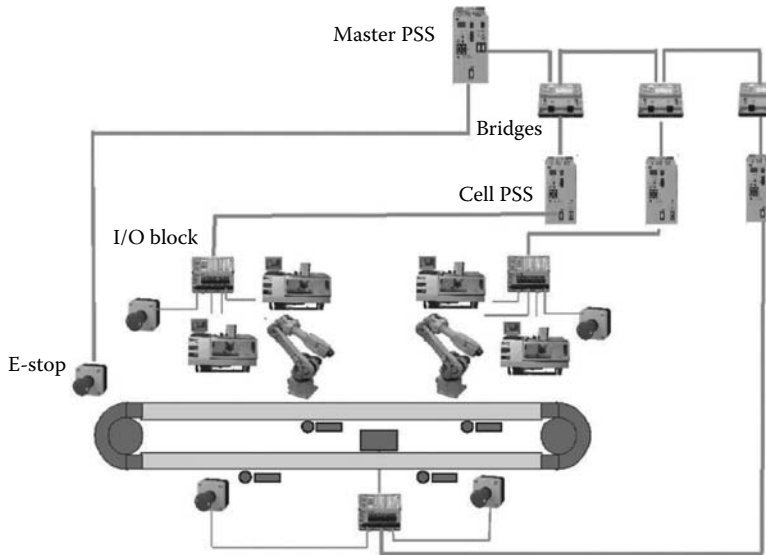
FIGURE 23.19 Safety network implementation on the RFT.
