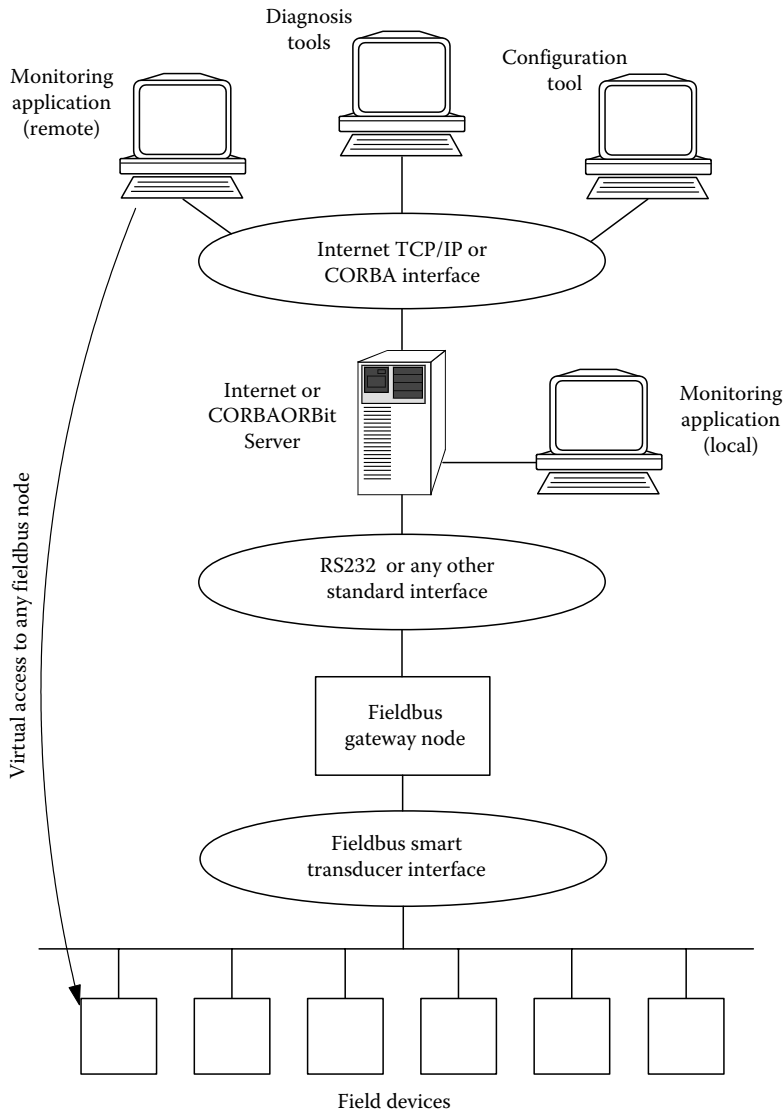
FIGURE 22.1 Architecture for remote configuration and monitoring. (From Pitzek, S. and Elmenreich, W., Configuration and management of fieldbus systems. In R. Zurawski, ed., The Industrial Communication Technology Handbook . CRC Press, Boca Raton, 2005. With permission.)
