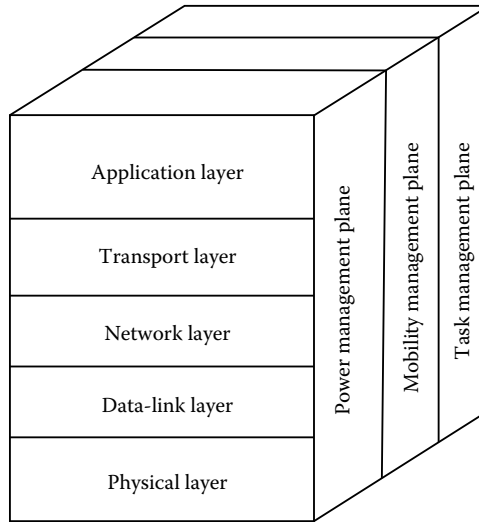
FIGURE 4.4 Protocol stack representation of the architecture. (From Akyildiz, I., Su, W., Sankarasubramaniam, Y., and Cayirci, E., IEEE Commun. Mag. , 40, 102, 2002.)
