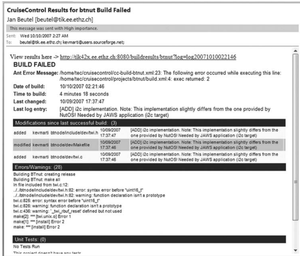
FIGURE 11.7 Build results and error messages are directly reported using email notification.
