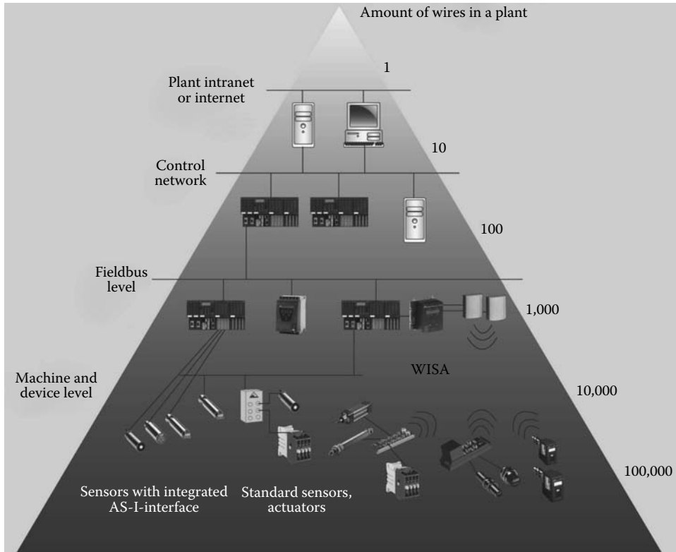
FIGURE 28.1 Automation hierarchy in factory automation, communication levels, and number of possible nodes to be connected wirelessly.
