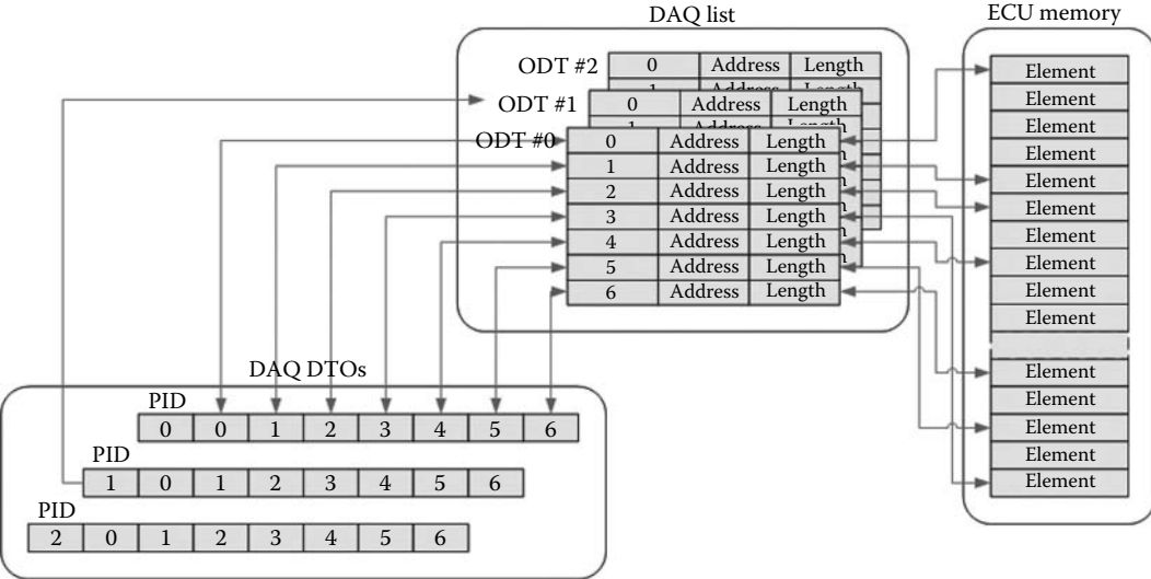
FIGURE 18.11 Structure of a DAQ list.
