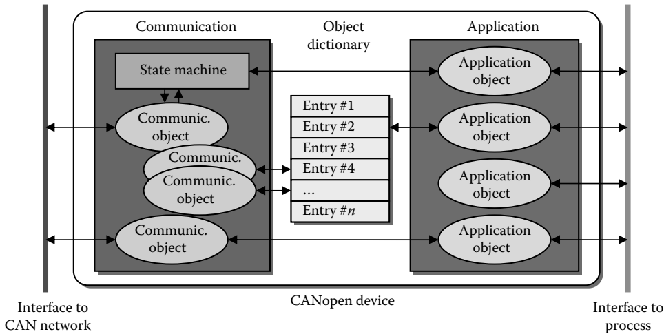
FIGURE 15.10 Conceptual internal architecture of CANOpen devices.
