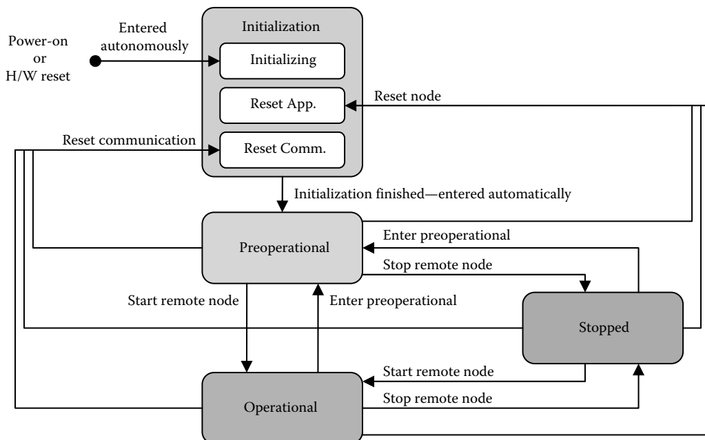
FIGURE 15.13 NMT state machine.
