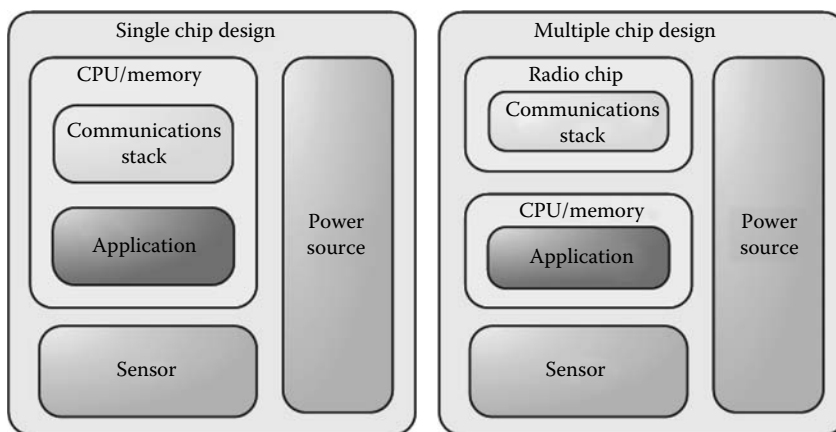
FIGURE 27.16 Example of single vs. multi-chip solution.
