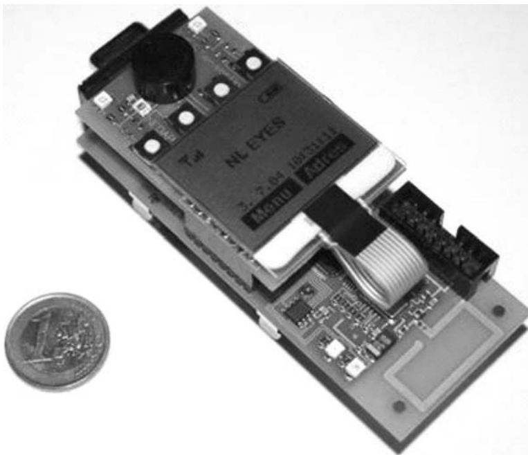
FIGURE 4.1 EYES sensor node. (From Consortium: EYES European project. http://eyes.eu.org , 2006.)
