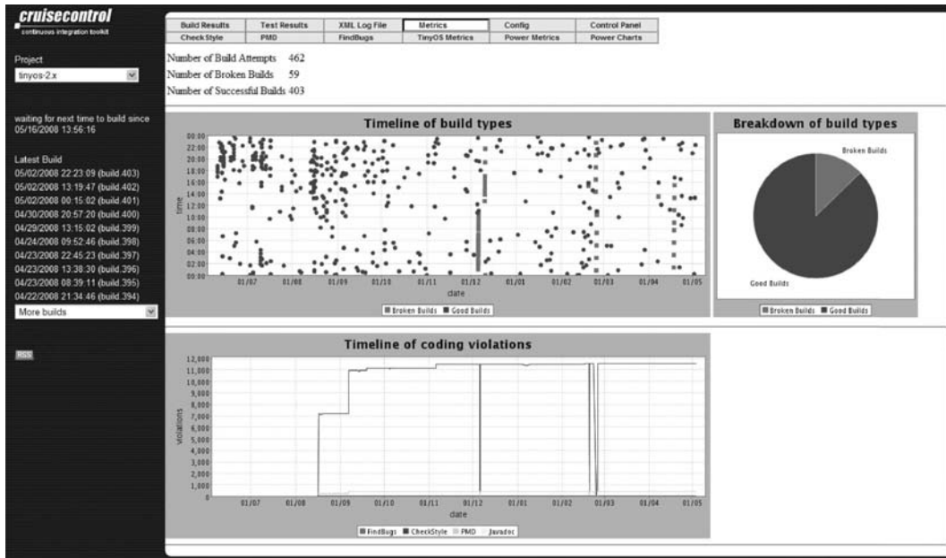
FIGURE 11.6 Build result status, histogram, and statistics are reported on the CruiseControl Webpage.
