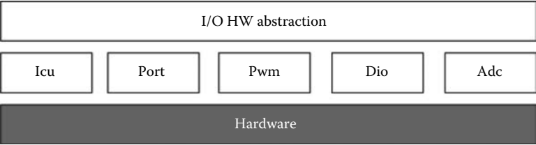
FIGURE 18.16 AUTOSAR—I/O substack.
