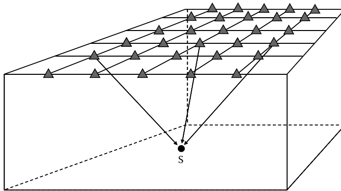
FIGURE 6.12 Schematic of the Active Bat system. (From Blumenthal, J., Resource aware and decentral localization of autonomous sensor nodes in sensor networks, PhD thesis, University of Rostock, Rostock, Germany, 2007, submitted. With permission.)
