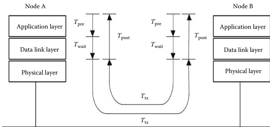
FIGURE 23.1 Timing diagram showing time spent sending a message from a source node to a destination node.
