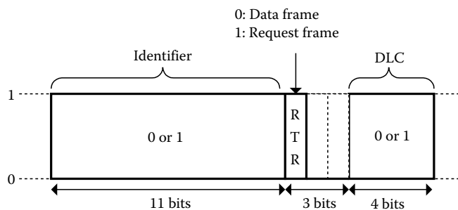
FIGURE 13.2 Format of the header field of the CAN 2.0A data frame. (From Navet, N., Song, Y.Q., Simonot-Lion, F., and Wilwert, C., Proc. IEEE , 93(6), 1204, 2005. With permission.)
