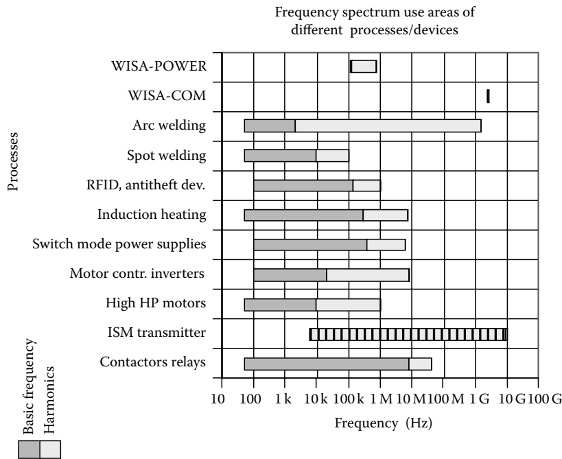
FIGURE 28.9 Electromagnetic interference from typical applications in industry.
