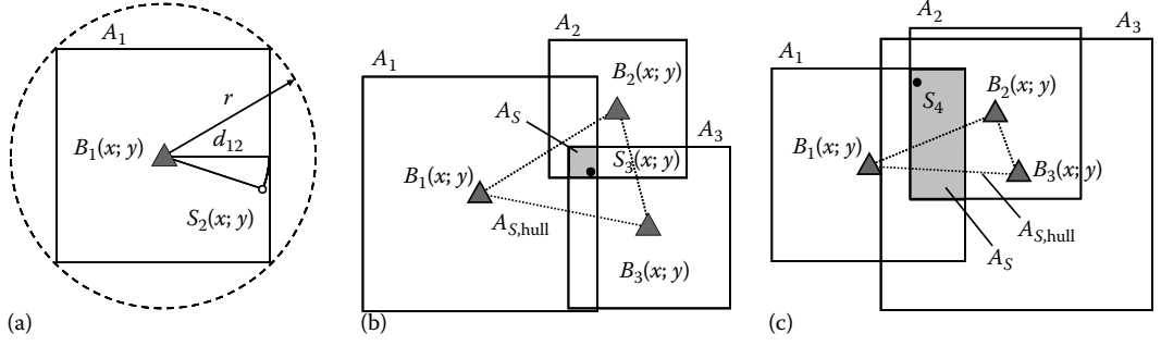
FIGURE 6.19 (a) Bounding box of B_1(x_1; y_1) , (b) bounding box A_S of sensor node S_3(x_3; y_3) ( S_3 \in A_{S,hull} ), and (c) bounding box A_S ( S_4 \notin A_{S,hull} ). (From Blumenthal, J., Resource aware and decentral localization of autonomous sensor nodes in sensor networks, PhD thesis, University of Rostock, Rostock, Germany, 2007, submitted. With permission.)
