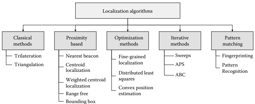
FIGURE 6.13 Classification of localization algorithms.
