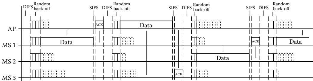
FIGURE 25.4 Principle time behavior of IEEE 802.11 under the distributed coordination function; note that the random back-off timer from units not transmitted next continues after the next DIFS with the remaining number of slots. (From Matheus, K. Industrial Information Technology Handbook . Ed. R. Zurawski, CRC Press, Boca Raton, FL, 2004. With permission.)
