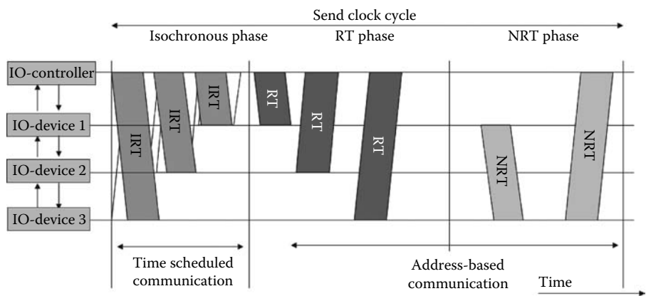
FIGURE 21.7 PROFINET timing.
