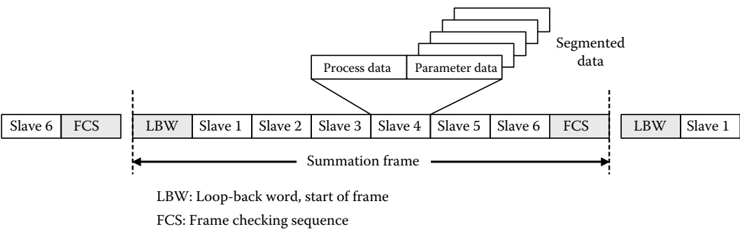
FIGURE 20.19 Summation frame of INTERBUS.
