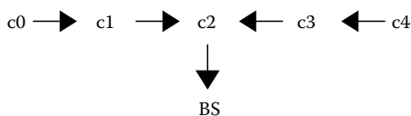
FIGURE 7.6 Chain-based forwarding in PEGASIS.
