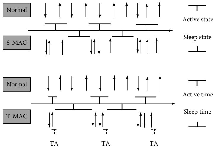
FIGURE 8.3 Duty cycles comparison between S-MAC and T-MAC. The arrows represent message transmissions and receptions.
