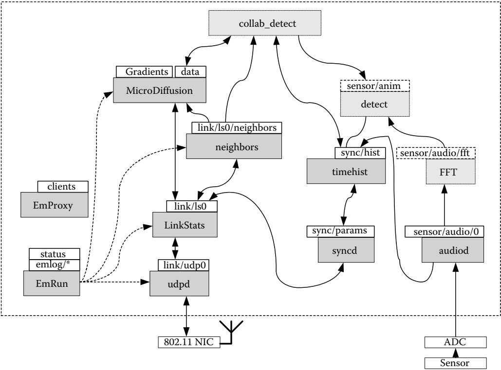
FIGURE 12.21 EmStar sample application consisting of EmStar core modules (dark-gray) and hypothetical application-specific modules (light-gray).
