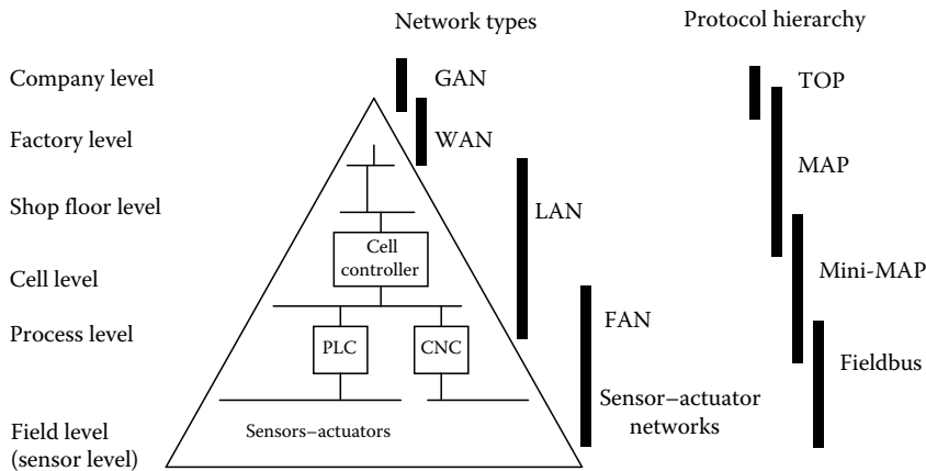
FIGURE 20.1 Hierarchical network levels in automation and protocols originally devised for them. (From Sauter, T., in The Industrial Communication Handbook , CRC Press, Boca Raton, FL, 2005, 71–739. With permission.)
