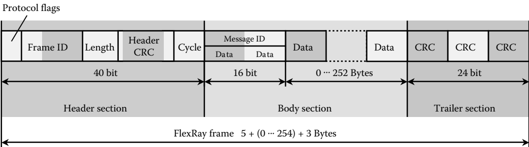
FIGURE 16.7 FlexRay frame format.
