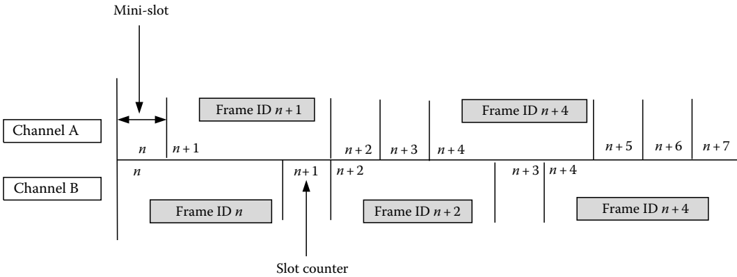
FIGURE 13.5 Example of message scheduling in the dynamic segment of the FlexRay communication cycle. (From Navet, N., Song, Y.Q., Simonot-Lion, F., and Wilwert, C., Proc. IEEE , 93(6), 1204, 2005. With permission.)
