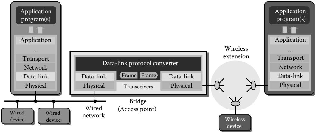
FIGURE 26.3 Interconnection of networks via a bridge.
