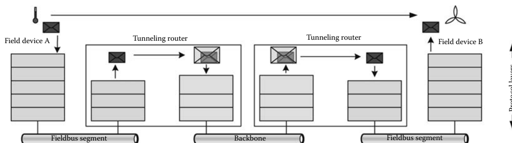
FIGURE 29.5 Tunneling router.
