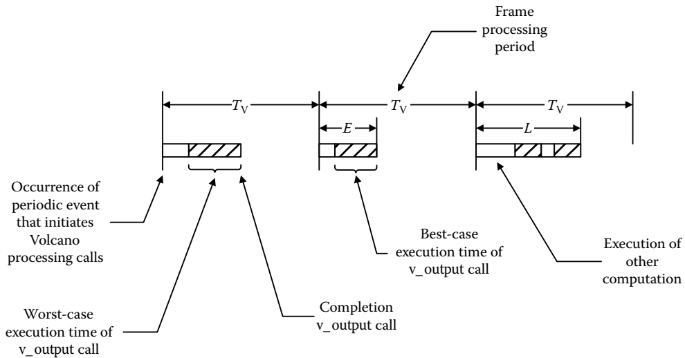
FIGURE 19.3 Output jitter.
