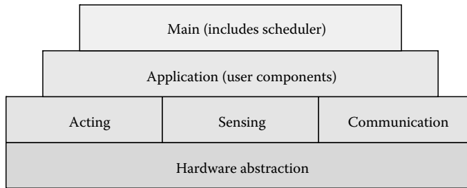
FIGURE 12.5 Software architecture of TinyOS.
