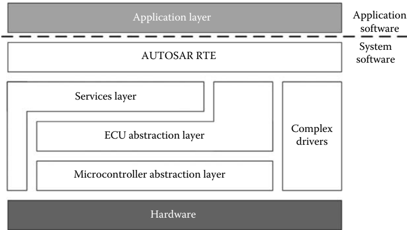
FIGURE 18.12 AUTOSAR—system software layered architecture.
