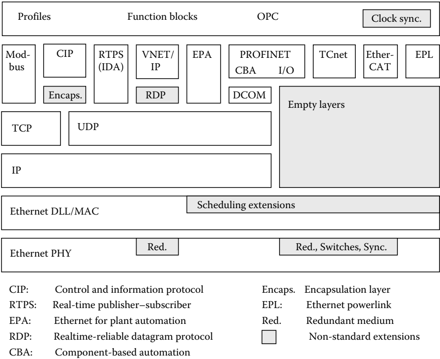
FIGURE 20.30 Protocol architecture of selected RTE solutions proposed for IEC 61784-2.
