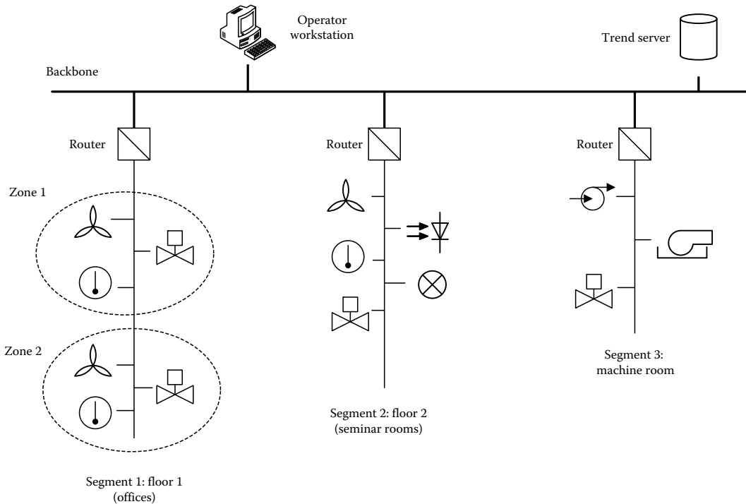
FIGURE 29.4 Automation network and backbone.
