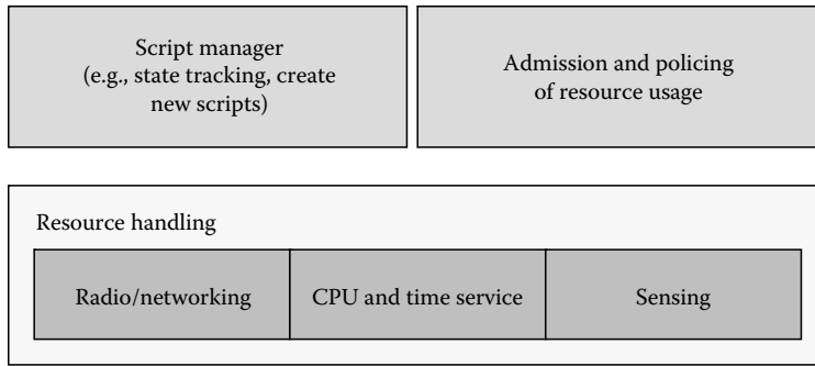
FIGURE 12.10 SensorWare runtime environment.
