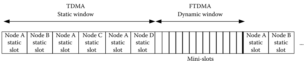
FIGURE 13.4 Example of a FlexRay communication cycle with 4 nodes A, B, C, and D. (From Navet, N., Song, Y.Q., Simonot-Lion, F., and Wilwert, C., Proc. IEEE , 93(6), 1204, 2005. With permission.)
