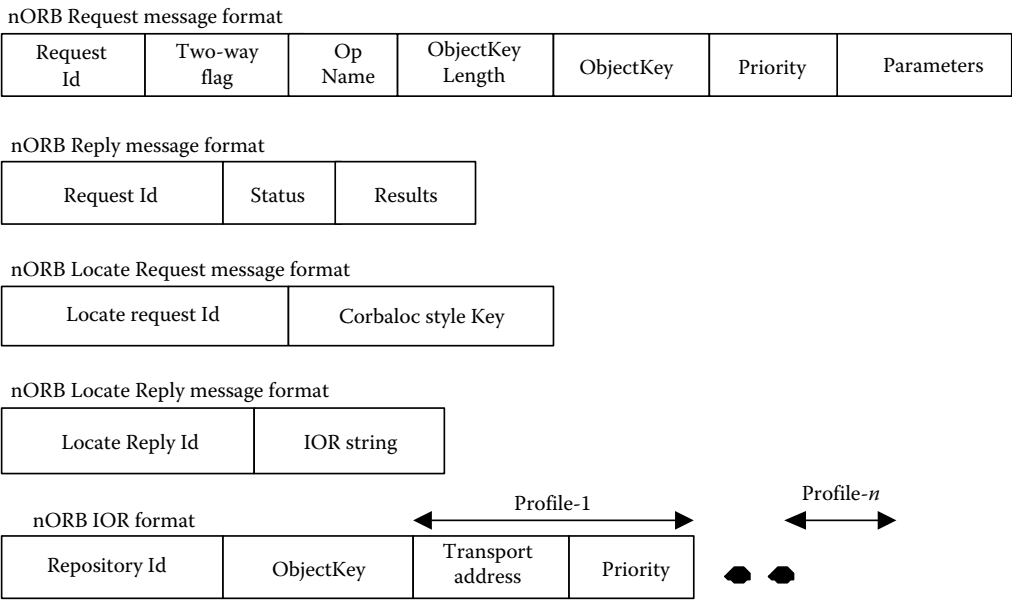
FIGURE 2.3 nORB IOR and message formats.
