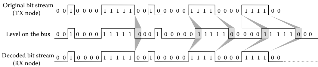
FIGURE 15.2 Bit stuffing technique.
