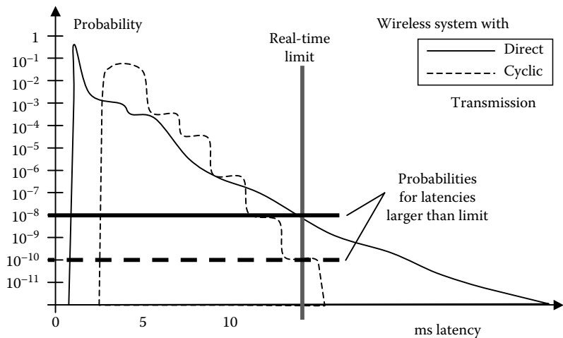
FIGURE 28.2 Typical distribution of latency measurements in wireless automation devices.
