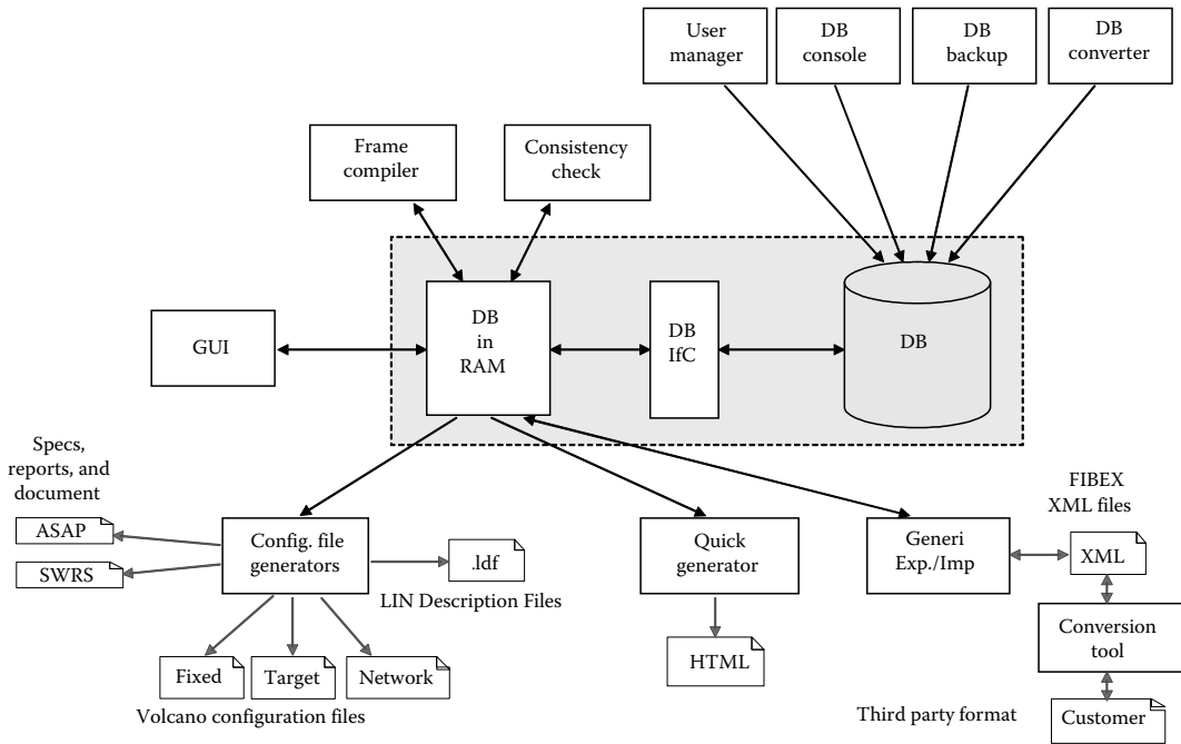
FIGURE 19.4 Structure of the VNA tool.
