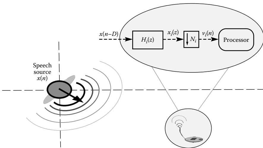
FIGURE 9.3 Relation between the signal v_i(n) produced by the front end of the i th sensor and the original source signal x(n) .
