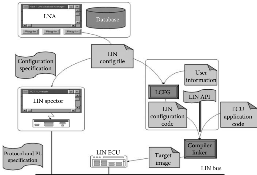
FIGURE 17.4 LIN configuration file (LDF) centric process flow.
