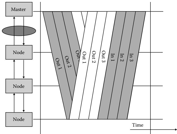
FIGURE 21.6 EtherCAT timing.
