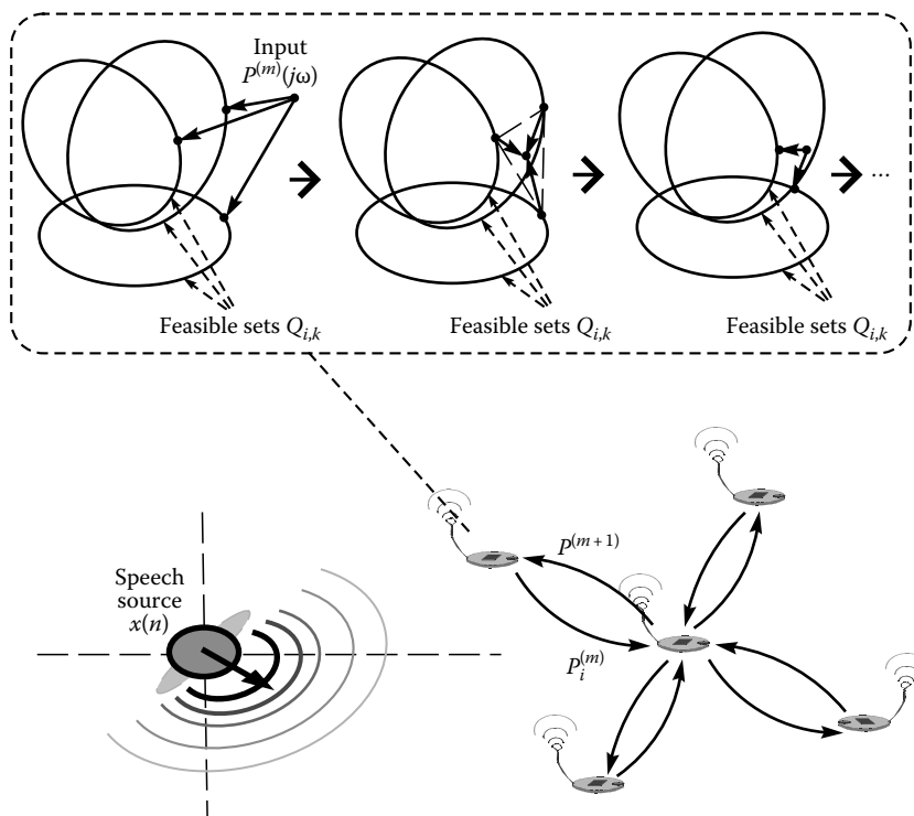
FIGURE 9.8 Star Algorithm. Again, only three feasible sets Q_{i,k} are shown in the inside picture. In practice, each sensor node has to repeat the sequence of projections and averaging many times before it can successfully project the input P^{(m)}(e^{j\omega}) supplied by the central node into the intersection of its feasible sets. The projection result, which is called P_i^{(m)}(e^{j\omega}) is sent back to the central node. The central node then averages all the P_i^{(m)}(e^{j\omega}) it has received and averages them to produce P^{(m+1)}(e^{j\omega}) . This is sent back to the individual nodes and the process repeats.
