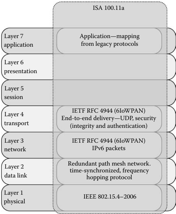
FIGURE 27.12 ISA100.11a protocol stack.
