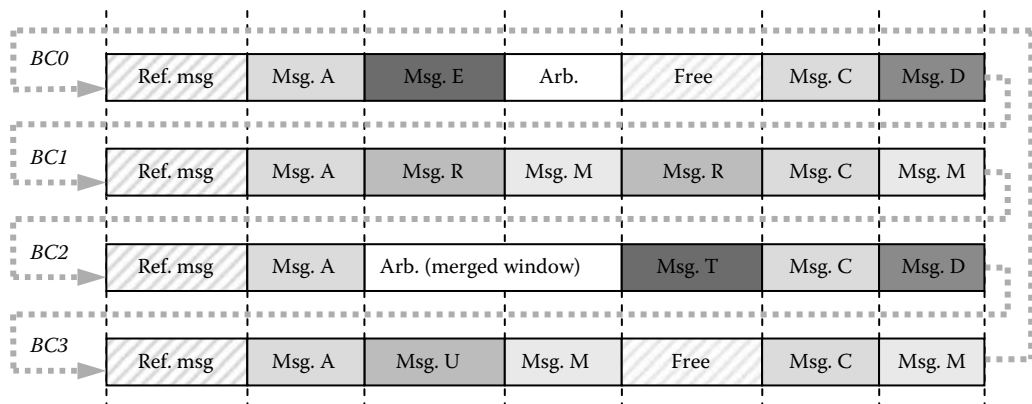
FIGURE 15.8 System matrix in TTCAN.
