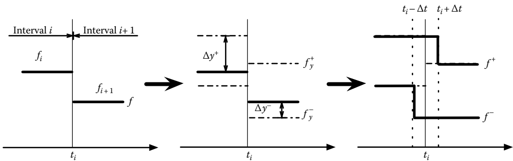
FIGURE 11.10 Illustration of bounds derivation of the acceptance region given a reference function.
