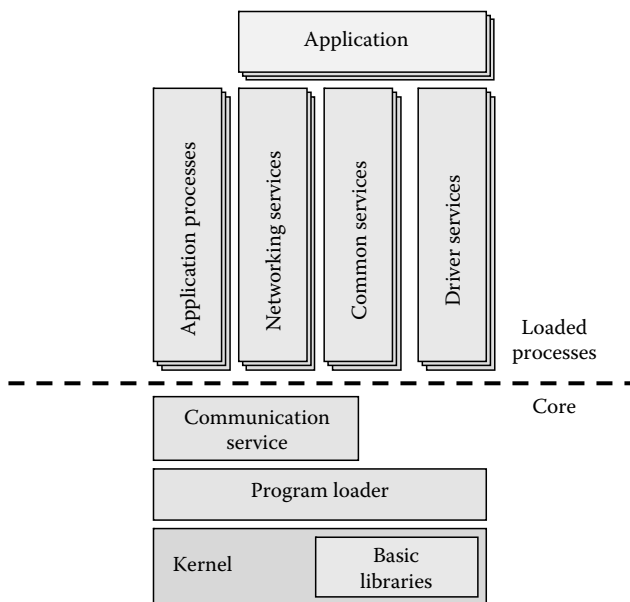
FIGURE 12.17 System architecture of Contiki.
