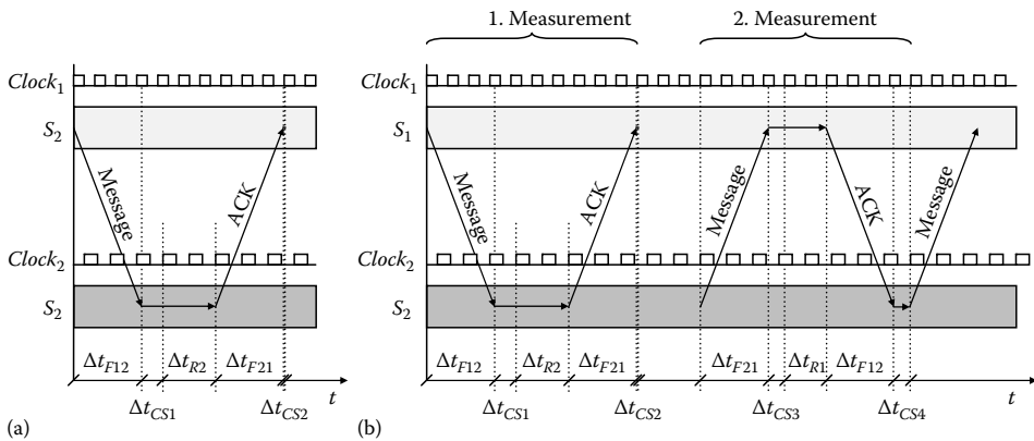
FIGURE 6.4 (a) Round trip time RTT and (b) symmetric double-sided two-way ranging SDS-TWR.
