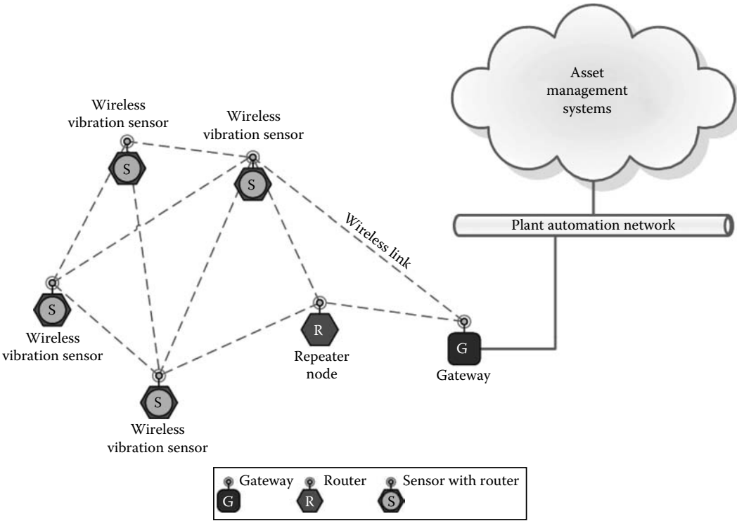
FIGURE 27.7 Wireless vibration monitoring system.
