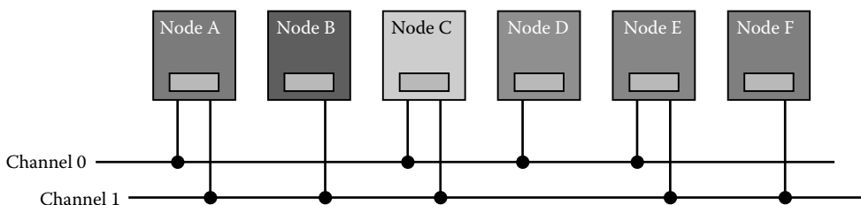
FIGURE 16.1 FlexRay network.
