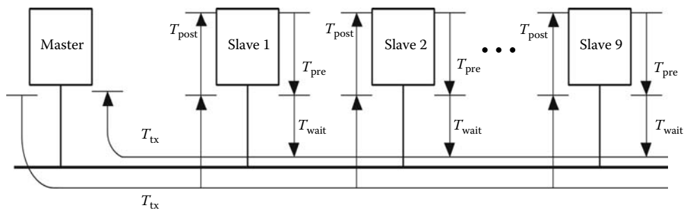
FIGURE 23.3 Waiting time diagram for a strobe message configuration.
