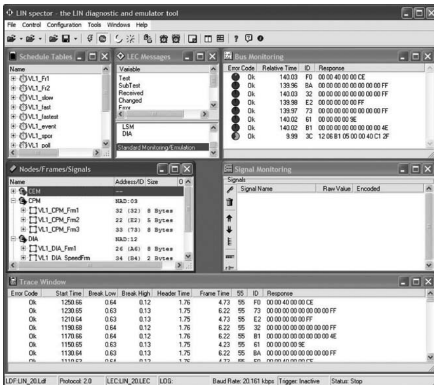
FIGURE 17.11 LIN Spector, diagnostics, and emulation tool for LIN.
