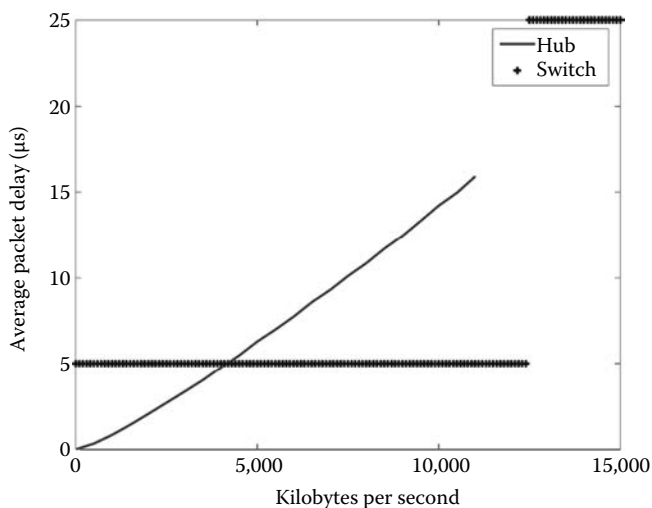
FIGURE 23.9 Packet delay as a function of node traffic for a hub and a switch [48]. Simulation results with baselines (delay magnitudes) computed from experiments.
