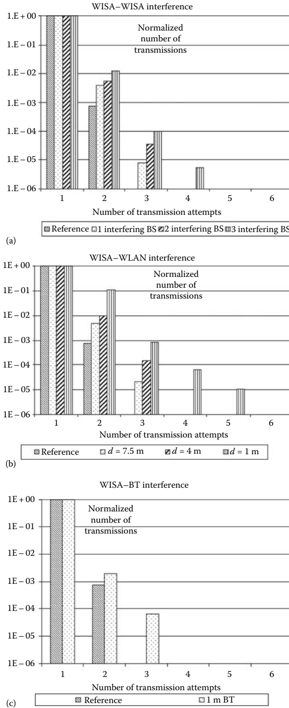
FIGURE 28.11 Measured retransmission statistics for WISA uplink messages due to interference (1 retransmit = 2048 \mu s). (a) WISA-WISA (1 m distance), (b) WISA-WLAN, (c) WISA-Bluetooth. (From Schieble, G., Dzung, D., Endresen, J., and Frey, J.-E., IEEE Ind. Electron. Mag. , 1, 25, 2007. With permission.)
