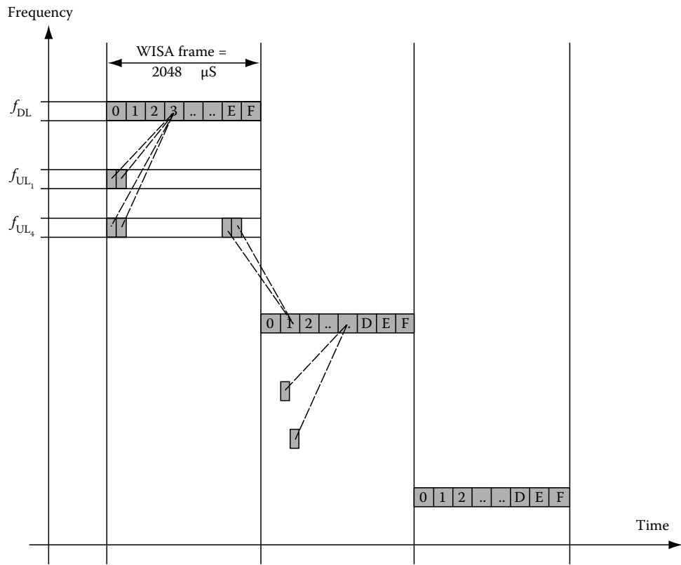
FIGURE 28.3 WISA TDMA/FDD/FH pattern. Dotted lines connect downlink/uplink slots allocated to one sensor/actuator. (TX/RX-turnaround time = 2 double slots = 256 \mu s, see Figure 28.4). (From Scheible, G., Dzung, D., Endresen, J., and Frey, J.-E., IEEE Ind. Electron. Mag. , 1, 25, 2007. With permission.)
