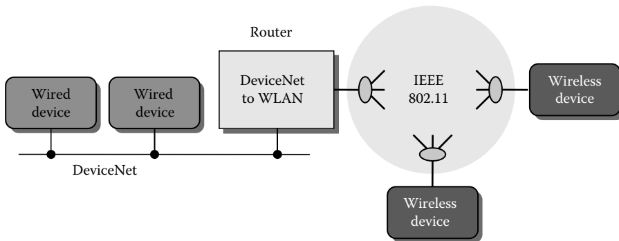
FIGURE 26.7 Extension of DeviceNet via a WLAN-enabled CIP router.
