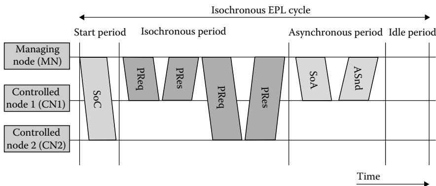
FIGURE 21.2 EPL timing.
