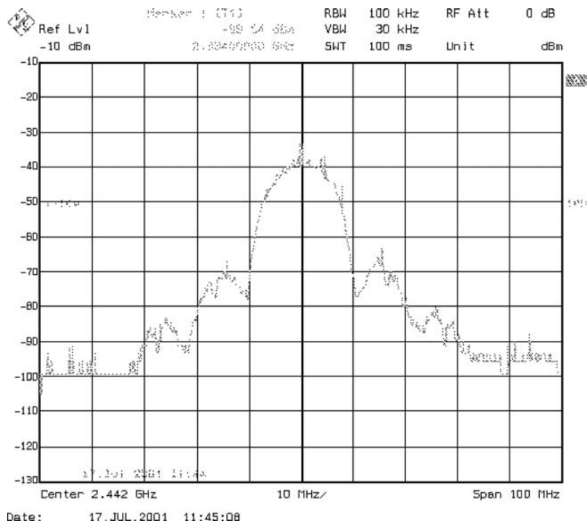
FIGURE 25.5 Measured spectrum of an IEEE 802.11b WLAN PCMCIA card. (From Matheus, K. Industrial Information Technology Handbook . Ed. R. Zurawski, CRC Press, Boca Raton, FL, 2004. With permission.)
