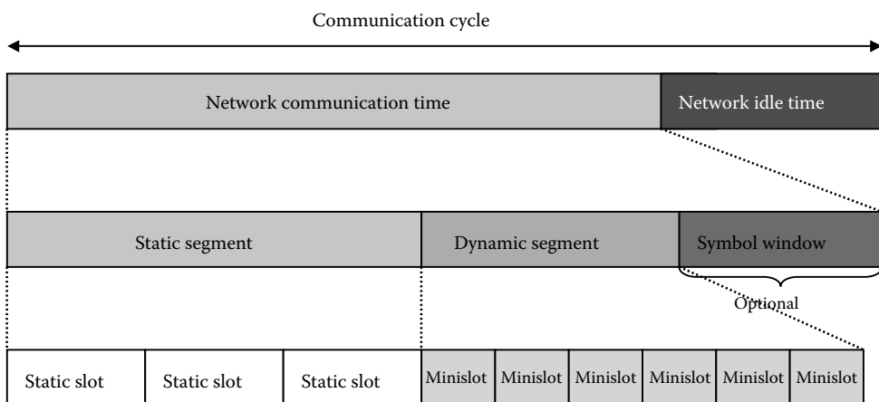
FIGURE 16.3 FlexRay communication cycle.
