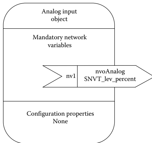
FIGURE 22.2 Functional profile for an analog input. (From Pitzek, S. and Elmenreich, W., Configuration and management of fieldbus systems. In R. Zurawski, ed., The Industrial Communication Technology Handbook . CRC Press, Boca Raton, 2005. With permission.)
