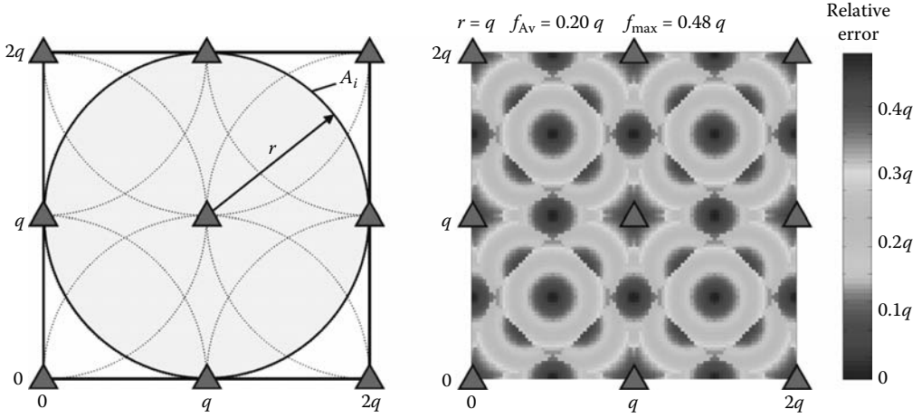
FIGURE 6.15 Scenario with a 3 \times 3 grid of beacons: (a) resulting overlaps and (b) localization error. (From Blumenthal, J. and Timmermann, D., 4th IEEE/ACM International Conference on Distributed Computing in Sensor Systems (DCOSS 2008) , pp. 47–48, Santorini, Griechenland, June 2008. With permission.)
