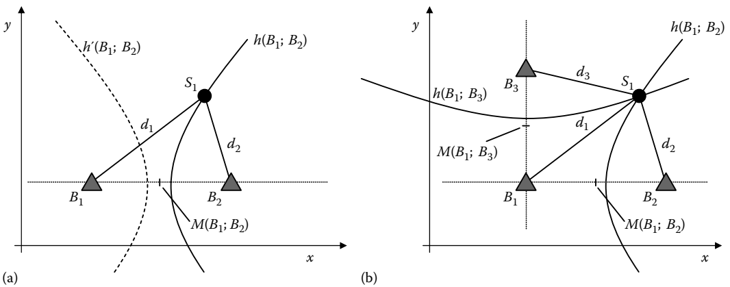
FIGURE 6.3 (a) Implicit distance estimation with time difference of arrival (TDoA) and (b) localization based on TDoA at intersection of h(B_1; B_2) and h(B_1; B_3) .
