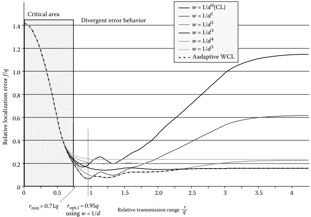
FIGURE 6.17 Localization error using different degrees. (From Blumenthal, J., Grosmann, R., Golatowski, F., and Timmermann, D., 1st European ZigBee Developer's Conference (EuZDC) , Munich, Germany, June 2007. With permission; Blumenthal, J., IEEE International Symposium on Intelligent Signal Processing, WISP 2007 , Madrid, Spain, October 2007. With permission.)
