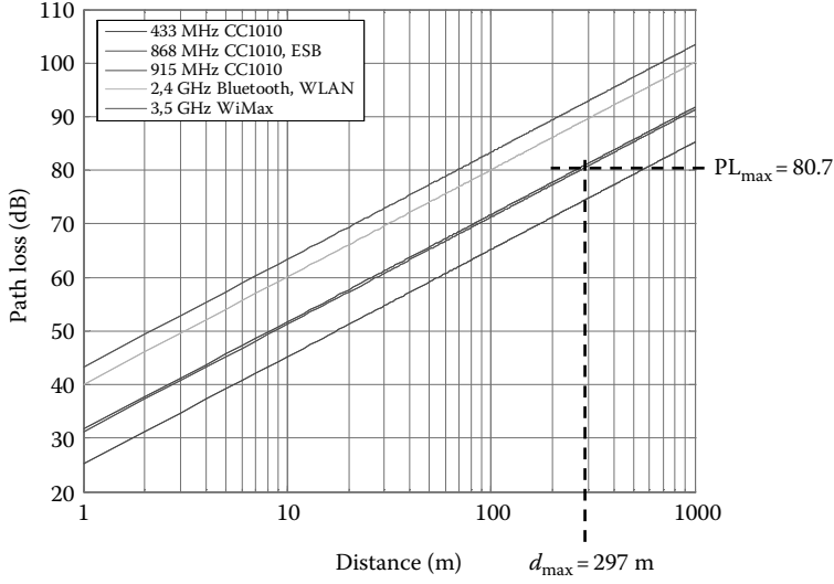
FIGURE 6.9 PL of radio signals over distance between sender and receiver at different frequencies, e.g., used by WiMax, WLAN, Chipcon CC1010, and ESB.
