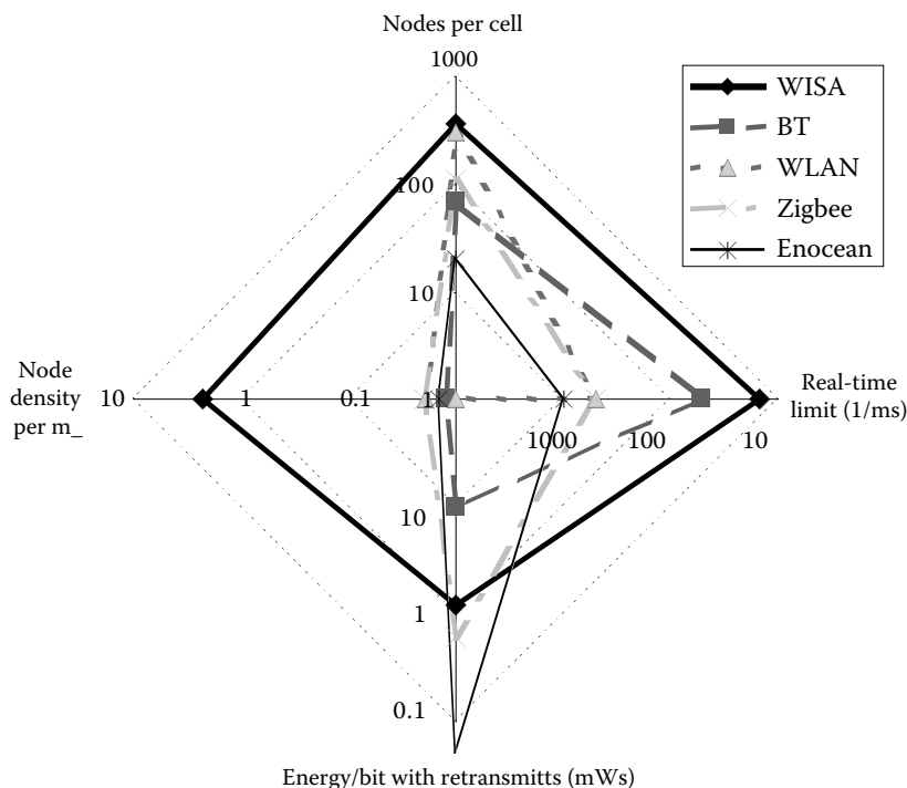
FIGURE 28.16 Visualization of comparison for the most important requirements in discrete factory automation (empirical, mind logarithmical scale). (From Scheible, G., Dzung, D., Endresen, J., and Frey, J.-E., IEEE Ind. Electron. Mag. , 1, 25, 2007. With permission.)
