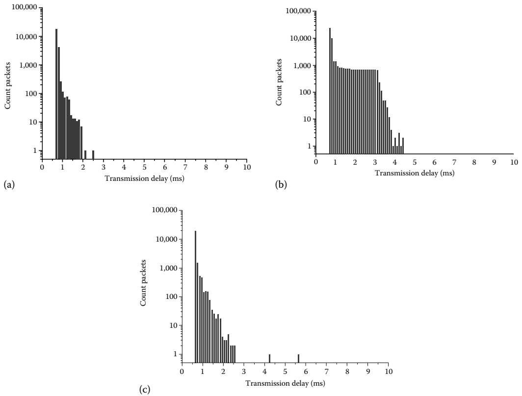
FIGURE 28.12 Measured WLAN-latency statistic (64 byte every 5 ms). (a) Reference measurement (no other frequency user). (b) with WISA in parallel, +2 ms downlink influence clearly visible (3 m distance). (c) same, but uplinks only (downlink in cable); four consecutive WISA nodes (50 events per second simultaneously)
