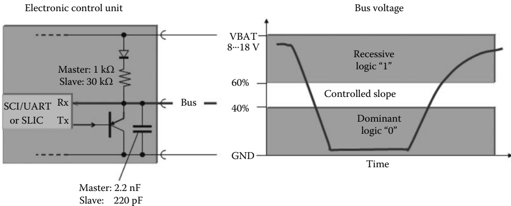
FIGURE 17.1 LIN logical level definitions. Note: The LIN specification refers to VBAT at the ECU connector.
