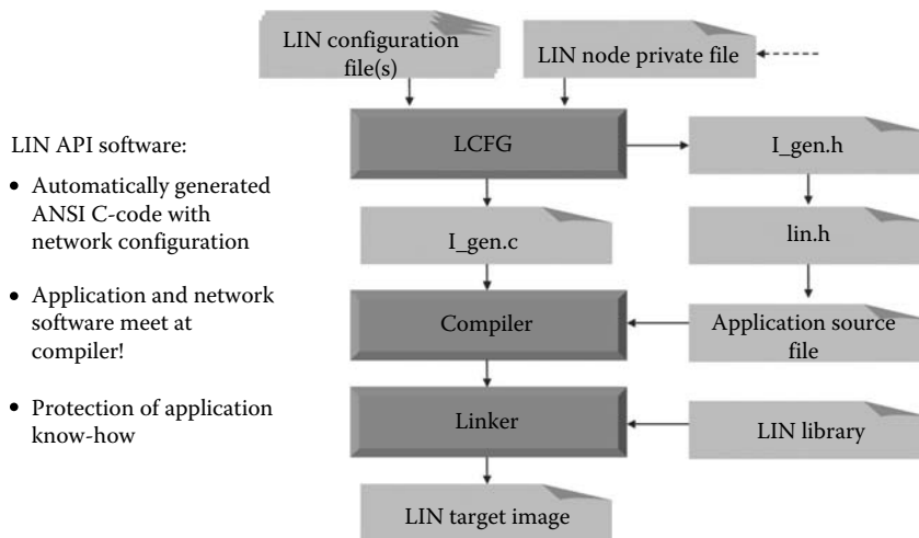
FIGURE 17.10 LIN target image building process.
