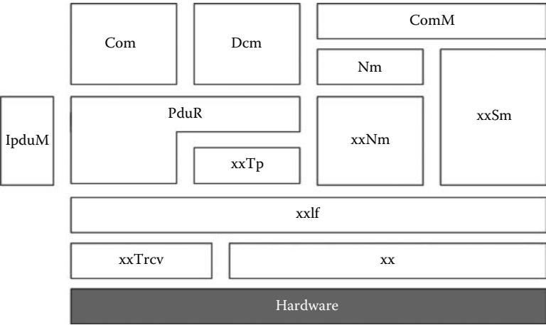
FIGURE 18.14 AUTOSAR—communication substack.
