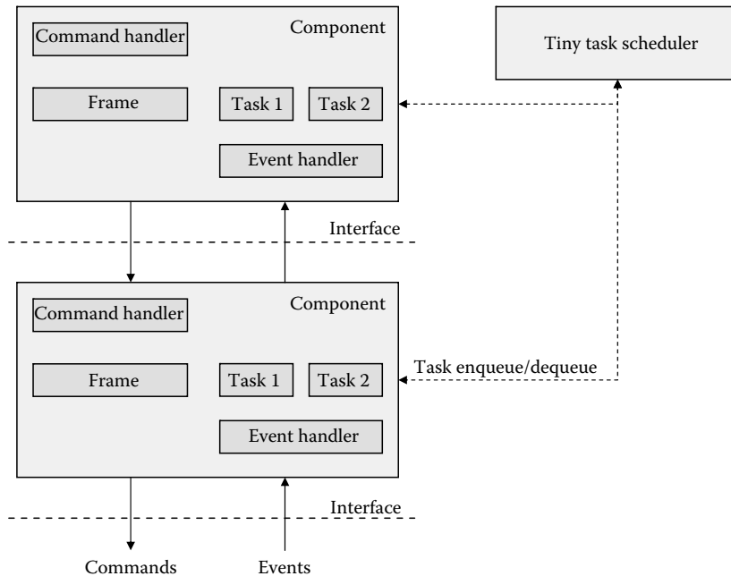
FIGURE 12.6 TinyOS architecture in detail.
