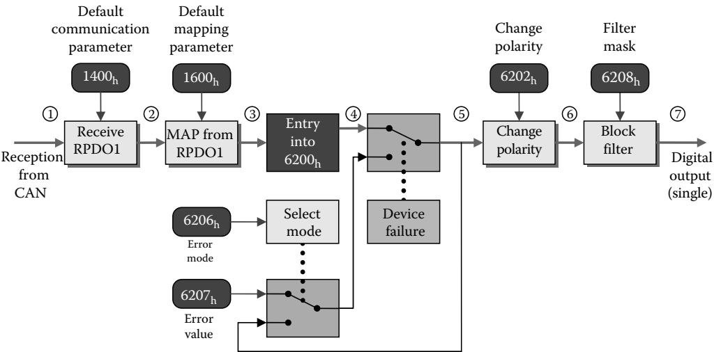
FIGURE 15.16 Conceptual architecture of digital outputs.
