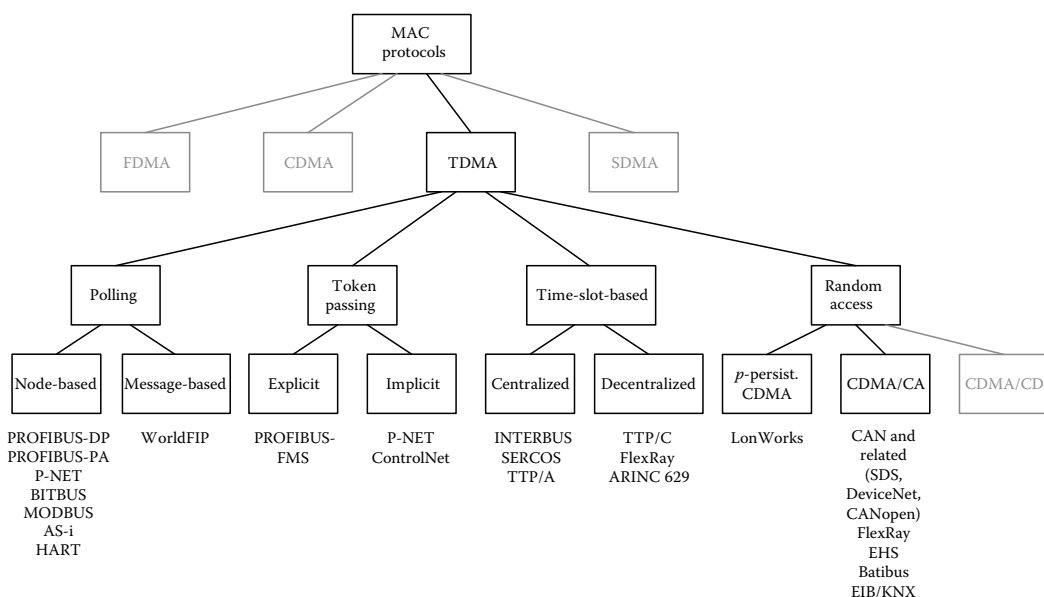
FIGURE 20.13 MAC strategies in fieldbus systems and examples.
