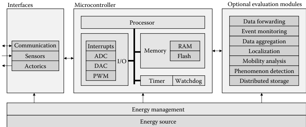
FIGURE 12.1 Structure of a sensor node.
