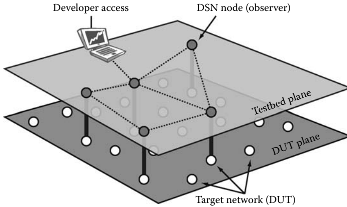
FIGURE 11.3 DSN is a WSN testbed that separates distributed observers (DSN nodes) and the target network under development or the DUT into two separate planes.
