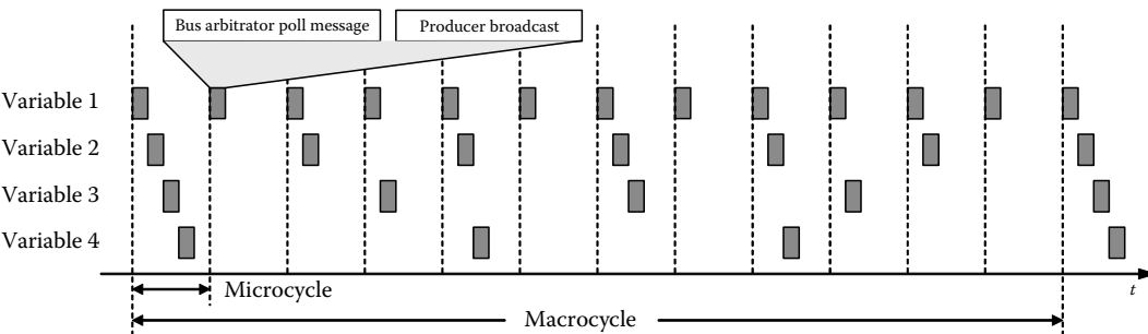
FIGURE 20.15 Bus cycle in WorldFIP.
