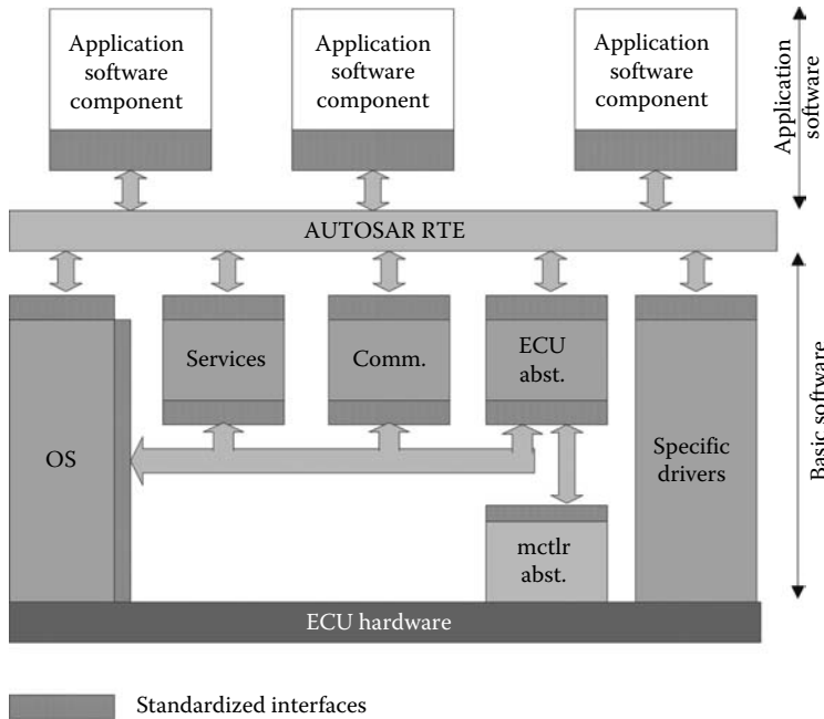
FIGURE 13.8 AUTOSAR reference architecture.
