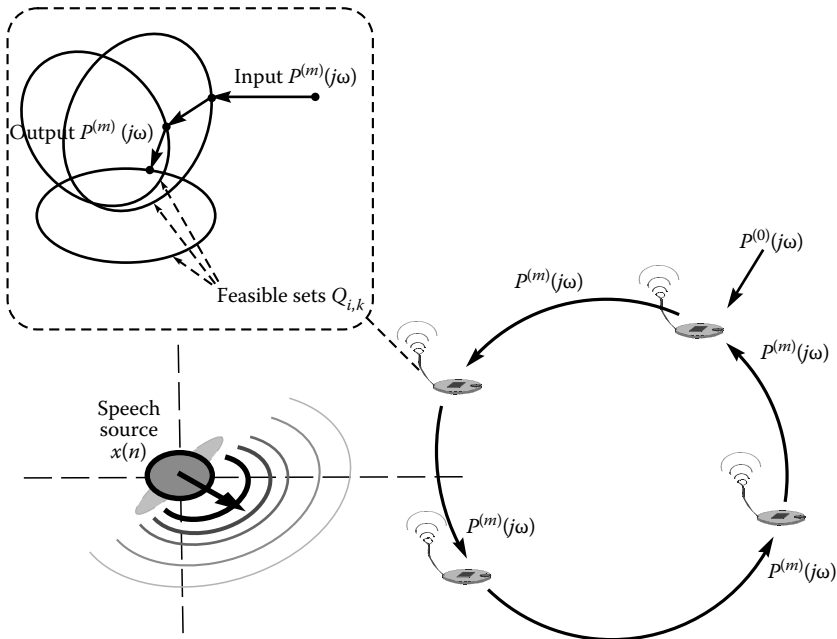
FIGURE 9.5 Graphical depiction of the Ring Algorithm. For illustrative reasons, only three feasible sets Q_{i,k} are shown in the inside picture. Also, it is shown that the output spectrum P^{(m)}(e^{j\omega}) is obtained from the input P^{(m)}(e^{j\omega}) only after three projections. In practice, each sensor node has L feasible sets and has to repeat the sequence of projections many times before it can successfully project the input P^{(m)}(e^{j\omega}) into the intersection of its feasible sets.
