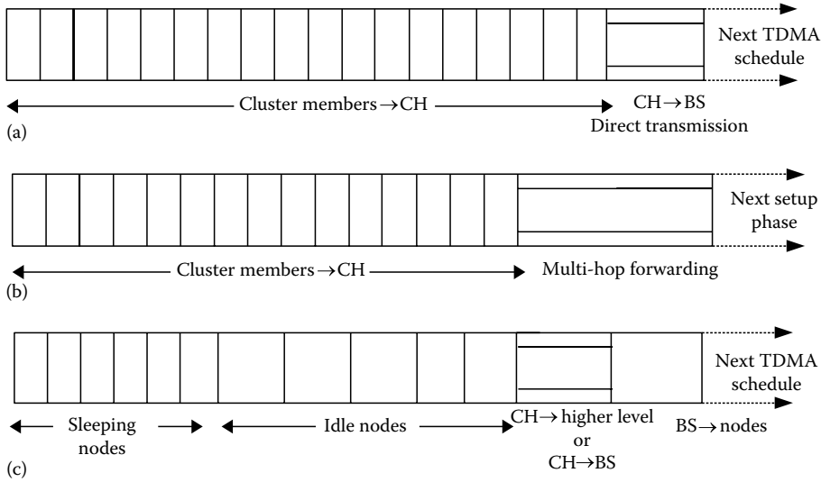
FIGURE 7.5 Super-frame comparisons between LEACH, MECH, and APTEEN. (a) LEACH transmission schedule. (b) MECH transmission and forwarding phases. (c) APTEEN transmission schedule.
