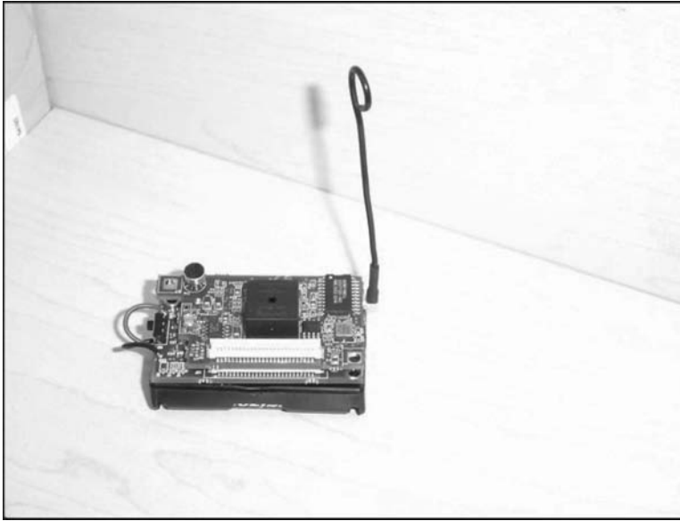
FIGURE 9.1 Wireless sensor node or Mote made by Crossbow Technology, Inc. in San Jose, California.
