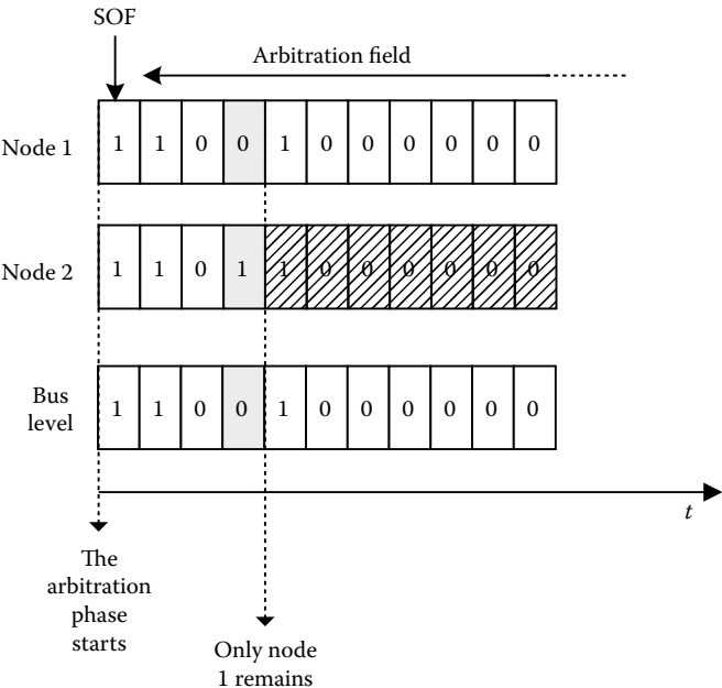
FIGURE 13.3 CAN arbitration phase with two nodes starting transmitting simultaneously. Node 2 detects that a frame with a higher priority than its own is being transmitted when it monitors a level 0 (i.e., dominant level) on the bus while it has sent a bit with a level 1 (i.e., recessive level). Afterwards, Node 2 immediately stops transmitting. (From Navet, N., Song, Y.Q., Simonot-Lion, F., and Wilwert, C., Proc. IEEE. , 93(6), 1204, 2005. With permission.)
