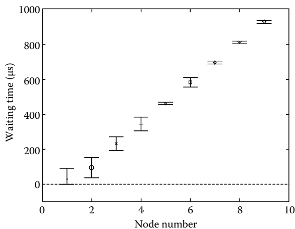
FIGURE 23.4 Nine identical devices with strobed message connection.
