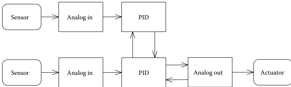
FIGURE 22.4 Example for an application model. (From Pitzek, S. and Elmenreich, W., Configuration and management of fieldbus systems. In R. Zurawski, ed., The Industrial Communication Technology Handbook . CRC Press, Boca Raton, 2005. With permission.)
