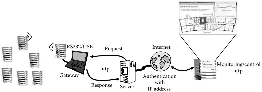
FIGURE 12.28 A deployed wireless sensor network.
