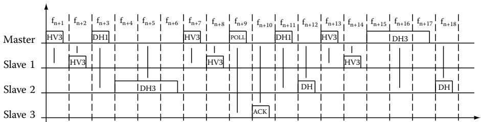
FIGURE 25.3 Example slot occupation within one piconet consisting of master and three slaves; to slave 1 there is an SCO-link, to slave 2 (best-effort) traffic is transmitted in both directions, slave 3 has currently nothing to send (but has to respond to the POLL-packet with an ACK); during the transmission of multislot packets the frequency is not changed. (From Matheus, K. Industrial Information Technology Handbook . Ed. R. Zurawski, CRC Press, Boca Raton, FL, 2004. With permission.)
