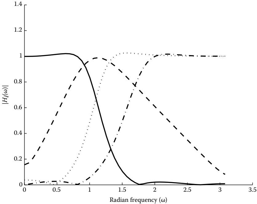
FIGURE 9.6 Frequency response amplitude of the transfer functions used in Example 9.3. The curves show, from left to right, |H_0(e^{j\omega})| , |H_1(e^{j\omega})| , |H_2(e^{j\omega})| , and |H_3(e^{j\omega})| .
