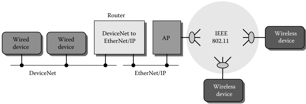
FIGURE 26.6 Extension of DeviceNet via a CIP router and an AP.
