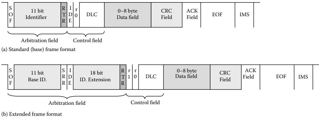
FIGURE 15.3 Format of data frames.
