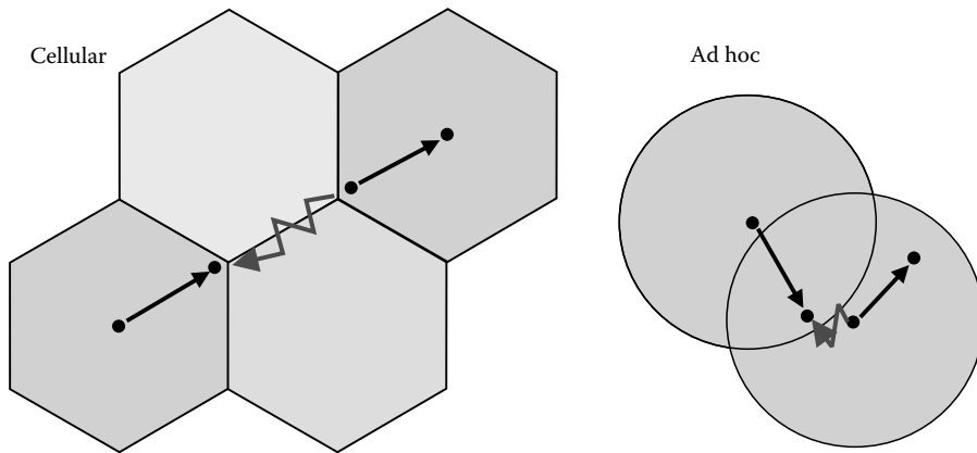
FIGURE 25.2 Closest next co-channel interferer in cellular and ad hoc networks. (From Matheus, K. Industrial Information Technology Handbook . Ed. R. Zurawski, CRC Press, Boca Raton, FL, 2004. With permission.)
