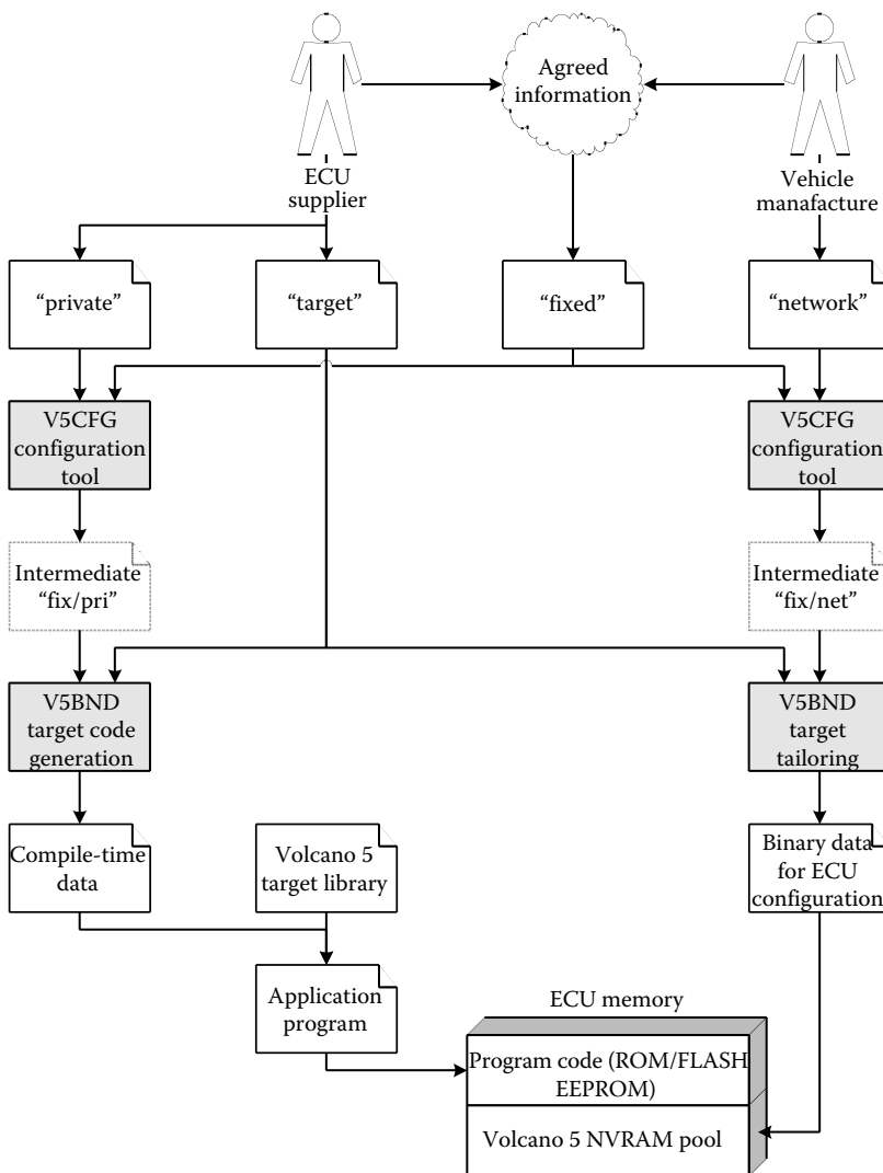
FIGURE 19.7 Configuration of Volcano target software.
