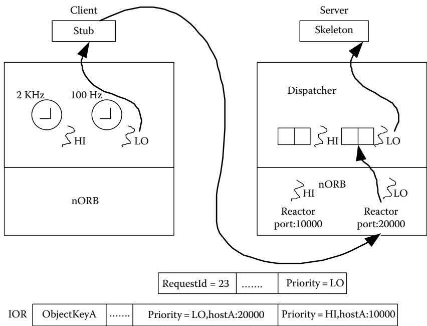
FIGURE 2.5 Priority propagation in nORB.
