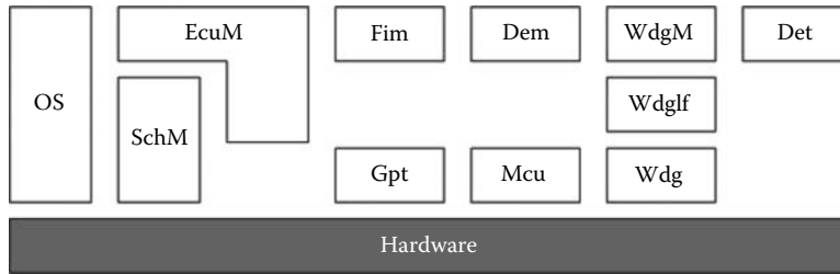
FIGURE 18.17 AUTOSAR—system services substack.
