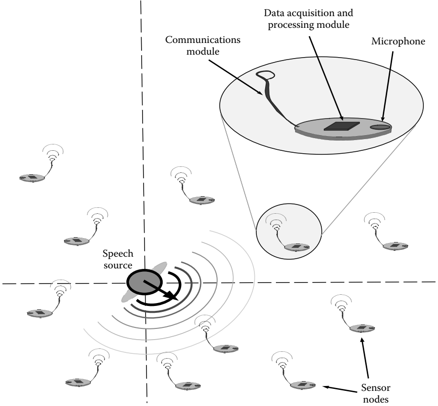
FIGURE 9.2 Sensor network monitoring a stationary sound source in room.
