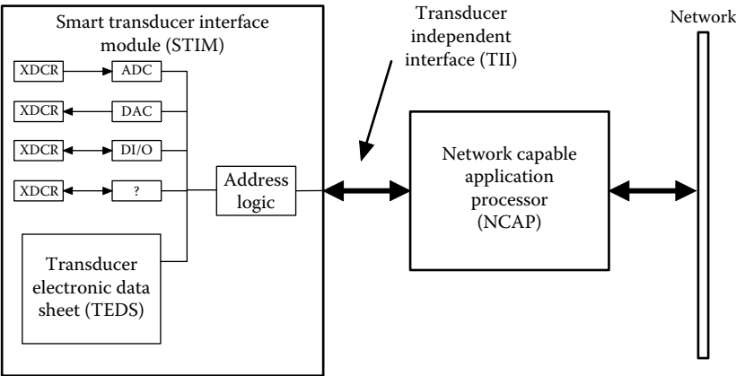
FIGURE 22.3 STIM connected to NCAP. (From Pitzek, S. and Elmenreich, W., Configuration and management of fieldbus systems. In R. Zurawski, ed., The Industrial Communication Technology Handbook . CRC Press, Boca Raton, 2005. With permission.)
