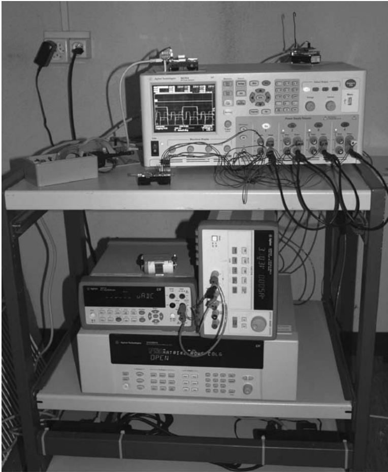
FIGURE 11.9 Testbed setup consists of a monitoring node, an interface board for power measurements, a supply, and the DUT.
