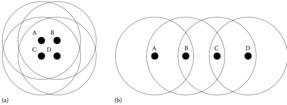
FIGURE 12.26 (a) Physically arranged sensor nodes (solid circles). All nodes are in transmission range (dotted line) of each other. (b) Virtually arranged nodes with appropriated transmission ranges. Nodes are not longer able to communicate without routing.
