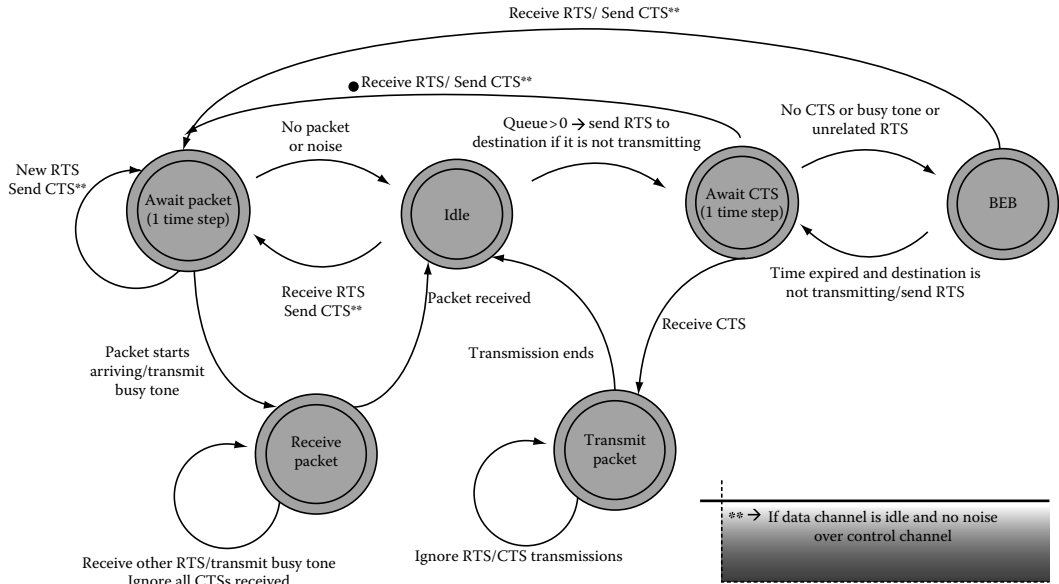
FIGURE 8.2 PAMAS protocol. (Redrawn from Singh, S. and Raghavendra, C.S., Comput. Commun. Rev. , 28(3), 5, 1998.)
