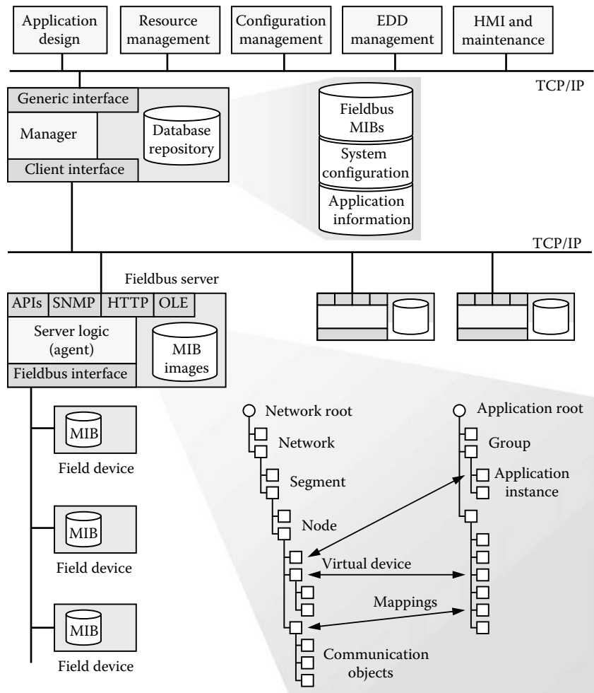
FIGURE 20.25 NOAH system architecture.
