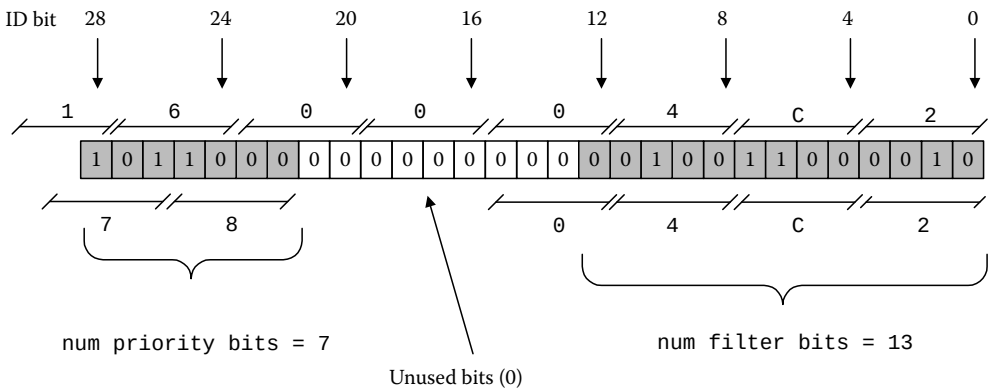
FIGURE 19.5 CAN ID filtering scheme in volcano.
