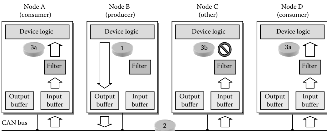
FIGURE 15.5 Producer/consumer model.
