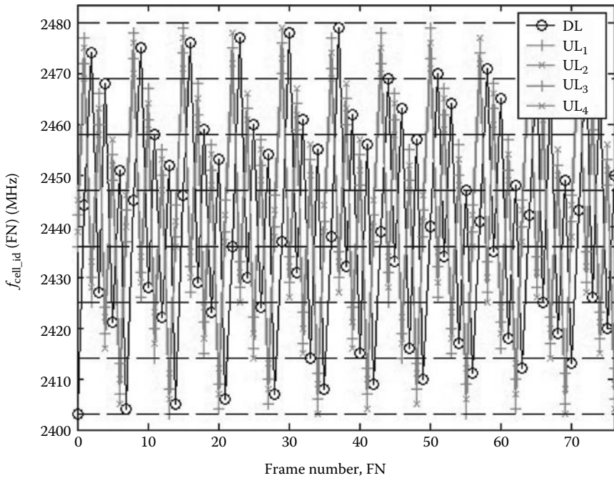
FIGURE 28.6 Example FH sequences (cell_id = 27). (From Schieble, G., Dzung, D., Endresen, J., and Frey, J.-E., IEEE Ind. Electron. Mag. , 1, 25, 2007. With permission.)
