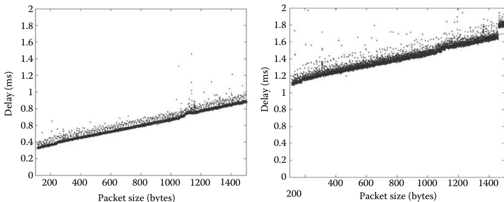
FIGURE 23.5 Example of the impact of VPN security encryption on Ethernet network performance (the figure on the left is the round-trip delay measured for user datagram protocol (UDP)* packet transmission on a 100 Mbps switched Ethernet network; the figure on the right is the delay measured for the same system, but with VPN encryption added).
