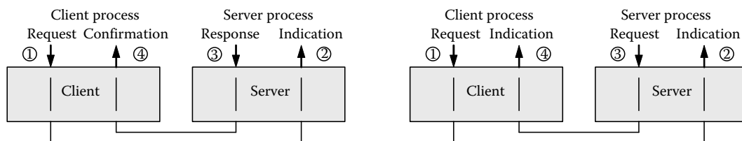
FIGURE 20.21 Communication services used in the client–server model (left: normal; right: based on unconfirmed services).
