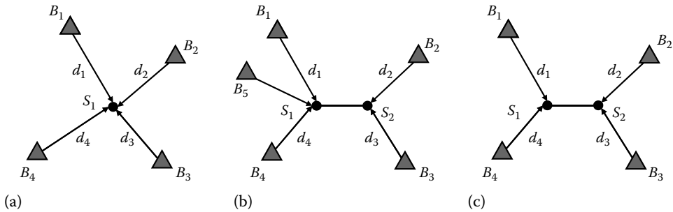
FIGURE 6.20 (a) Atomic, (b) iterative, and (c) collaborative multilateration.
