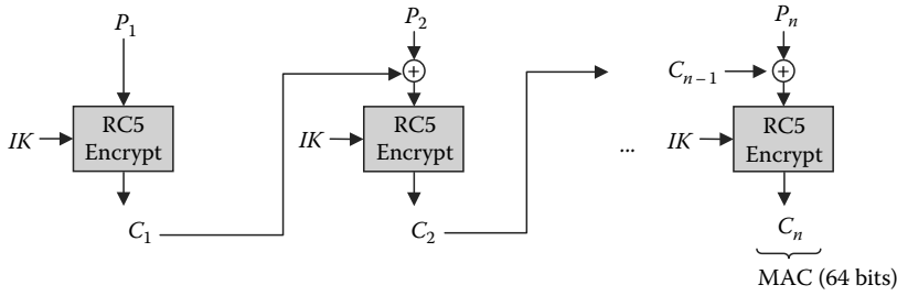
FIGURE 10.6 Computing an MAC in cipher block chaining mode.
