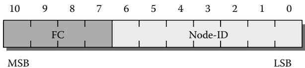
FIGURE 15.14 CAN-ID in the predefined connection set.
