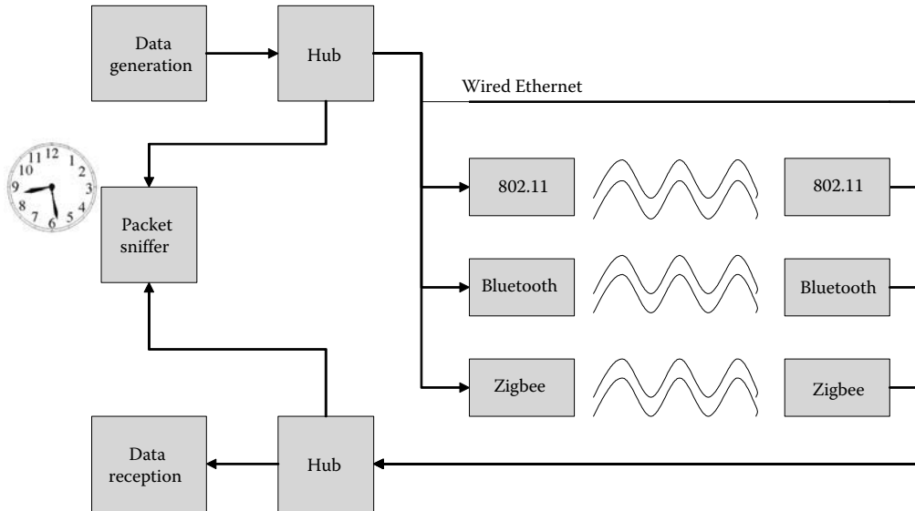
FIGURE 23.20 Experimental setup for determining and investigating the wireless NCS performance.
