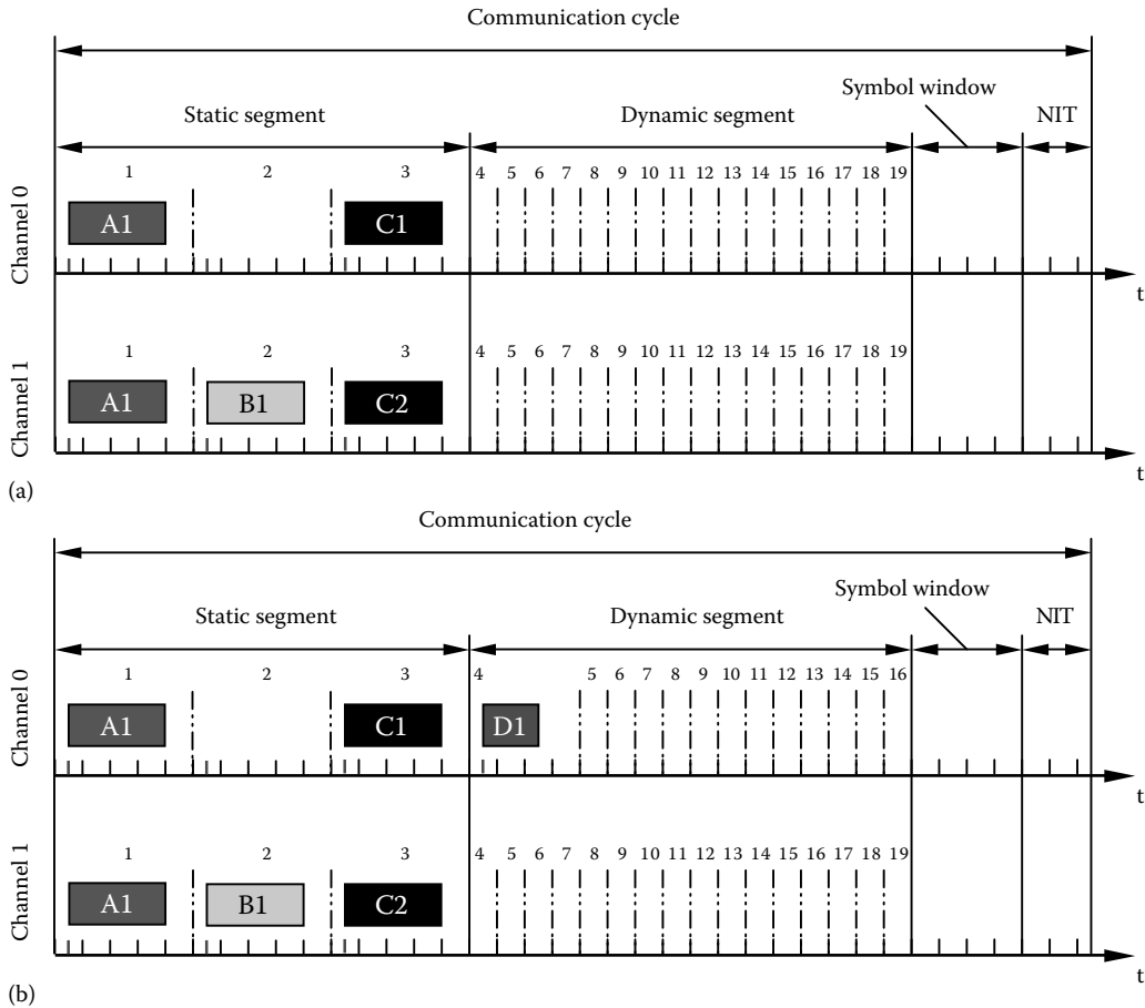
FIGURE 16.4 FlexRay dynamic segment.
