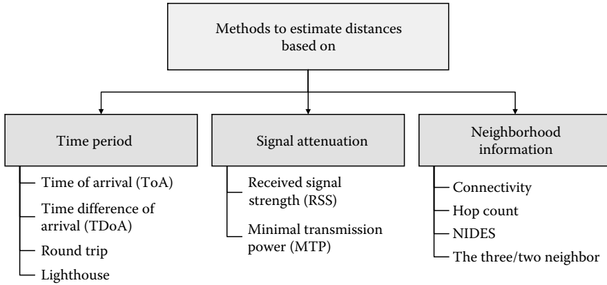
FIGURE 6.1 Classification of distance estimation methods.
