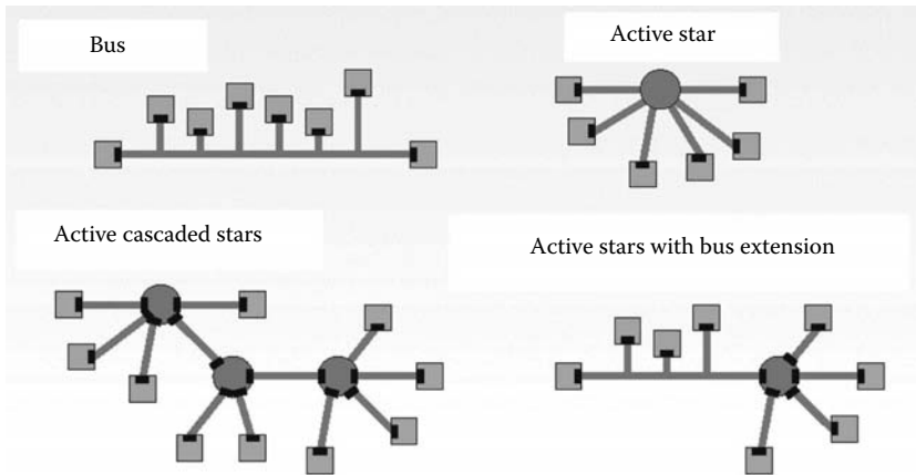
FIGURE 16.8 Topologies.
