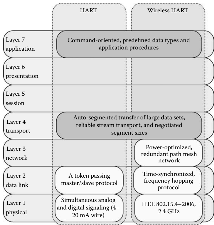
FIGURE 27.10 HART and WirelessHART protocol stacks.
