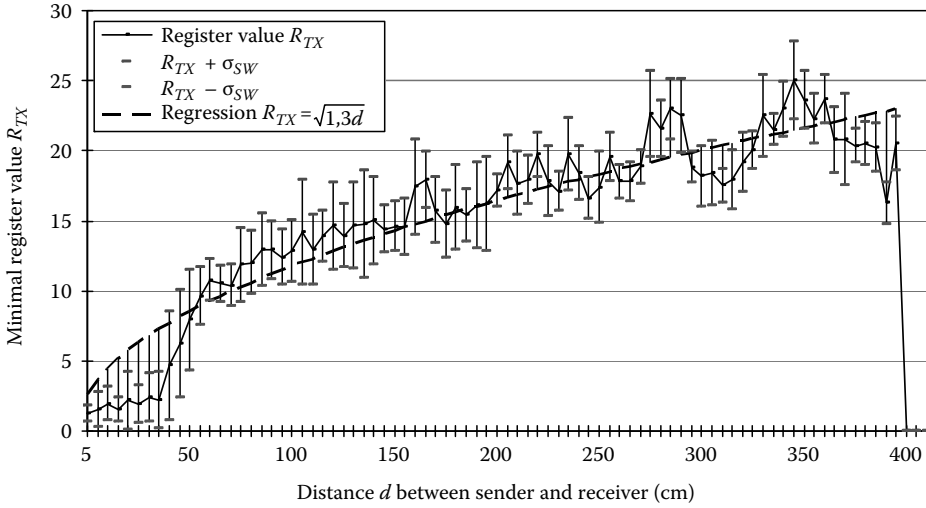
FIGURE 6.11 Register value R_{TX} of minimal transmission power P_{TX,\min} depending on the distance (ESB, 40 measurements).
