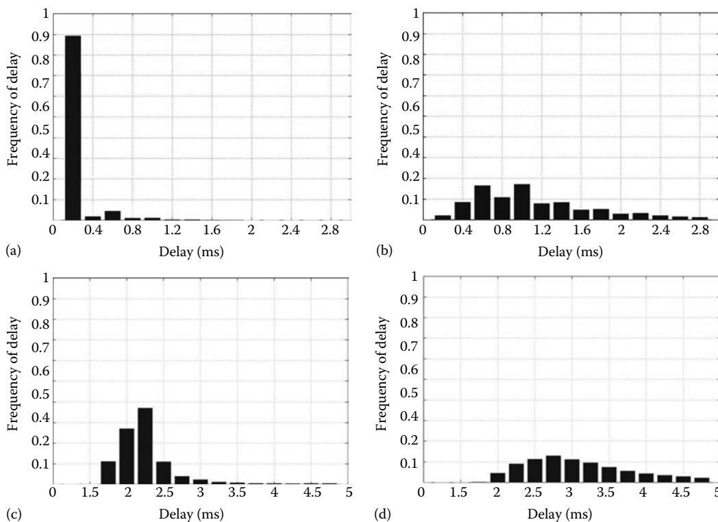
FIGURE 23.13 Distributions of packet delays for different values of cross-traffic throughput on an 802.11a network. (a) UDP delays, 3Mb/s cross-traffic, (b) UDP delays, 22Mb/s cross-traffic, (c) OPC delays, 3Mb/s cross-traffic, and (d) OPC delays, 22Mb/s cross-traffic.
