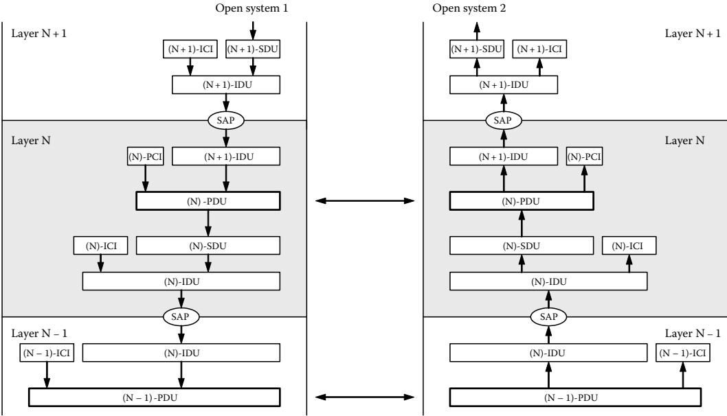
FIGURE 20.5 Communication in the OSI model.
