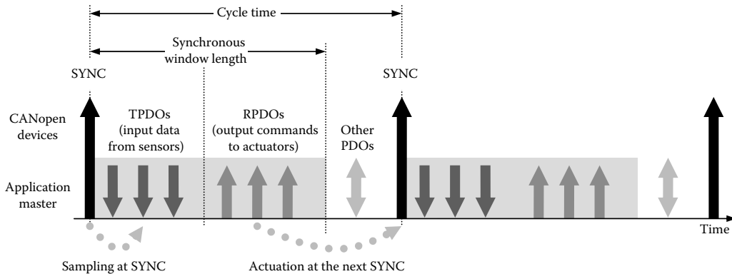
FIGURE 15.11 Synchronous operation.
