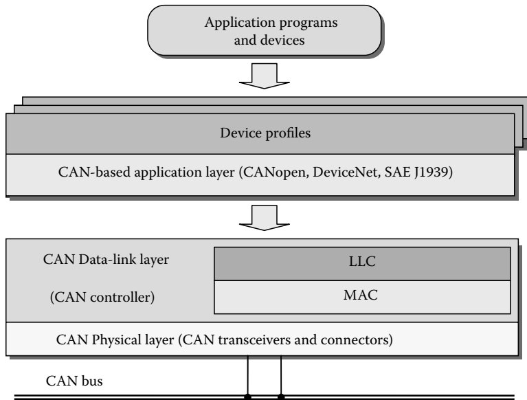
FIGURE 15.1 CAN protocol stack.
