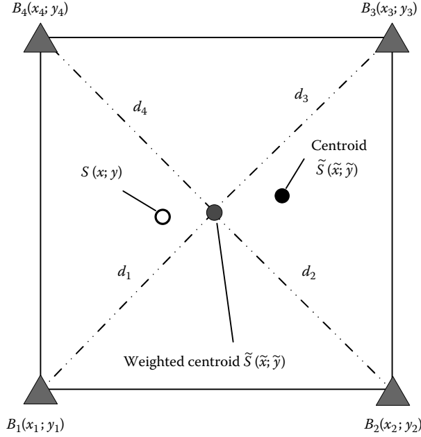
FIGURE 6.16 WCL compared to CL. (From Reichenbach, F., Resource aware algorithms for exact localization in wireless sensor networks, PhD thesis, University of Rostock, Rostock, Germany, December 2007. With permission.)
