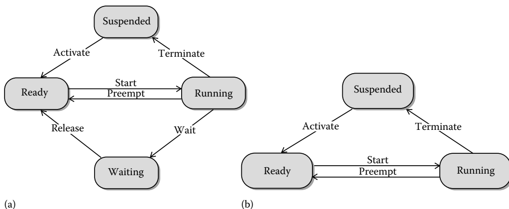
FIGURE 18.3 OSEK OS task states.
