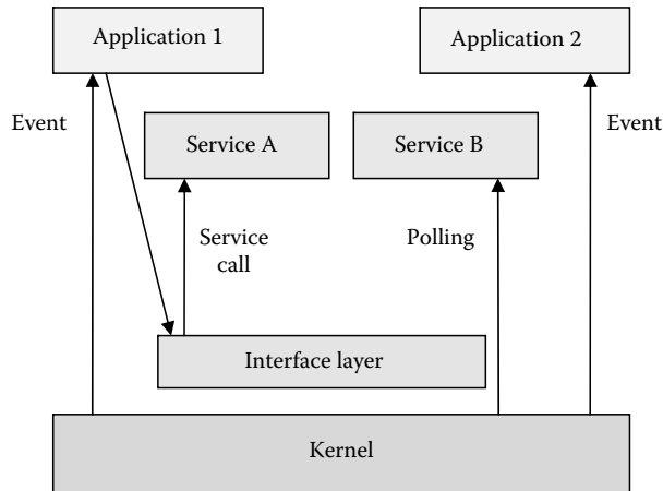
FIGURE 12.18 Interprocess operations in Contiki.
