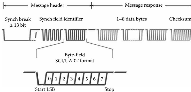
FIGURE 17.2 Frame structure.
