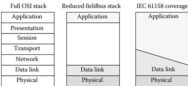
FIGURE 20.11 Layer structure of a typical fieldbus protocol stack as defined by the IEC 61158. (From Sauter, T., in The Industrial Communication Technology Handbook , CRC Press, Boca Raton, FL, 2005, 24.1–24.19. With permission.)
