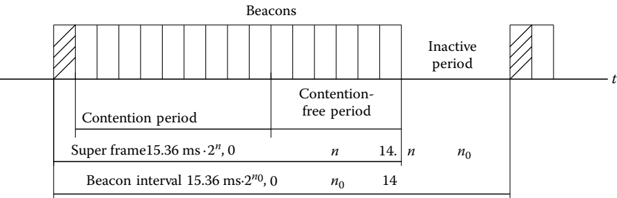
FIGURE 25.6 Optional IEEE 802.15.4/ZigBee beacon interval and super frame.
