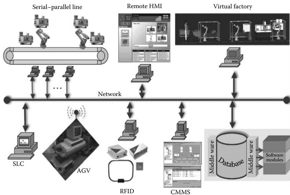
FIGURE 23.17 Reconfigurable factory testbed.
