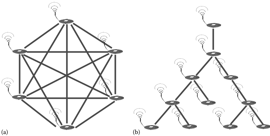
FIGURE 9.11 Other possible topologies for distributed sensor network fusion using the convex feasibility paradigm: (a) fully-connected topology and (b) tree topology.
