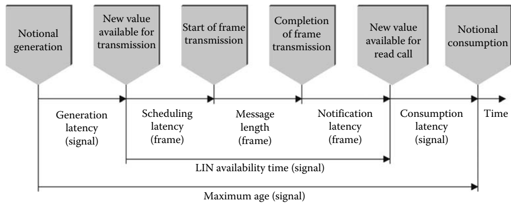
FIGURE 17.8 LIN timing model.
