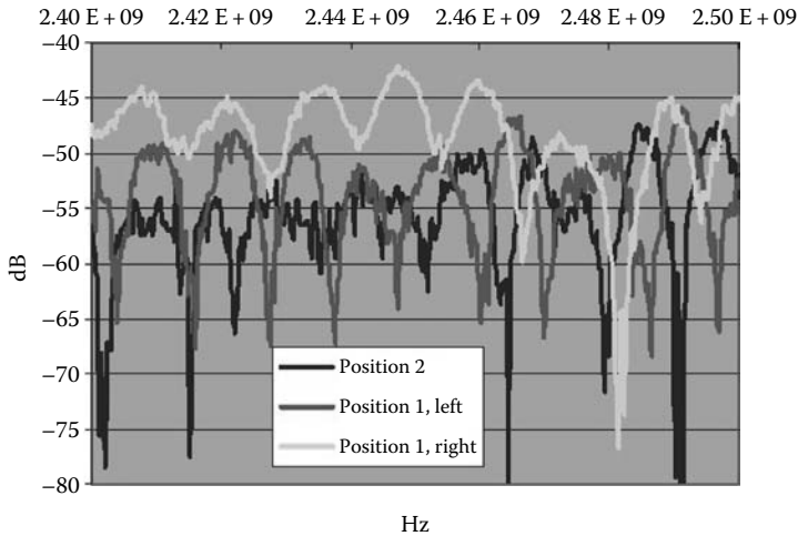
FIGURE 28.5 Frequency selective fading in the 2.4 GHz ISM band: frequency-dependent attenuation from a sensor/actuator to three BS antennas in a test installation. Gray and light gray: pair of base station antennas, separated by 37 cm. Black: third BS antenna, line of sight path obstructed by a robot arm. (From Schieble, G., Dzung, D., Endresen, J., and Frey, J.-E., IEEE Ind. Electron. Mag. , 1, 25, 2007. With permission.)
