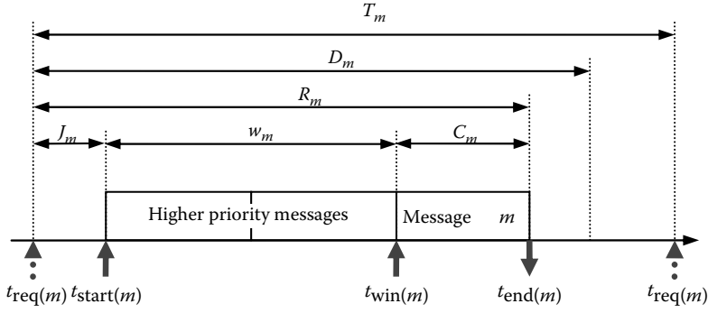
FIGURE 15.6 Worst-case response time in CAN.
