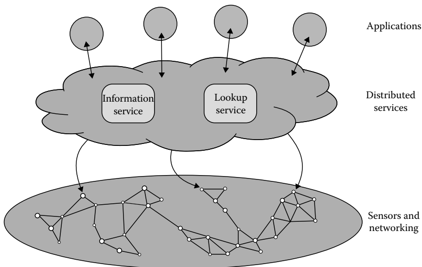
FIGURE 4.5 EYES project architecture description.
