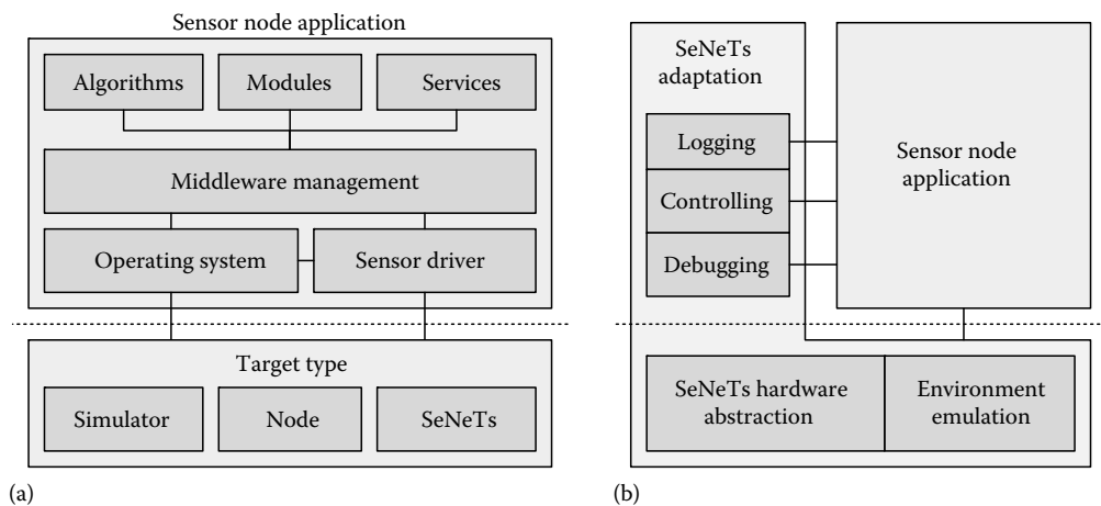
FIGURE 12.24 (a) Software layer model of a SNA and (b) Software layer model of a SeA.
