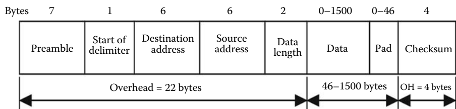
FIGURE 23.8 Ethernet (CSMA/CD) frame format; 20 Byte interframe space not shown.
