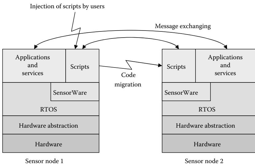
FIGURE 12.11 Sensor node architecture.
