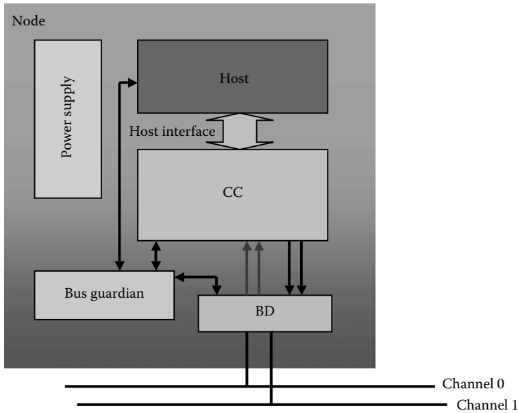
FIGURE 16.2 ECU architecture.
