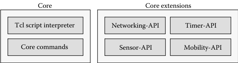
FIGURE 12.9 SensorWare scripting language.
