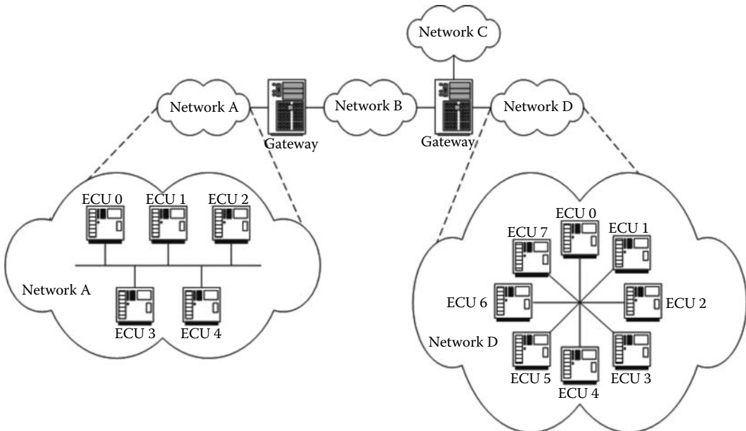
FIGURE 18.1 Hardware architecture—system and network level.
