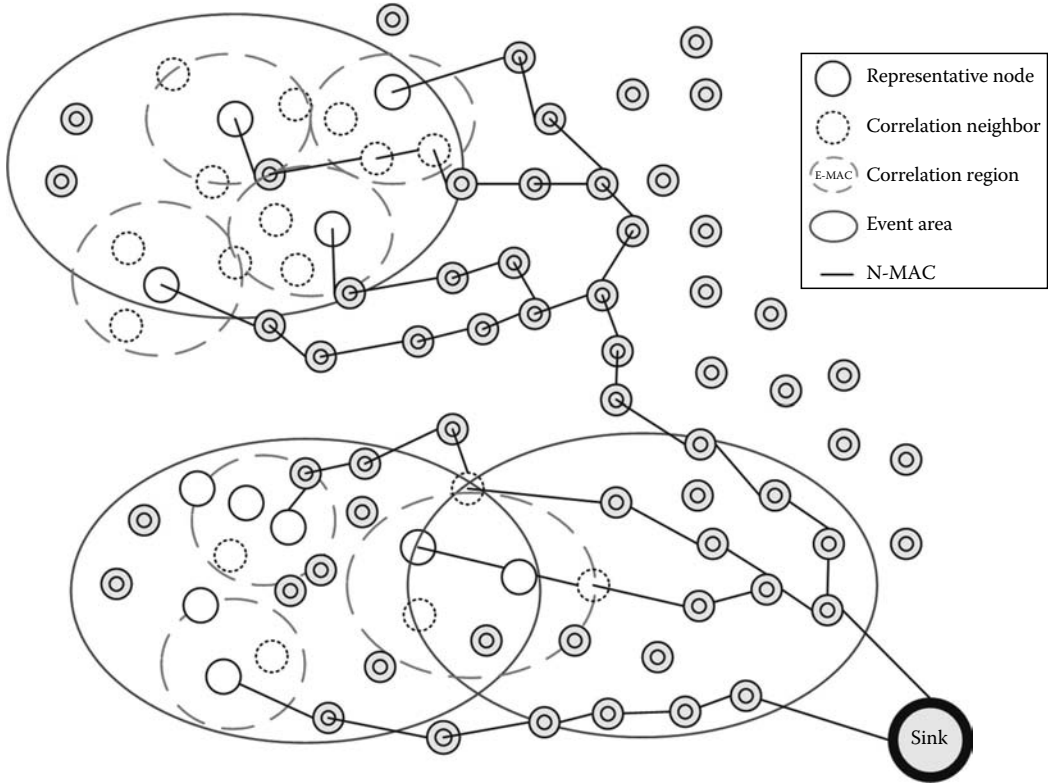
FIGURE 8.4 CC-MAC protocol operations. (Redrawn from Vuran, M.C. and Akyildiz, I.F., IEEE/ACM Trans. Network. , 14(2), 316, 2006.)
