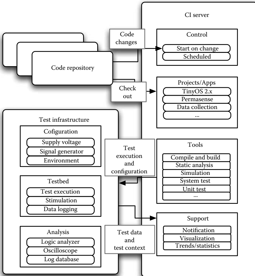
FIGURE 11.5 Overview of the test and instrumentation architecture.
