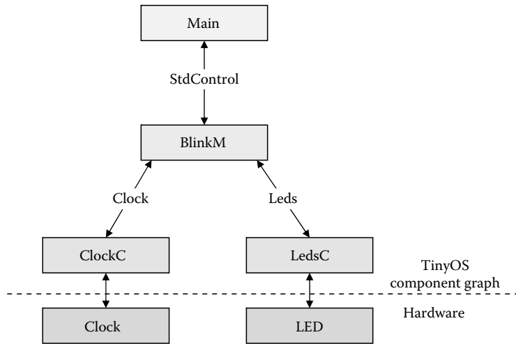
FIGURE 12.7 Simple TinyOS application.
