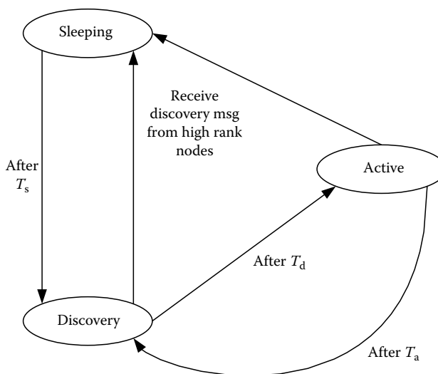
FIGURE 7.8 State transitions of the GAF protocol.
