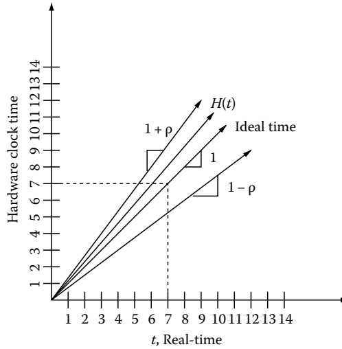
FIGURE 5.1 Drifting of hardware clock time.
