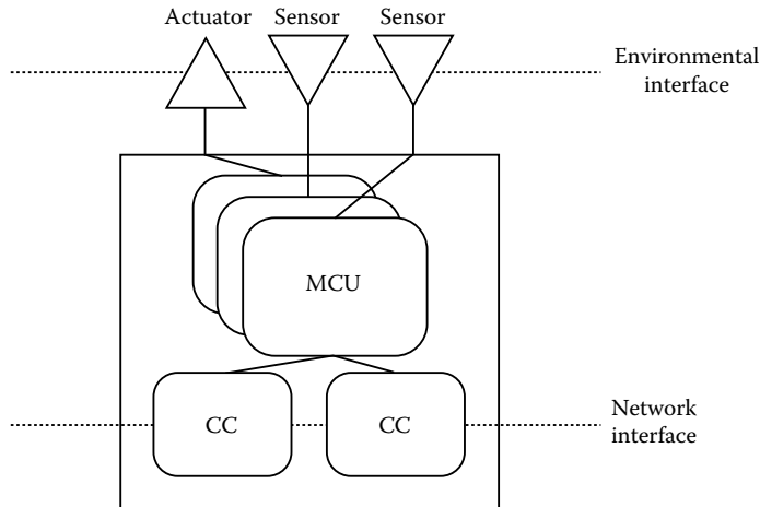
FIGURE 18.2 Hardware architecture—ECU level.
