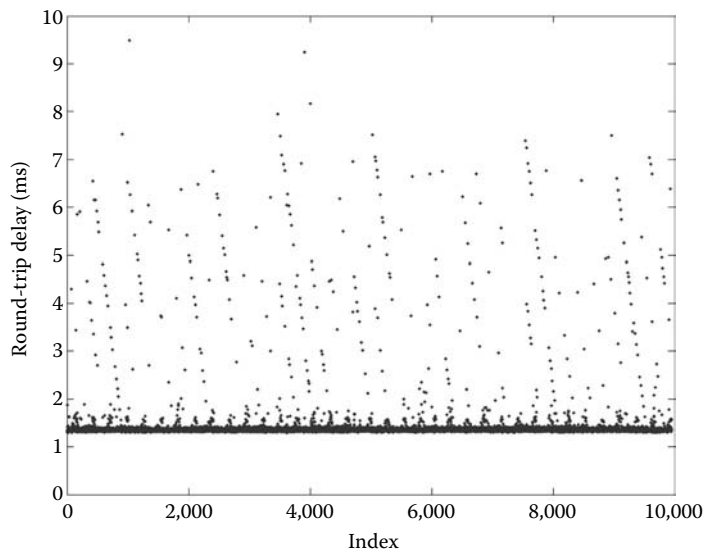
FIGURE 23.11 Illustration of overhead delay associated with OPC over a 100 Mb/s switched Ethernet network. Mean = 1.5 ms with standard deviation = 0.03 ms; for comparison purposes the mean UDP round-trip time over the same network is 0.33 ms.
