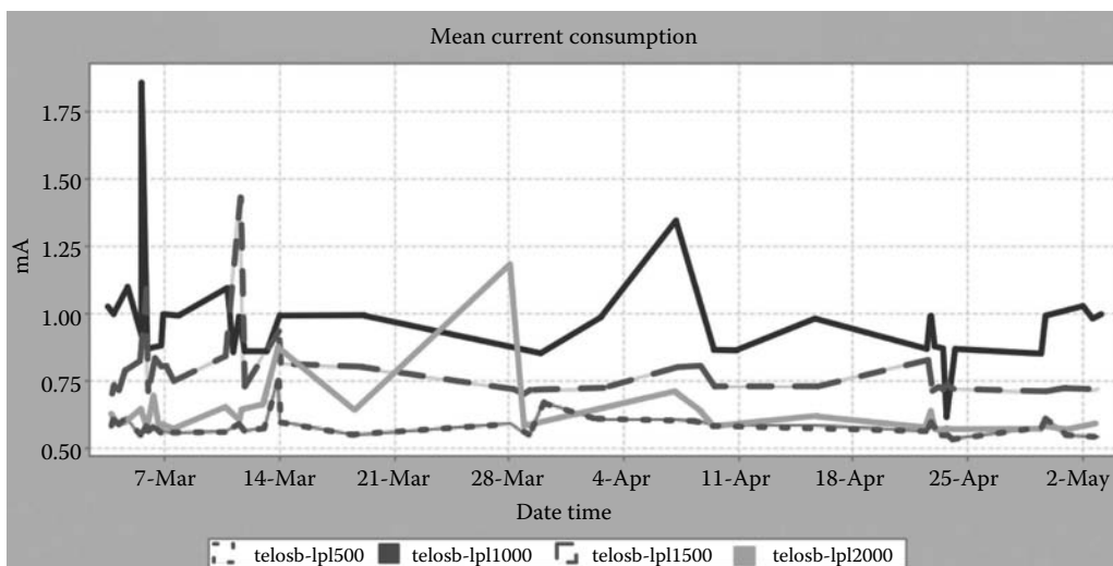
FIGURE 11.8 Parametrized data collection application project: plot of average power consumption for different sleep intervals.
