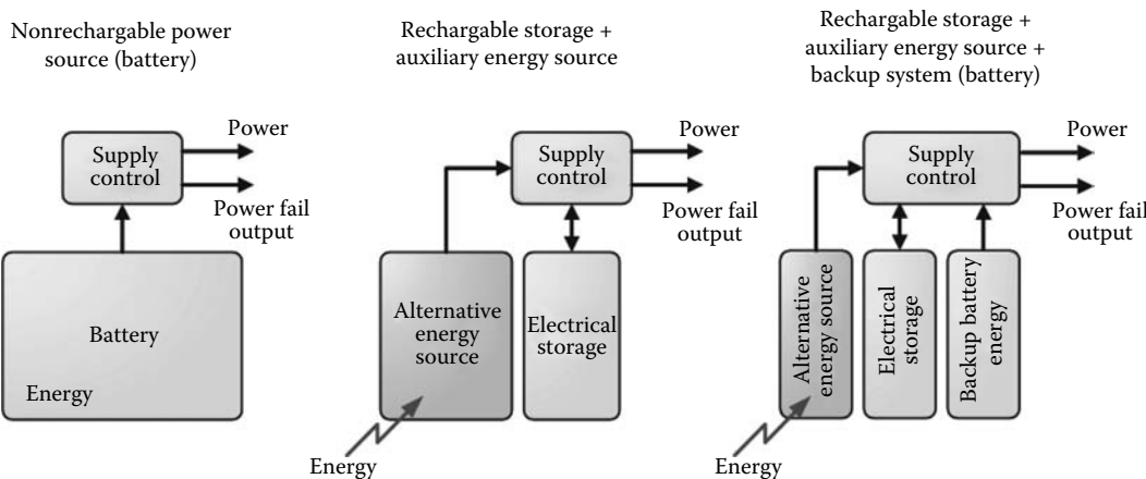
FIGURE 27.17 Power management.
