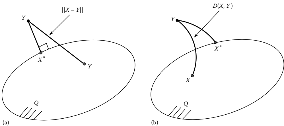
FIGURE 9.4 (a) Symbolic depiction of metric projection and (b) generalized projection of a vector Y into a closed convex set \mathcal{Q} . In (a) the projection X^* is selected by minimizing the metric \|X - Y\| over all X \in \mathcal{Q} while in (b) X^* is found by minimizing the generalized distance D(X, Y) over the same set.
