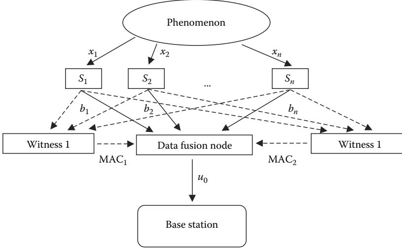
FIGURE 10.9 Overview of the witness-based approach [DDHV03b].
