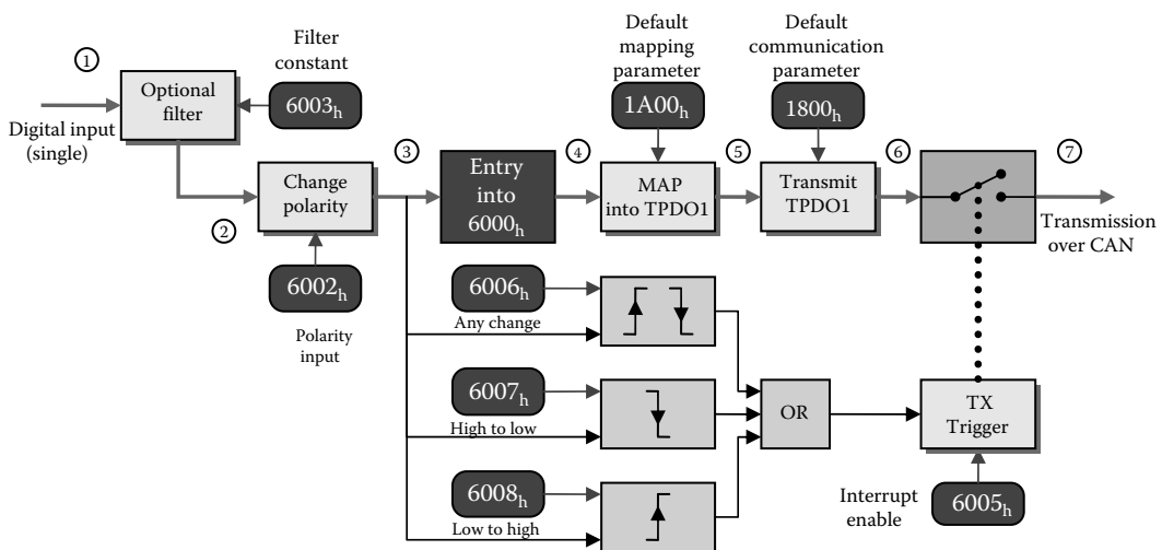
FIGURE 15.15 Conceptual architecture of digital inputs.
