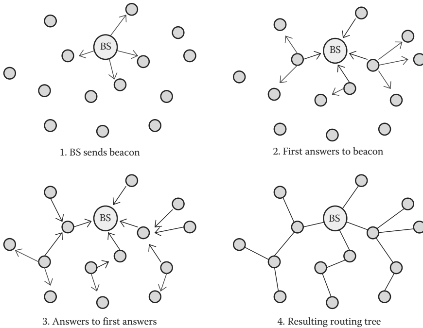
FIGURE 10.2 Breadth first search.
