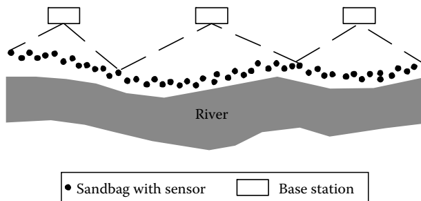
FIGURE 12.2 Example sensor network application: leakage detection along dikes.
