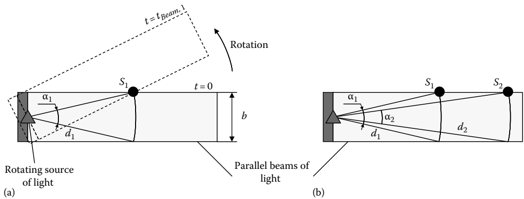
FIGURE 6.6 Lighthouse localization system: (a) Angle detection and (b) distance estimation depending on angles.
