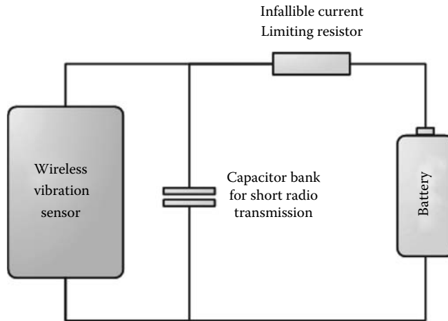
FIGURE 27.14 Battery design.
