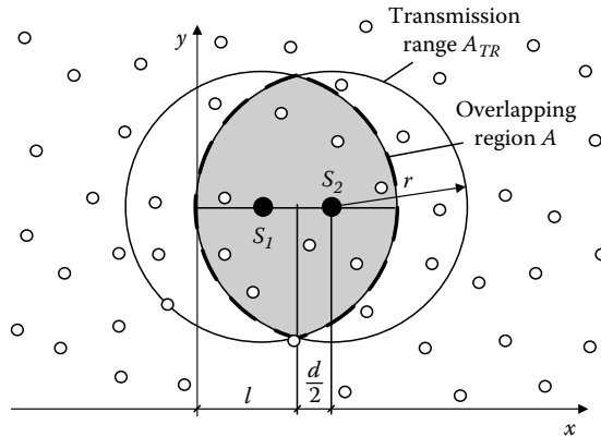
FIGURE 6.8 Neighborhood intersection distance estimation schema.
