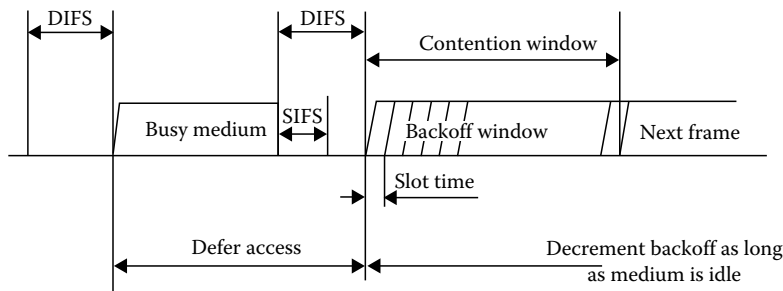
FIGURE 23.12 Timing diagram for wireless Ethernet (IEEE 802.11).
