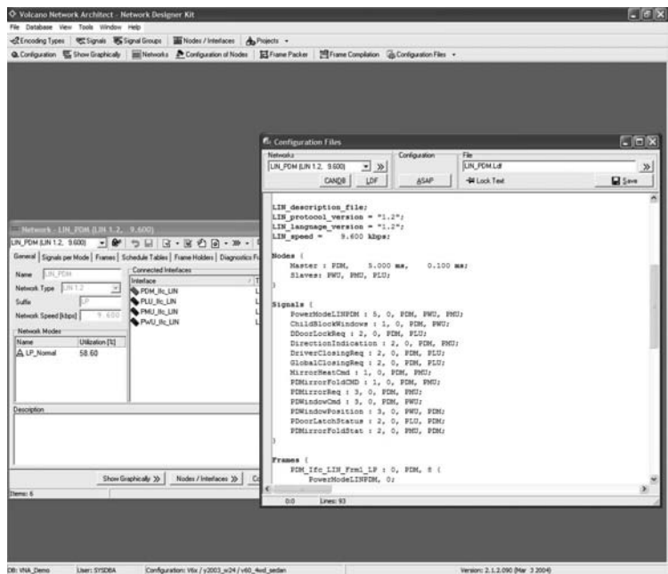
FIGURE 17.9 LDF file generation.
