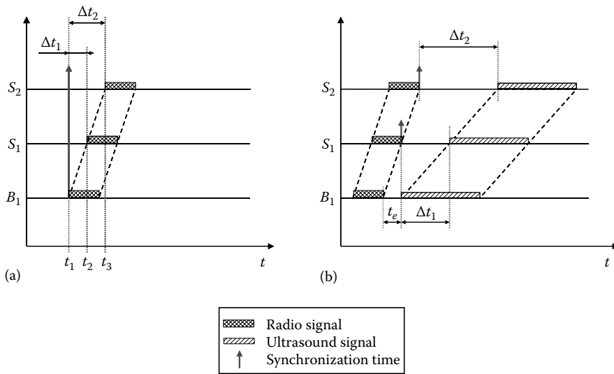
FIGURE 6.2 Distance estimation with time of arrival (ToA) at (a) global synchronization time stamp or (b) local synchronization time stamp.
