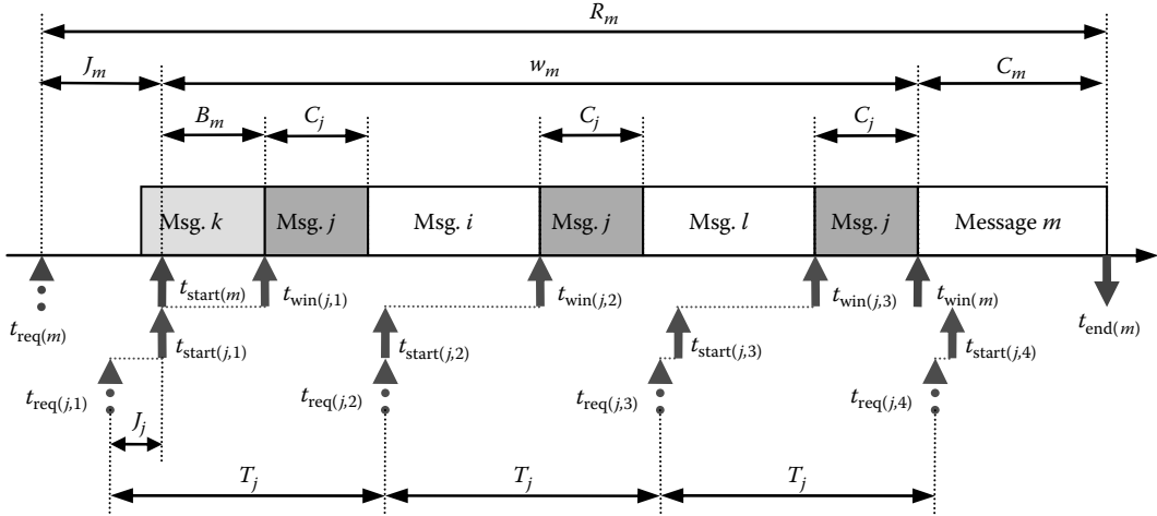
FIGURE 15.7 Blocking time and interference.
