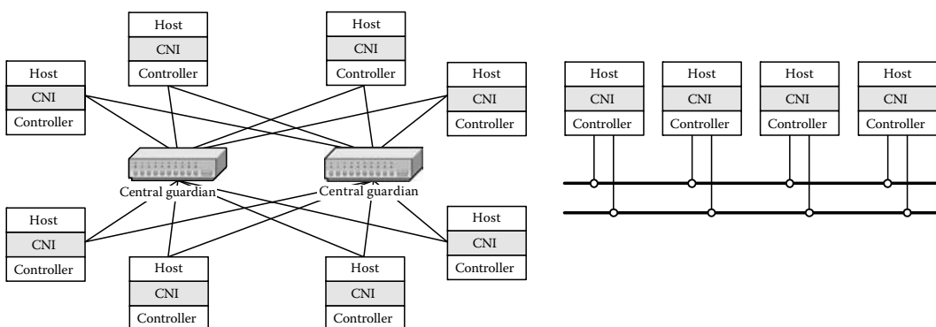
FIGURE 14.1 TTP/C network with star topology (left) and bus topology (right).
