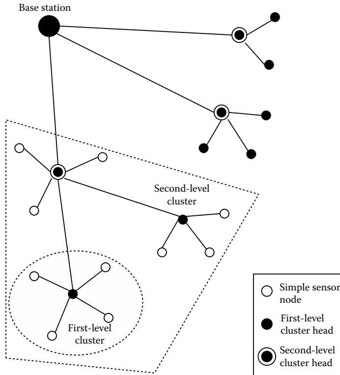
FIGURE 7.4 TEEN and APTEEN hierarchical clustering scheme.
