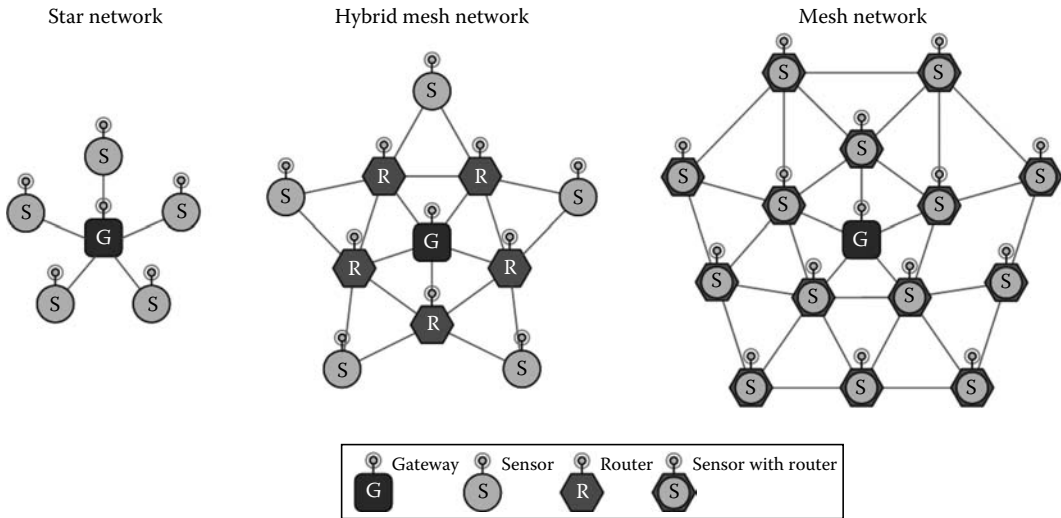
FIGURE 27.2 WSN topologies. (From Aakvaag, N. and Frey, J.-E., ABB Rev. , 2, 40, 2006. With permission.)
