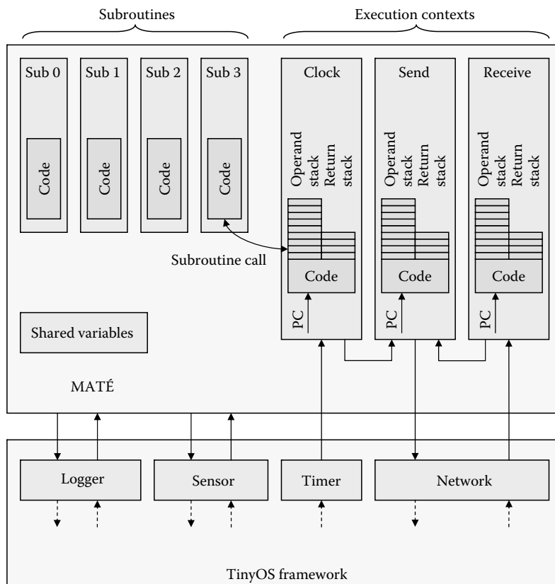
FIGURE 12.8 MATÉ architecture.
