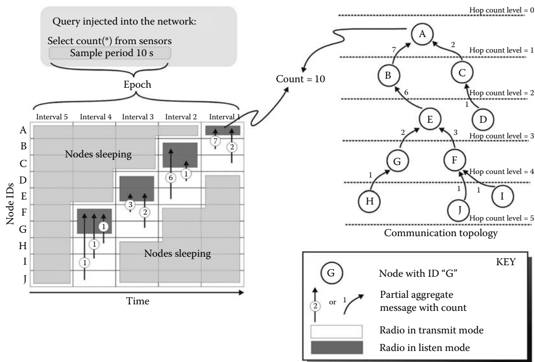
FIGURE 4.11 Aggregation operation using interval-based communication scheduling.
