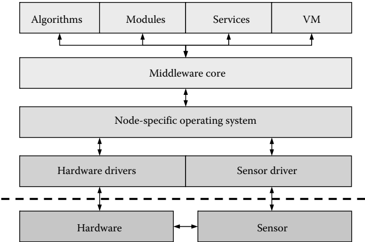
FIGURE 12.12 Structure of a node application.
