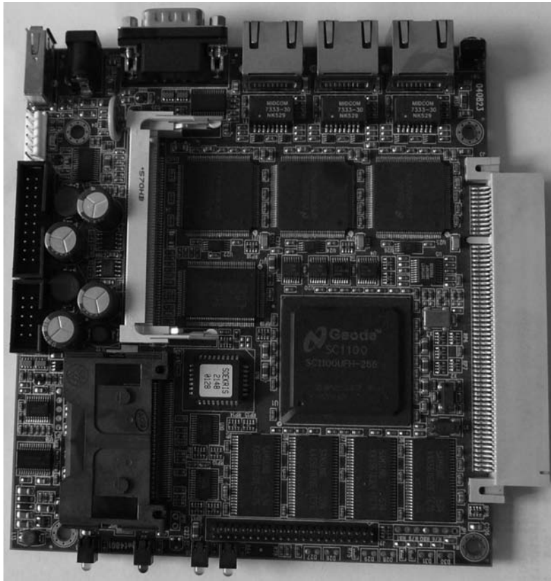
FIGURE 14.4 Time-triggered ethernet node based on Soekris 4801 in the software-based implementation.
