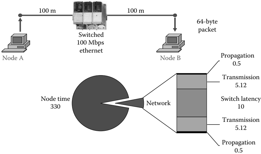
FIGURE 23.15 Illustration of node delay contribution to total delay in a typical two-node Ethernet network (pictured above). Time given in microseconds.
