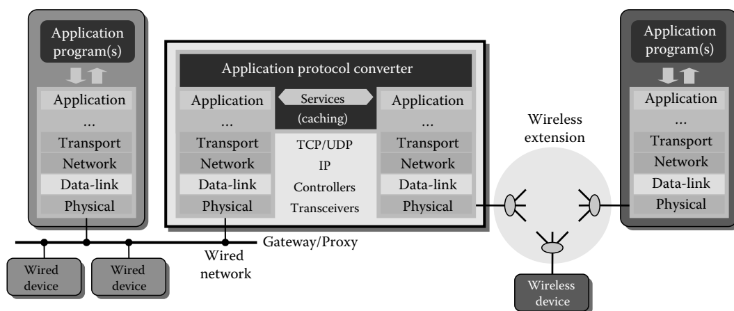
FIGURE 26.4 Interconnection of networks via a gateway.
