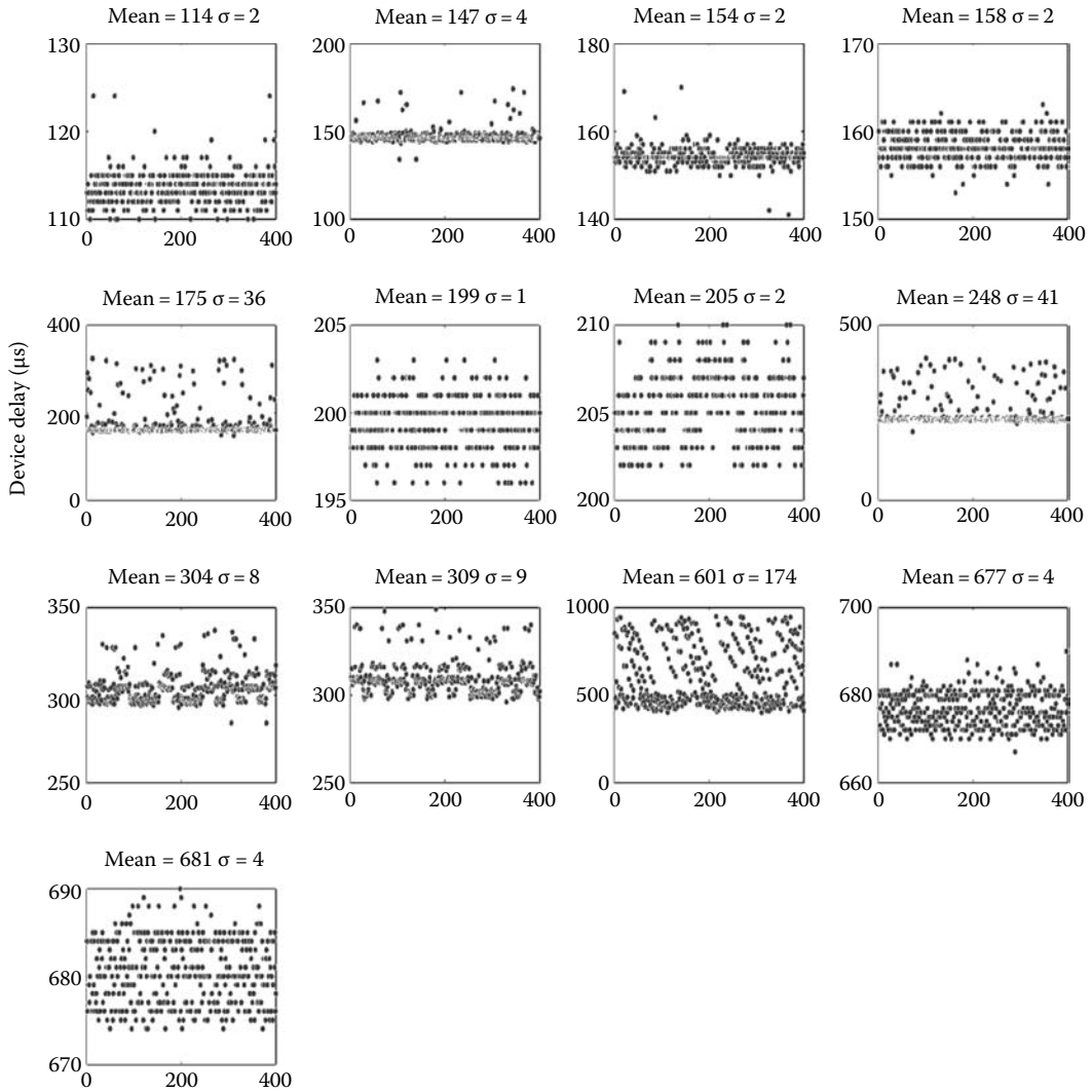
FIGURE 23.2 Device delays for DeviceNet devices in a request–response setup as described in Section 23.2.2.1. Delays are measured with only source and destination node communicating on the network and thus focus only on device delay jitter as described in Section 23.2.2. The stratification of delay times seen in some nodes is due to the fact that the smallest time that can be recorded is 1 μs.
