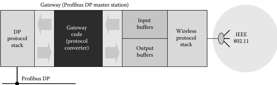
FIGURE 26.5 Gateway for Profibus DP with proxy functionality.
