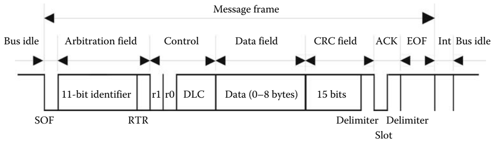
FIGURE 23.7 Message frame format of DeviceNet (standard CAN format).
