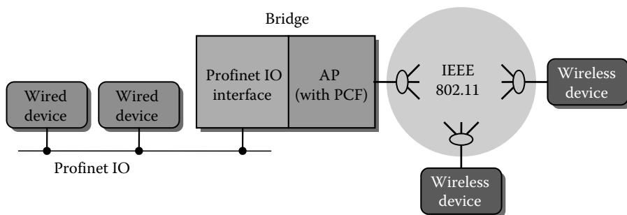
FIGURE 26.8 Extension of Profinet IO via a bridge.
