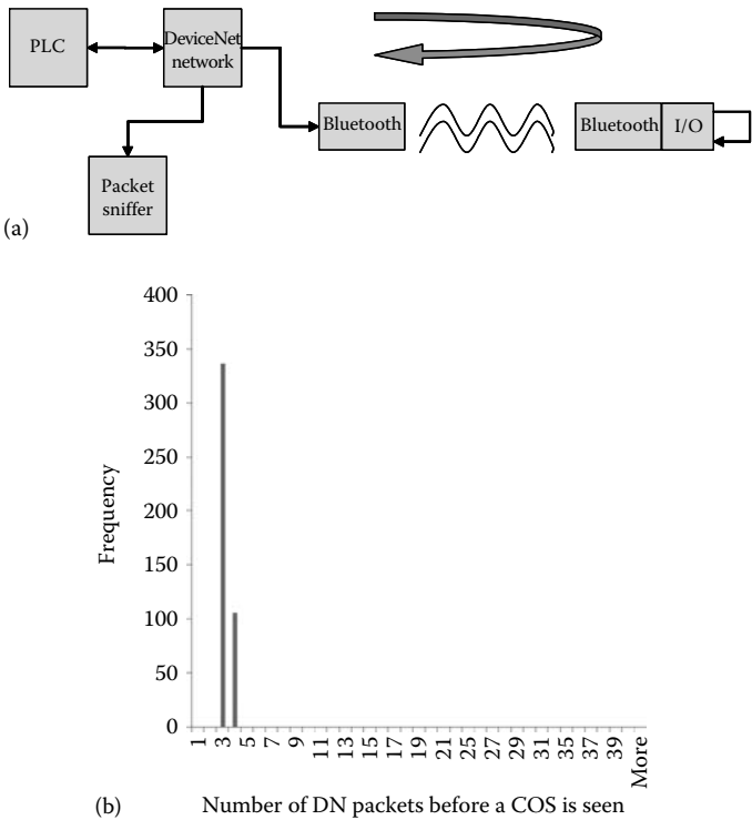
FIGURE 23.14 Experimental characterization of determinism in a Bluetooth system. (a) Bluetooth determinism performance experimental setup, (b) baseline result with minimal channel noise and near ideal distance between nodes, (c) distance test (10 m) is inset expanded view of nondeterminism, and (d) interference test, with nondeterminism highlighted.
