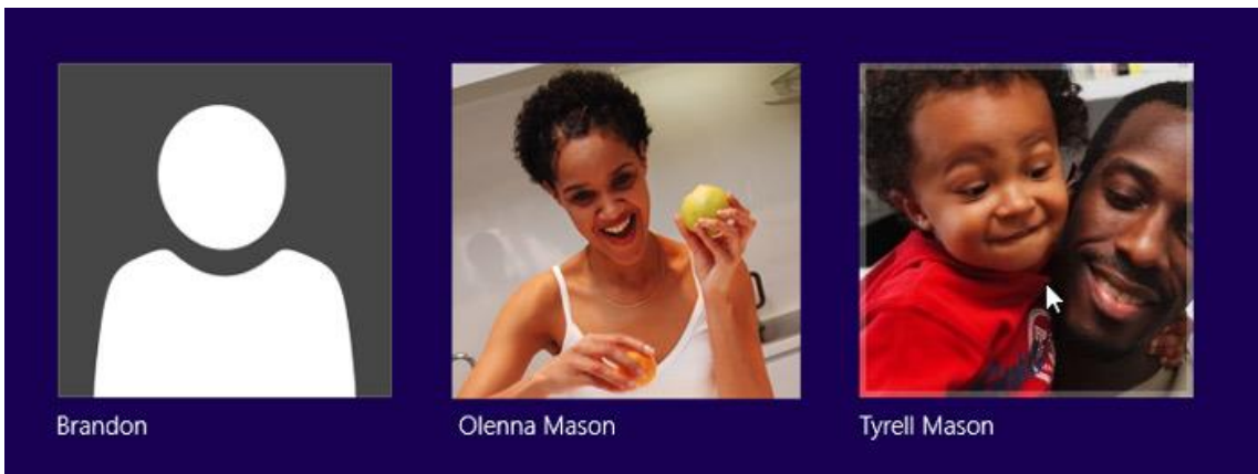
Gambar 13.60 Tools
