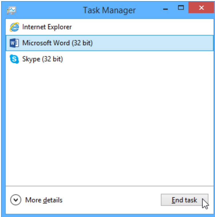
Gambar 13.74 Task Manager
