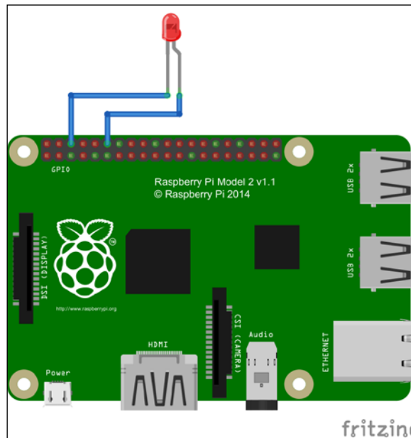
Figure 25 : Blinking an LED using Raspberry Pi 2
