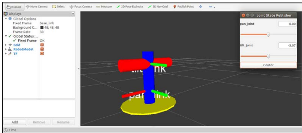
Figure 6 : Joint level of pan and tilt mechanism
