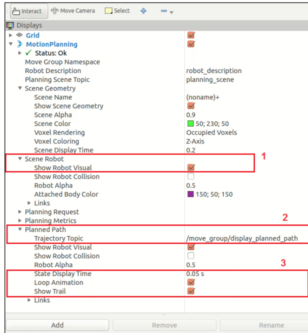
Figure 14 : Settings of the MotionPlanning plugin on RViz
