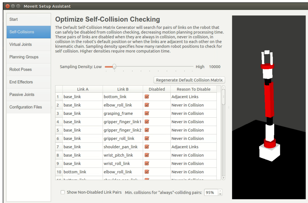
Figure 6 : Regenerating the Self-Collision matrix
