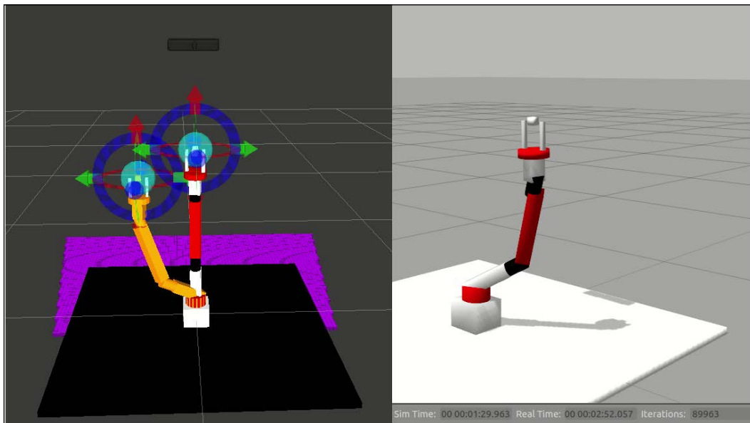
Figure 16 : Gazebo trajectory controllers executing the trajectory from MoveIt!
