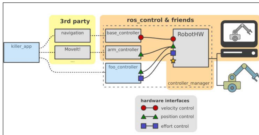
Figure 6 : Interacting ROS controllers with Gazebo
