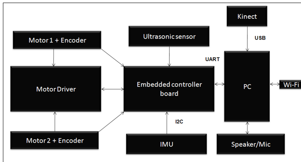
Figure 2: Block diagram of Chefbot
