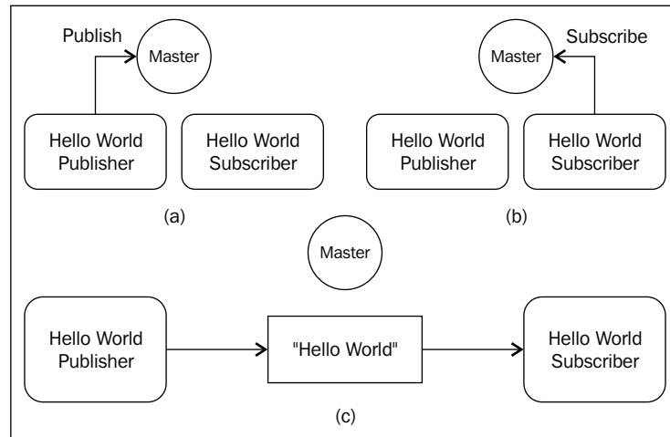
Figure 8: Communication between ROS Master and Hello World publisher and subscriber
