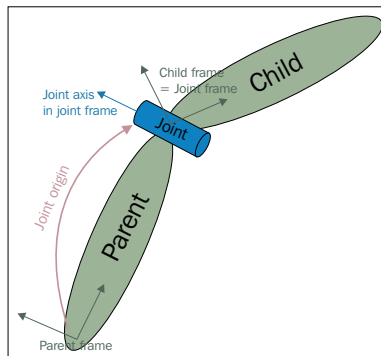
Figure 2 : Visualization of a URDF joint
