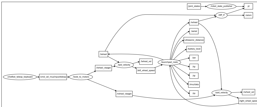
Figure 9: Interconnection of nodes in Chefbot
