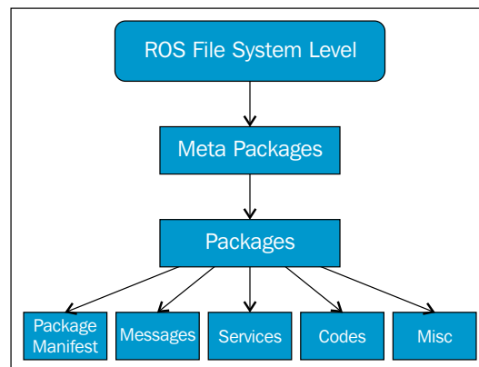
Figure 1 : ROS File system level
