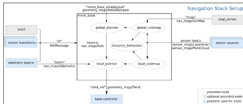
Figure 19 : Navigation stack setup diagram
