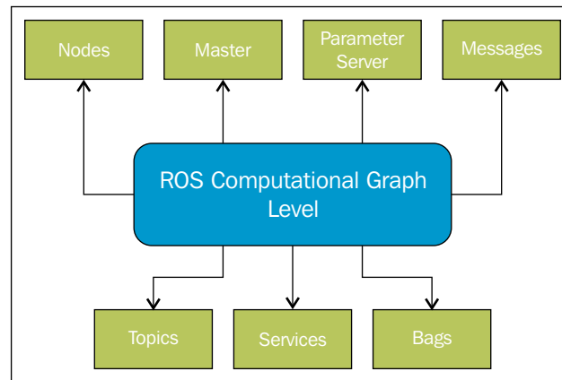
Figure 6 : Structure of the ROS Graph layer
