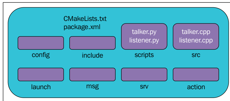
Figure 3 : Structure of a typical ROS package
