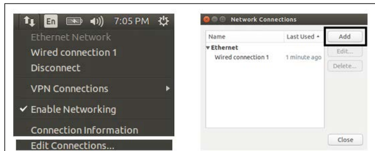
Figure 20 : Configuring a network connection in Ubuntu
