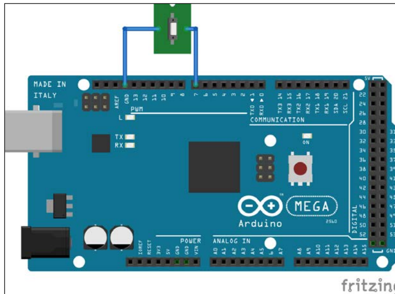
Figure 10 : Interfacing the push button to Arduino
