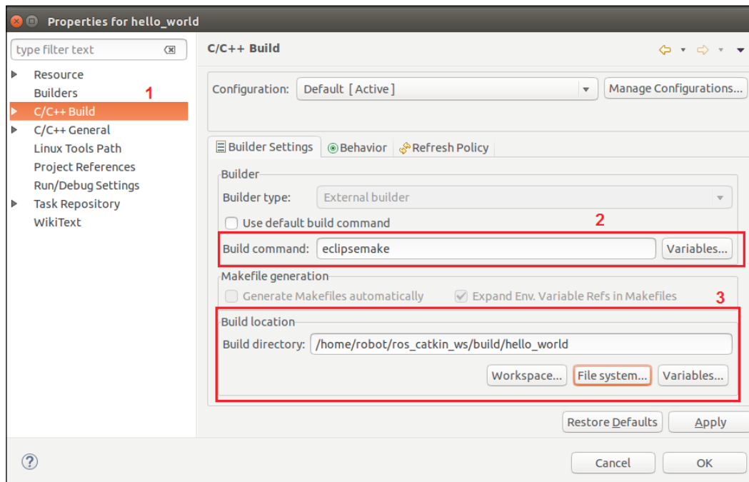
Figure 8: Eclipse build settings for ROS
