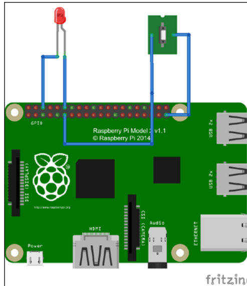
Figure 26 : LED + button in Raspberry Pi 2
