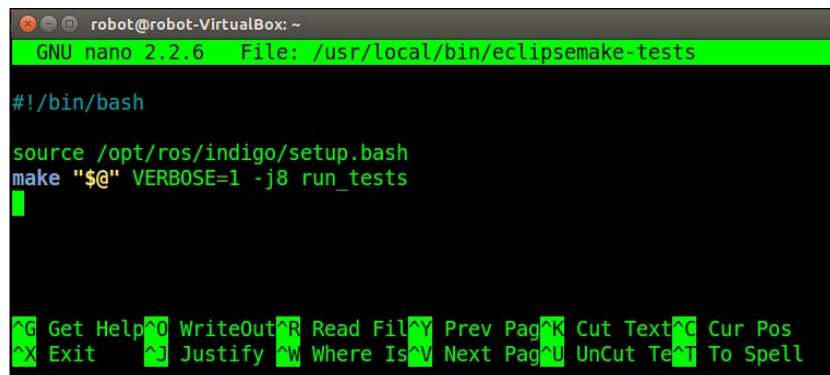
Figure 5: Script to source the ROS environment and running test
