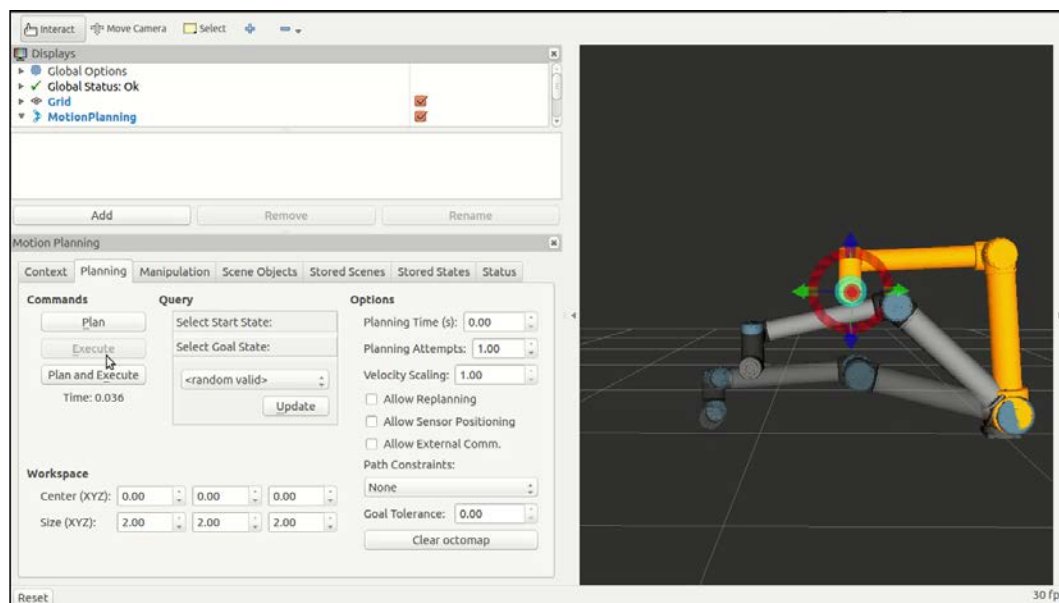
Figure 9: Motion planning in UR-10 model in RViz
