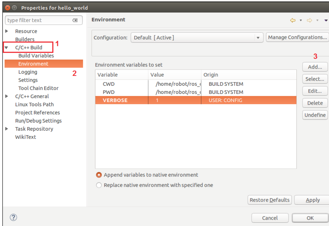
Figure 9: Setting VERBOSE in ROS project properties
