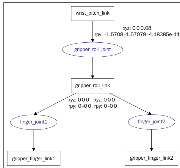
Figure 9 : Graph of the end effector section of seven dof arm robot
