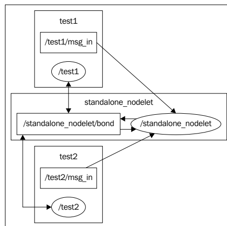
Figure 10: A two-node instance of a nodelet
