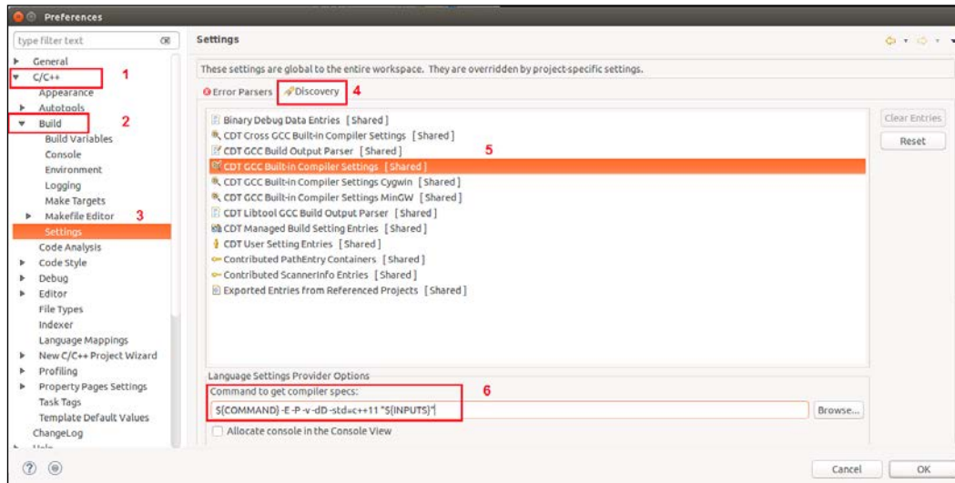
Figure 3: Eclipse Compiler settings
