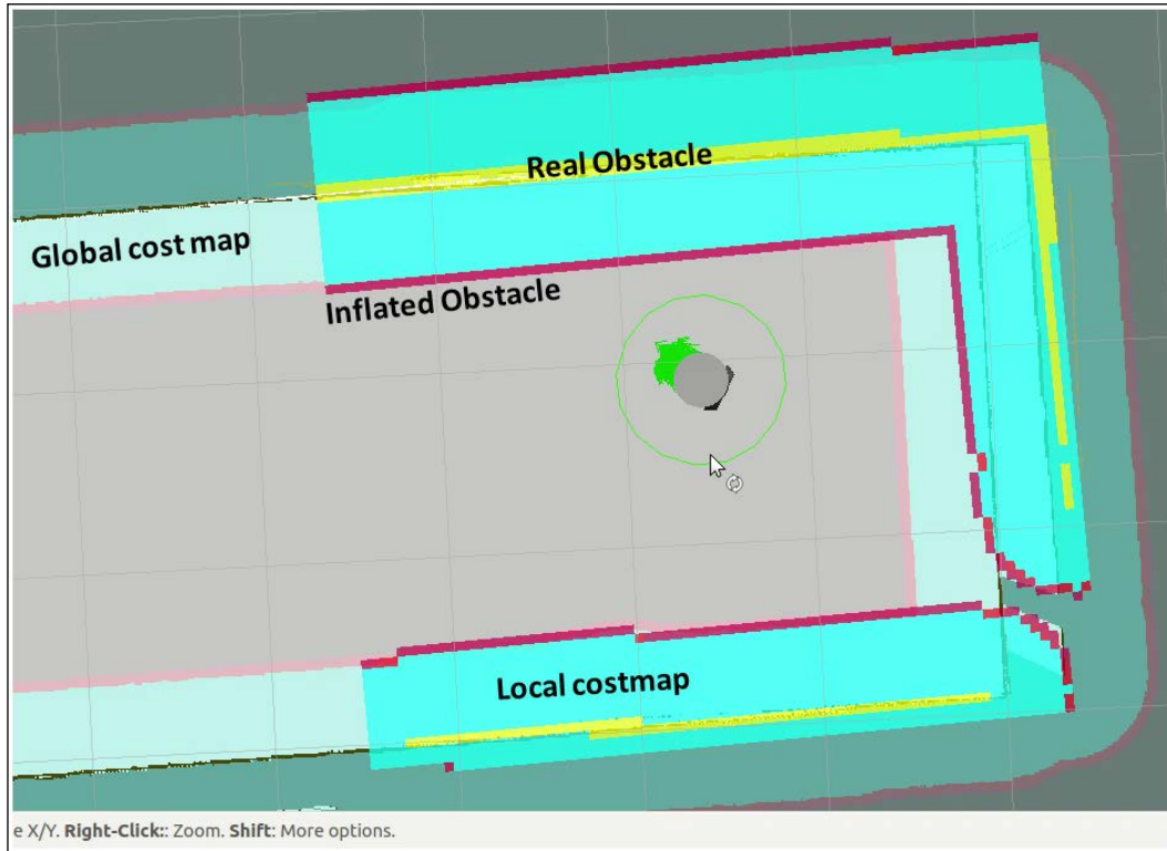
Figure 18 : Visualizing global and local map, and real and inflated obstacle in RViz
