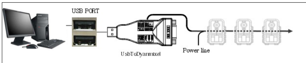
Figure 14 : Dynamixel Servos connected to PC using USB To Dynamixel controller.
