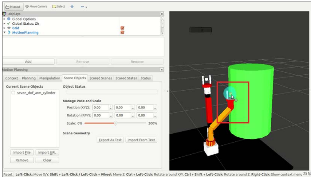
Figure 5: Visualizing collided link.
