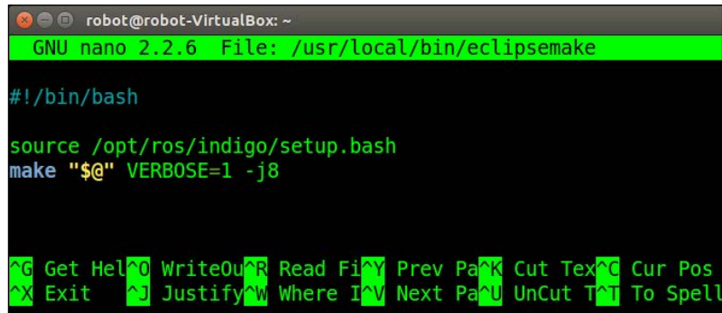
Figure 4: Script to source the ROS environment
