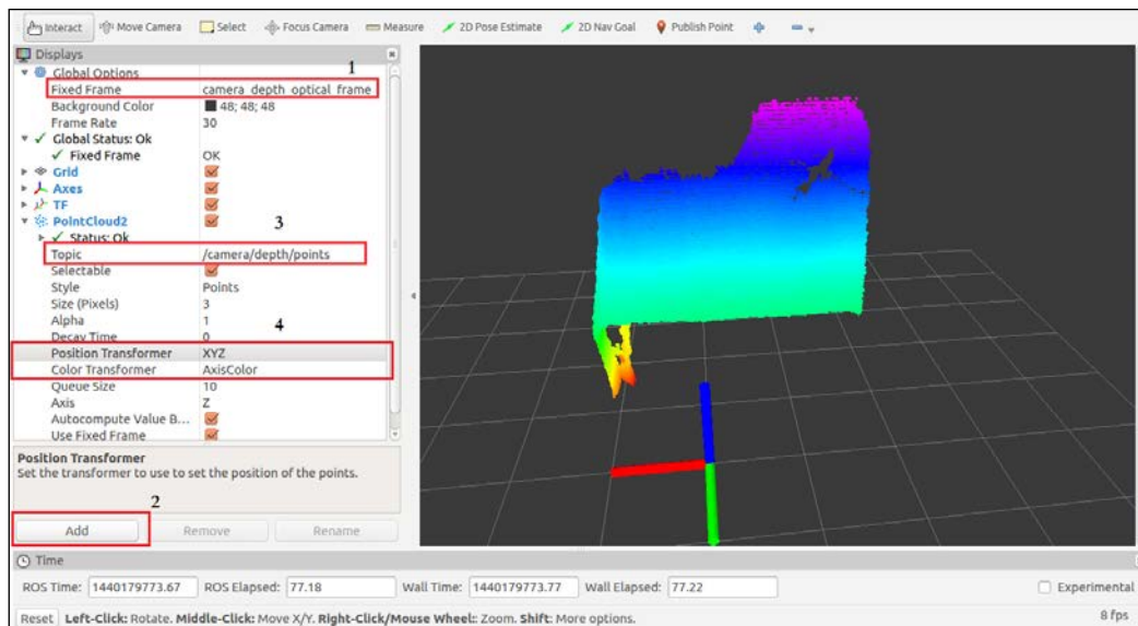
Figure 8: Unregistered point cloud view in RViz
