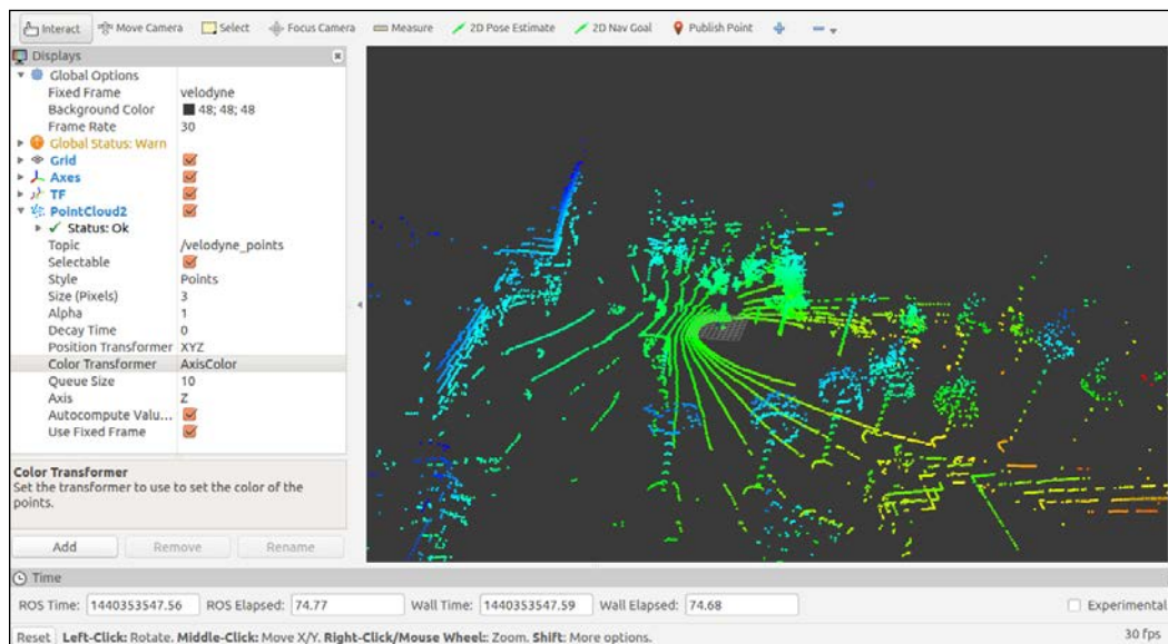
Figure 18: Velodyne point cloud view in RViz
