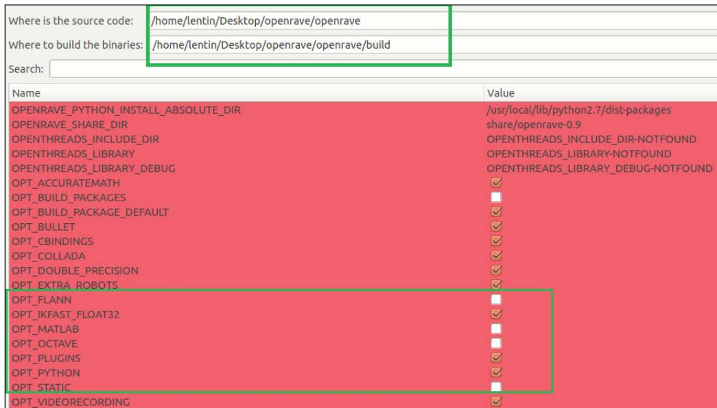
Figure 15: Configuring OpenRave with cmake-gui
