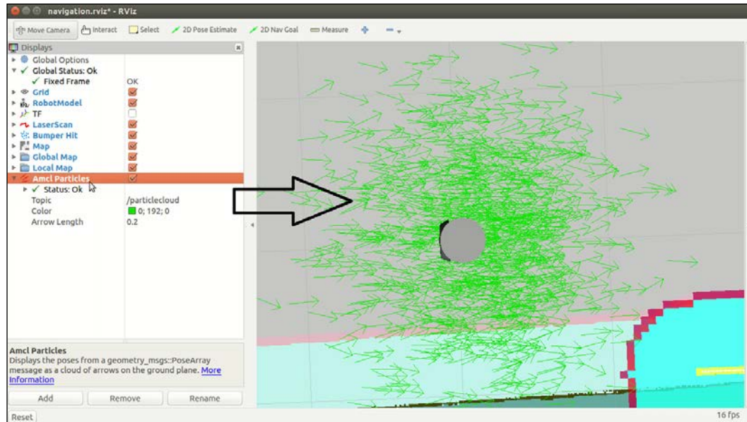
Figure 14: Visualizing AMCL particles
