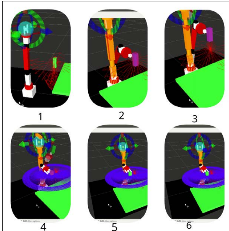
Figure 12 : Pick and place sequences using MoveIt!.
