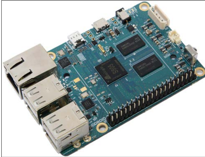
Figure 17 : Odroid-C1 board
