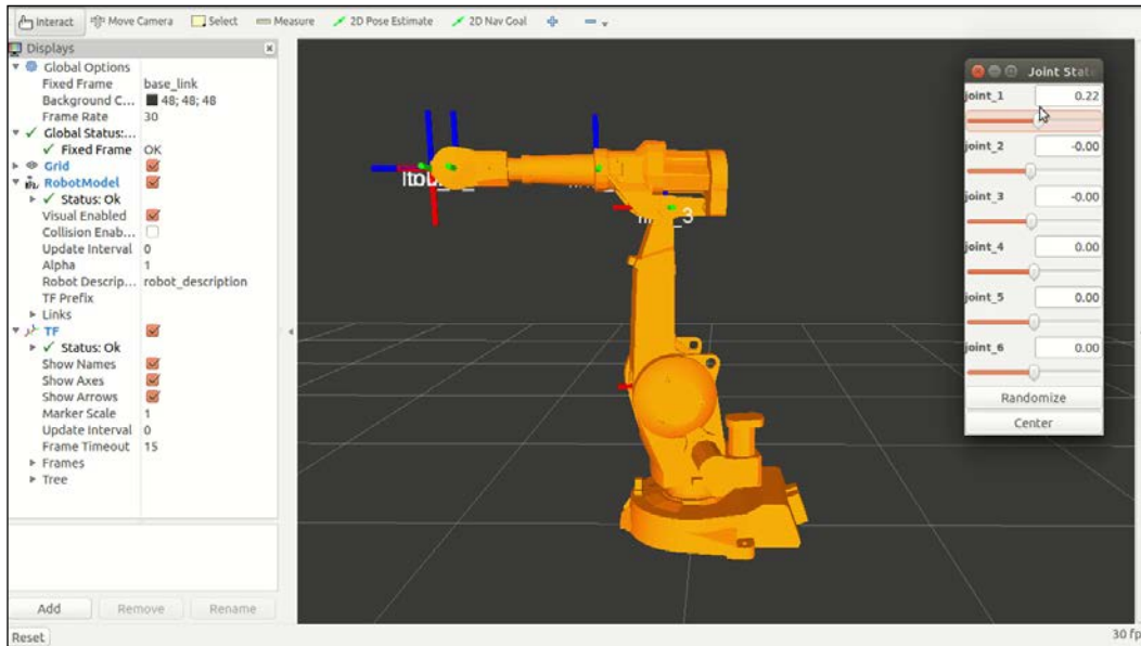
Figure 14: ABB IRB 2400 with joint state publisher on RViz
