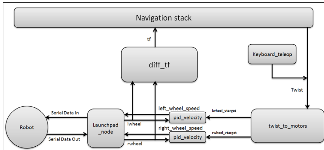
Figure 5: Interconnection of each nodes in Chefbot
