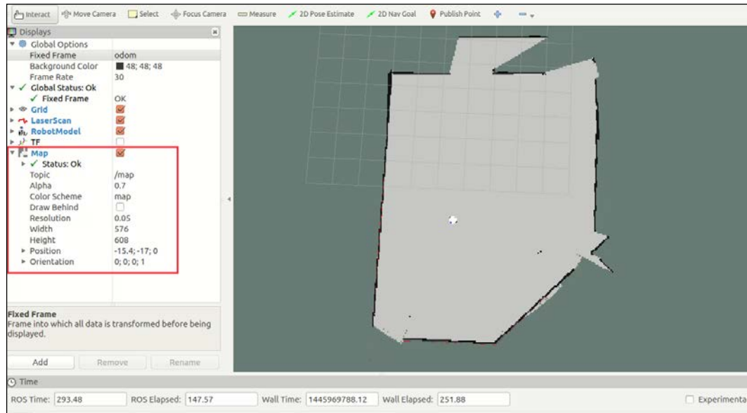
Figure 22 : Completed map of the room in RViz
