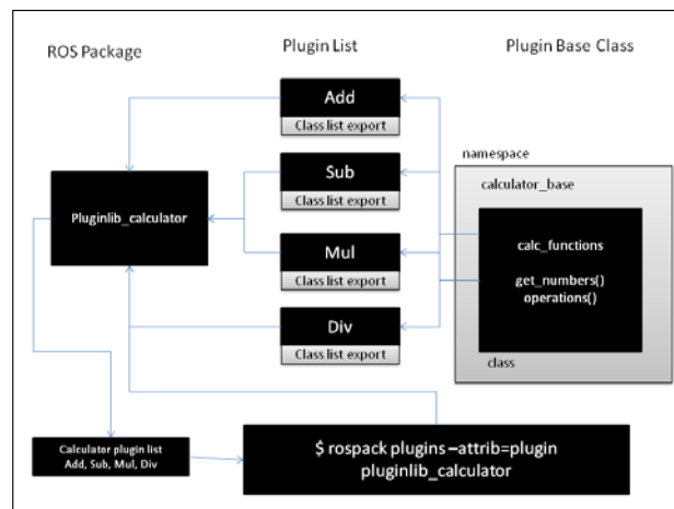
Figure 1: Organization of plugins in the calculator application
