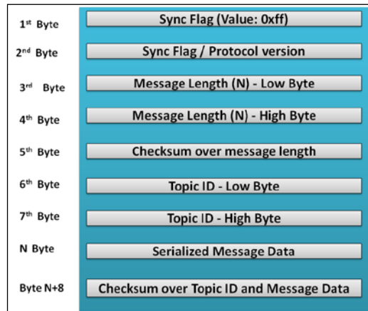
Figure 2 : roserial packet representation
