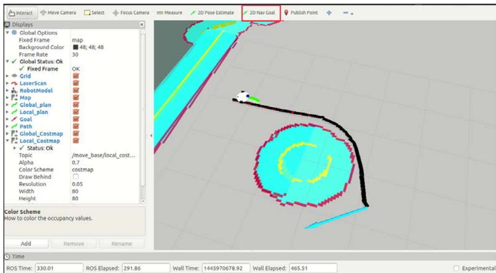
Figure 26 : Autonomous navigation using AMCL and the map
