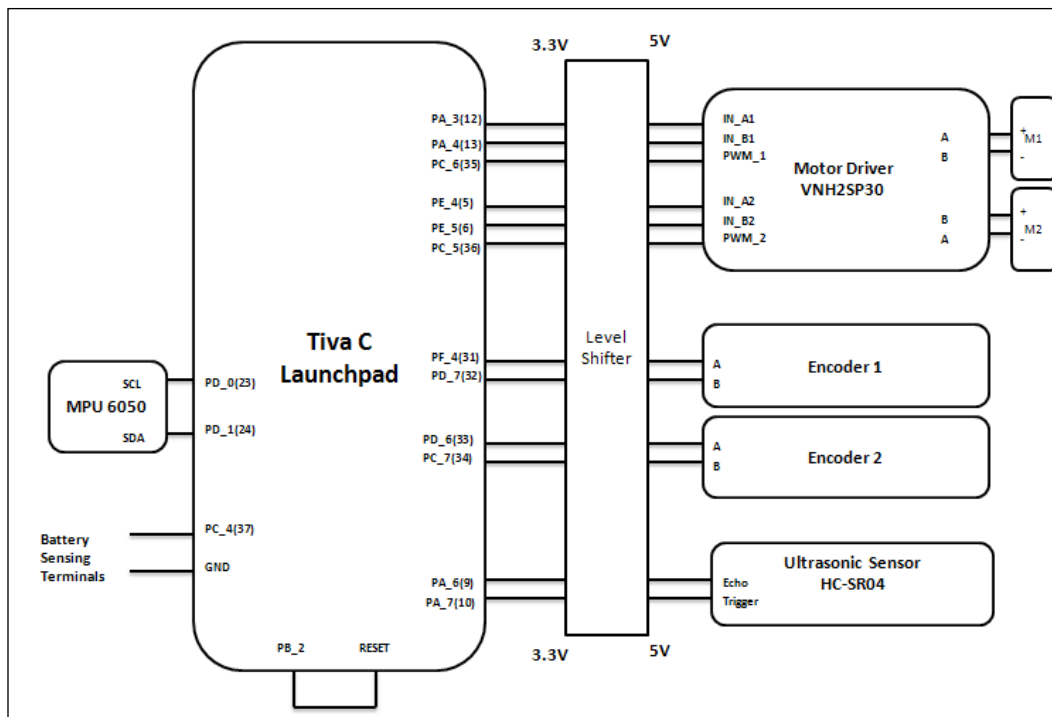
Figure 3: Connection diagram of Chefbot
