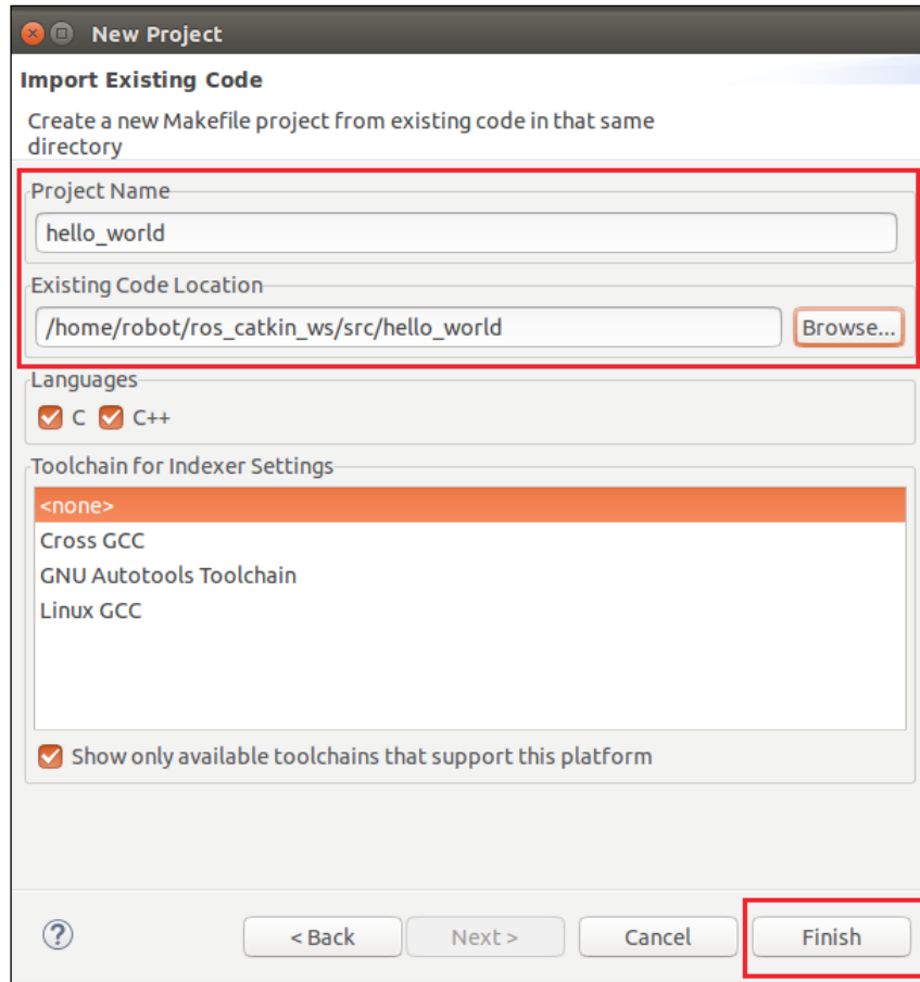
Figure 7: Giving project and location
