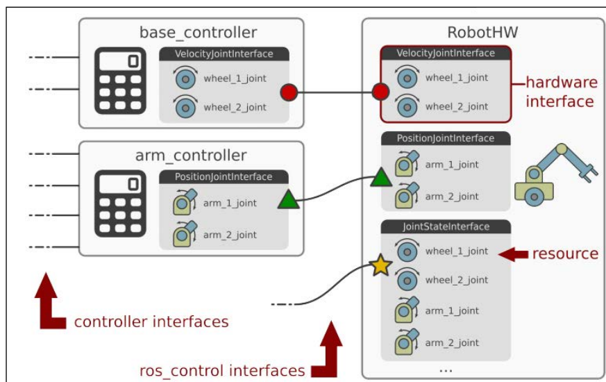
Figure 7 : Illustration of ROS controllers and hardware interfaces
