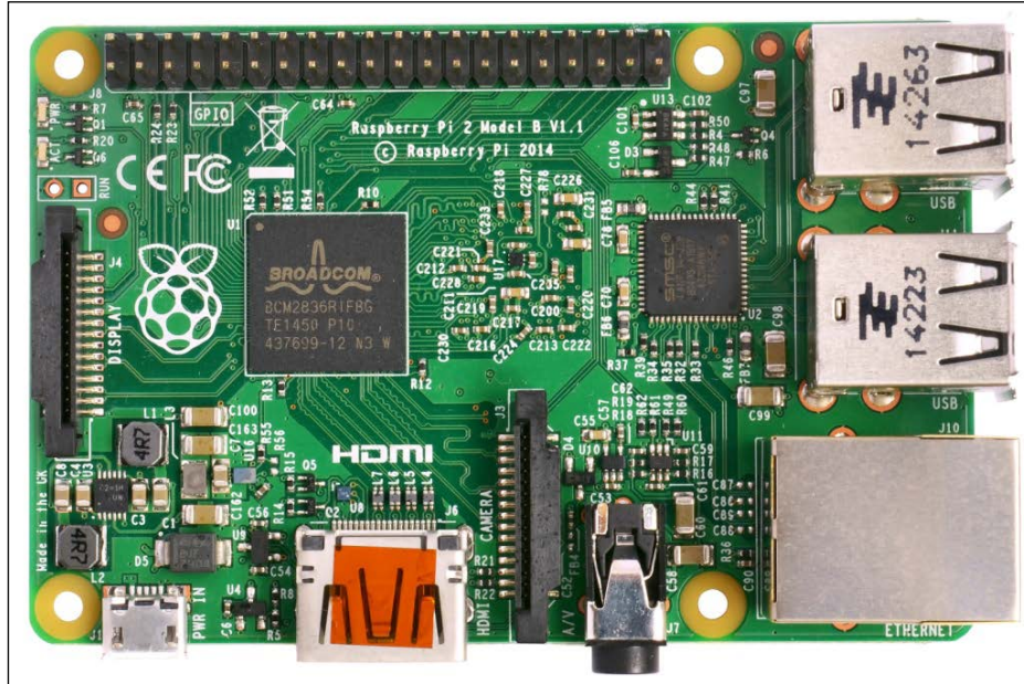
Figure 18 : The Raspberry Pi 2 board
