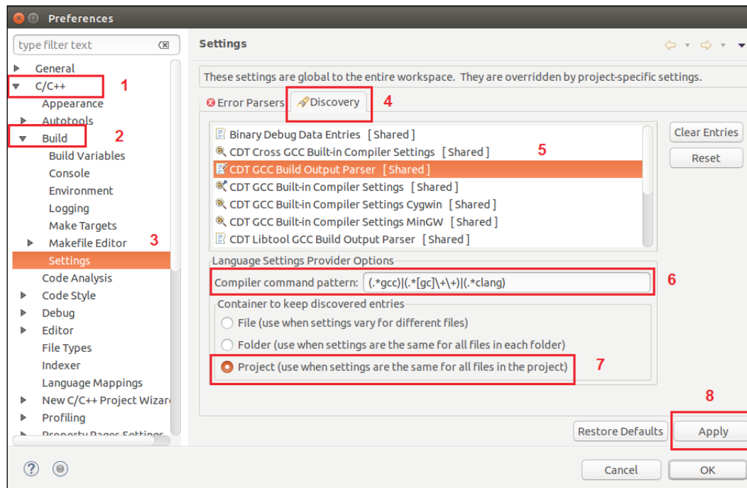
Figure 2: Settings inside Eclipse Preferences
