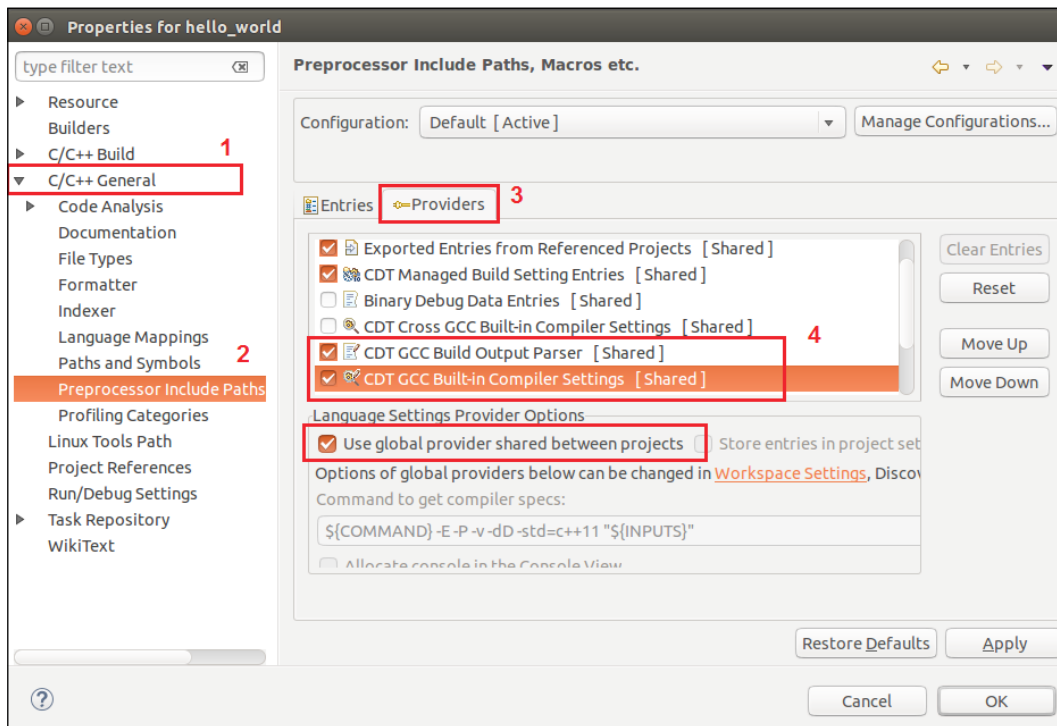
Figure 11: Setting Pre-processor in the project properties
