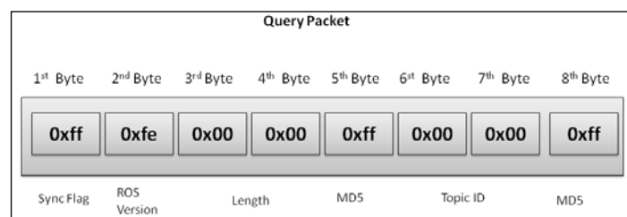
Figure 7 : Structure of Query Packet
