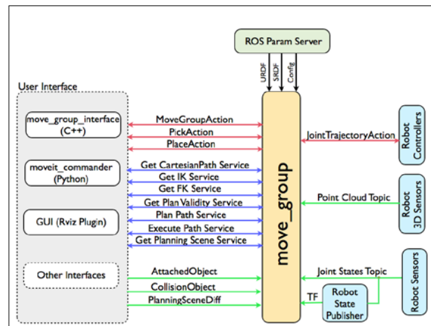
Figure 1: MoveIt! architecture diagram
