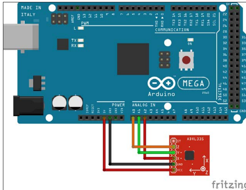
Figure 12 : Interfacing Arduino - ADXL 335
