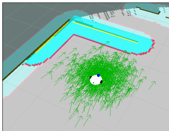
Figure 27 : The AMCL particle cloud
