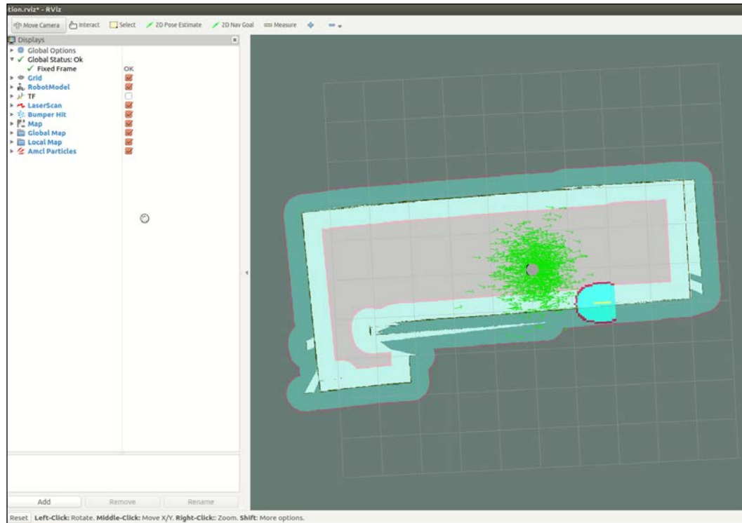
Figure 12: Robot autonomous navigation using AMCL
