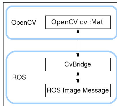
Figure 5 : Converting images using CvBridge
