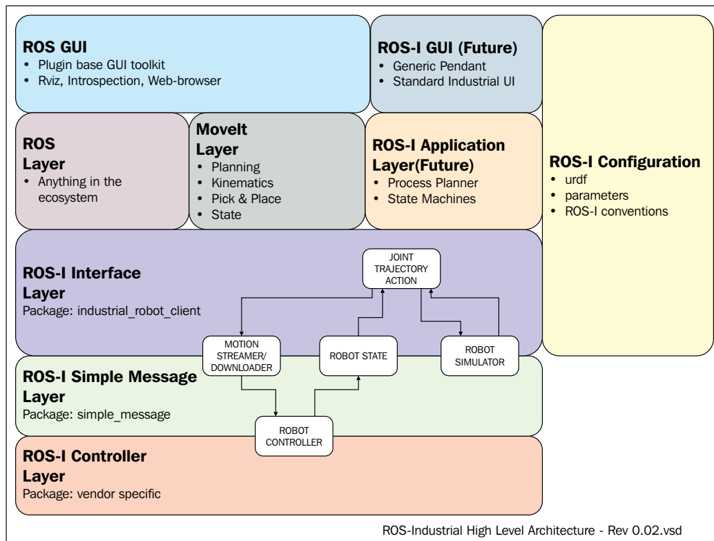
Figure 2: The block diagram of ROS-Industrial
