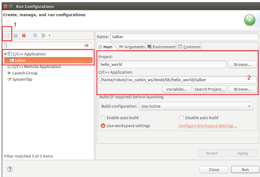
Figure 12: Creating the launcher for the talker node
