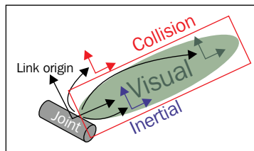
Figure 1 : Visualization of a URDF link
