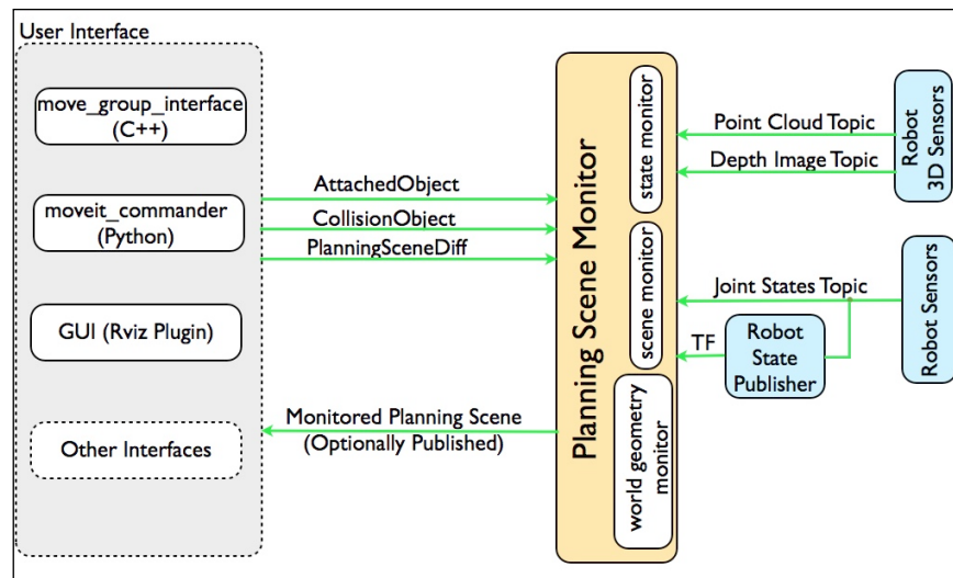
Figure 3 : MoveIt! planning scene overview diagram
