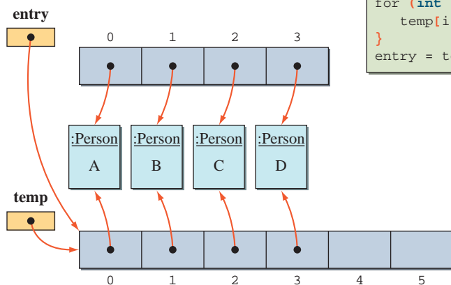
Figure 10.16 How a new array that is 150 percent of the original array is created. The size of the original array is 4.
