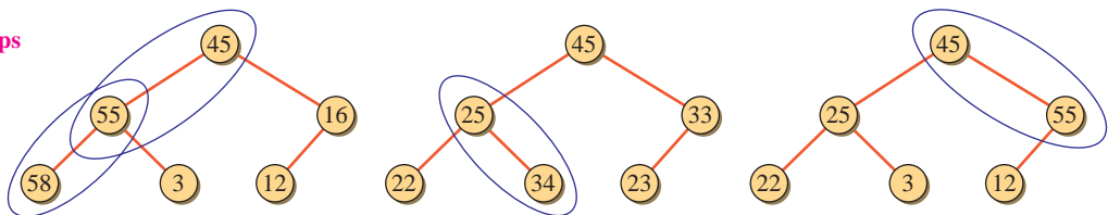
Figure 11.10 Sample heaps and nonheaps that violate the value relationship constraint. Violations are indicated by blue ellipses.
