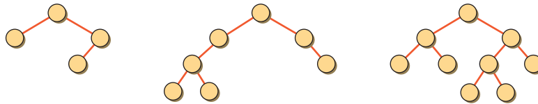
Figure 11.9 Sample heaps and nonheaps that violate the structural constraint.
