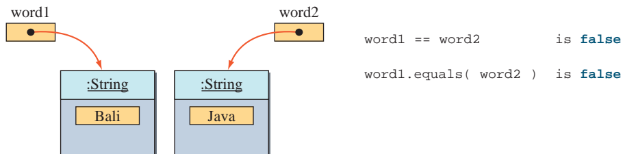
Figure 9.2 The difference between the equality test and the equals method.
