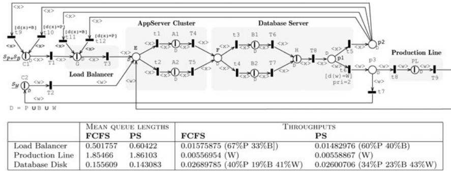
Fig. 3 SWN model for the distributed component-based example; throughputs and average number of customers computed for different queueing policies at the LB.
