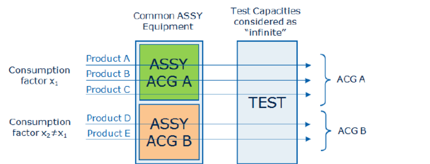
Fig. 1 Example of two Assy-ACGs.
