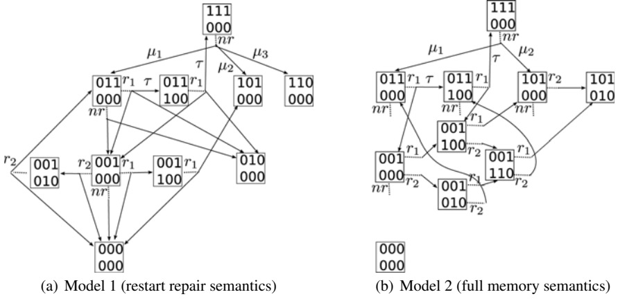
Fig. 1 Excerpt of the CTMDP for different Erlang-2 repair semantics for a parallel system of 3 components ((b) showing especially transitions for repair procedure which differ from (a)). Dashed lines represent decisions and solid lines exponential transitions.
