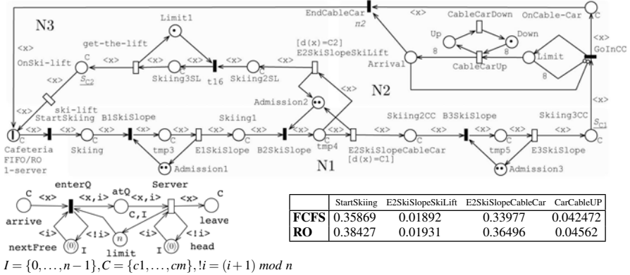
Fig. 1 SWN model for the skiers example (upper fig.); SWN submodel of FCFS policy (lower fig.); Table of the throughputs for RO or FCFS queueing policy at the cafeteria.
