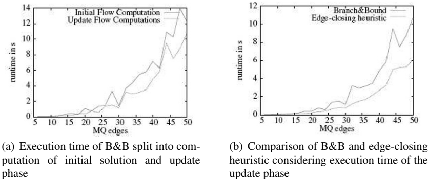
Fig. 1 Execution time comparisons on randomly generated networks with two models, averaged over 30 runs.
