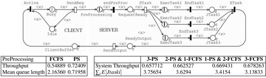
Fig. 2 SWN model for the Client-Server example; Performance indices of the Client-Server model varying the queueing policy: (left) in PreProcessing with hyper exponential service time; (right) in the fork/join construct.
