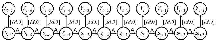
Fig. 2 Architecture of the Historical Consistent Neural Network (HCNN)
