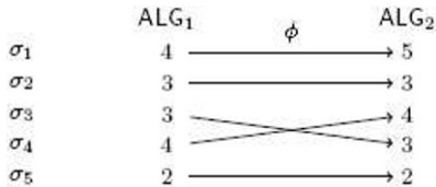
Fig. 3 Illustration of the idea of bijective analysis for the example from Figure 1: ALG_1 is at least as good as ALG_2 along the bijective mapping \phi .
