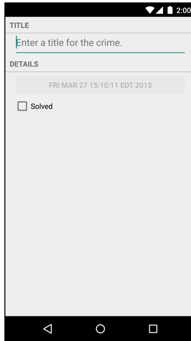
Figure 8.1 CriminalIntent, episode 2
