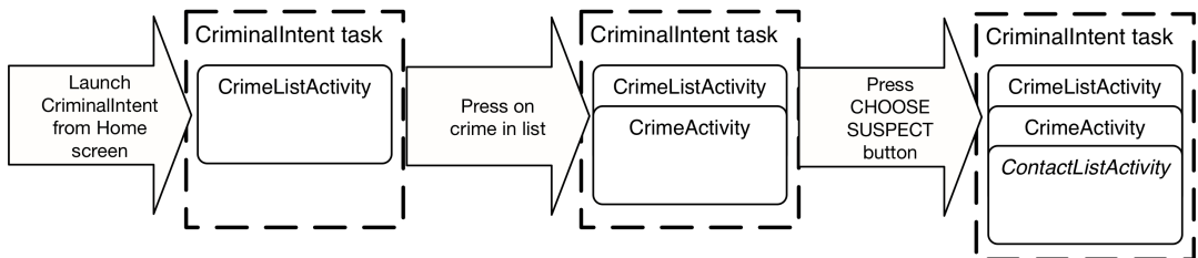
Figure 22.5 CriminalIntent task
