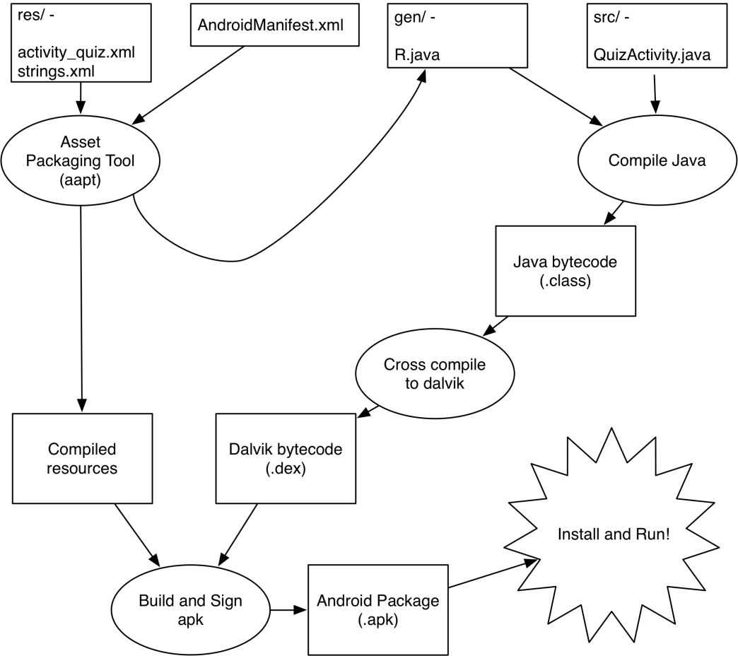
Figure 1.19 Building GeoQuiz
