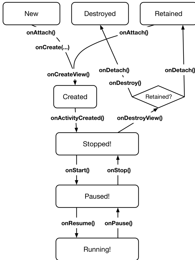
Figure 19.4 Fragment lifecycle
