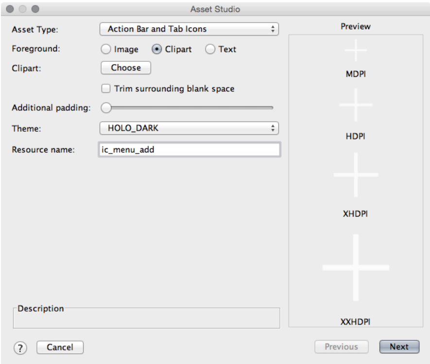
Figure 13.6 Asset Studio
