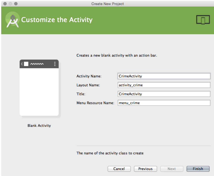
Figure 7.8 Configuring CrimeActivity
