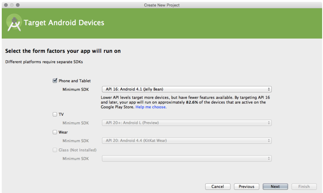
Figure 6.1 Remember me?
