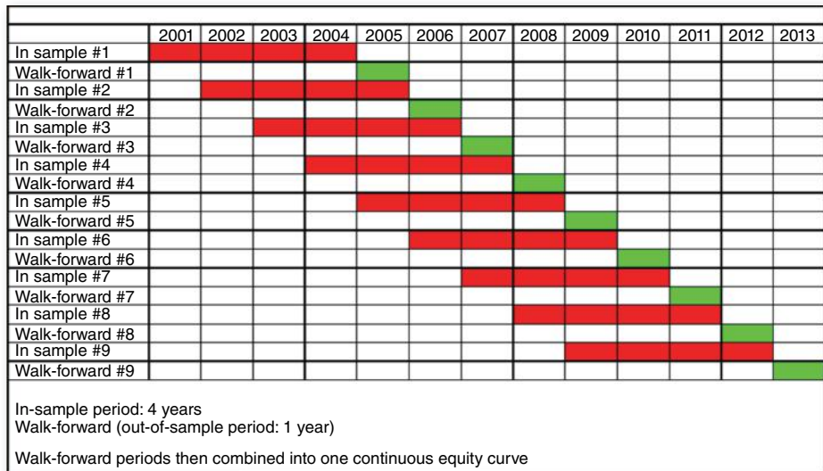
FIGURE 5.5 Walk-Forward Analysis
