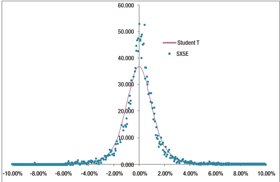
Figure 3-16. Method of moments fit for the SX5E Index (Euro Stoxx 50) to a Student's-t distribution
