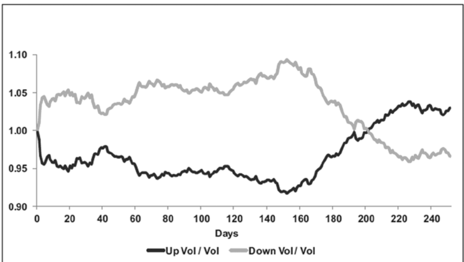
Figure 3-31. Term structure of “up” and “down” volatility for the dynamic portfolio allocation multi-asset proprietary index strategy, 2001–2011
