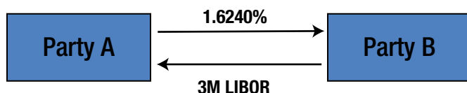
Figure 1-18. A Vanilla Interest Rate Swap.
