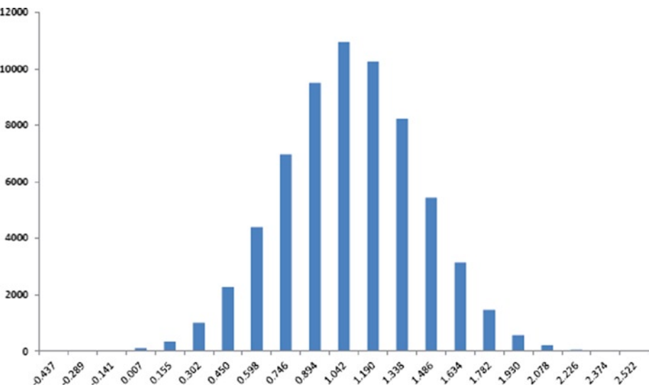
Figure 3-4. Raw histogram
