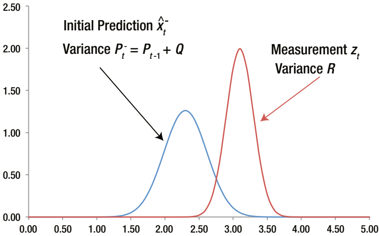
Figure 9-2. Example of the variances of a measurement and an initial prediction to be optimally combined
