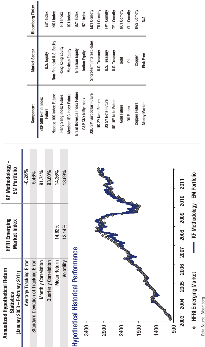
Figure 9-7. Replication of the HFRI Emerging Market Index
