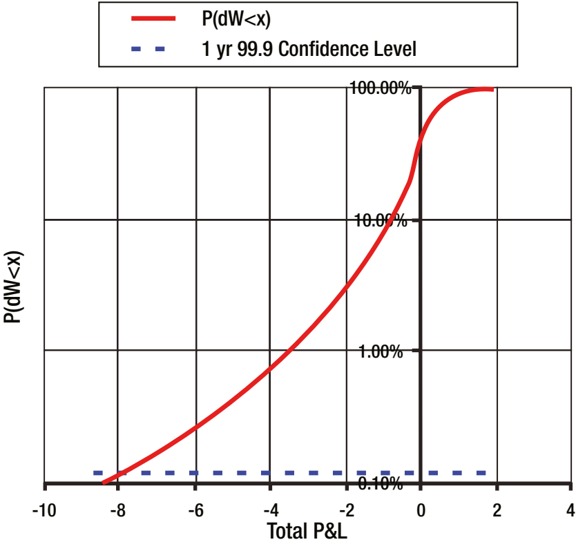
Figure 5-11. Cumulative wealth change distribution F(\Delta W(0, T))
