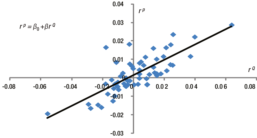
Figure 4-8. Linear regression
