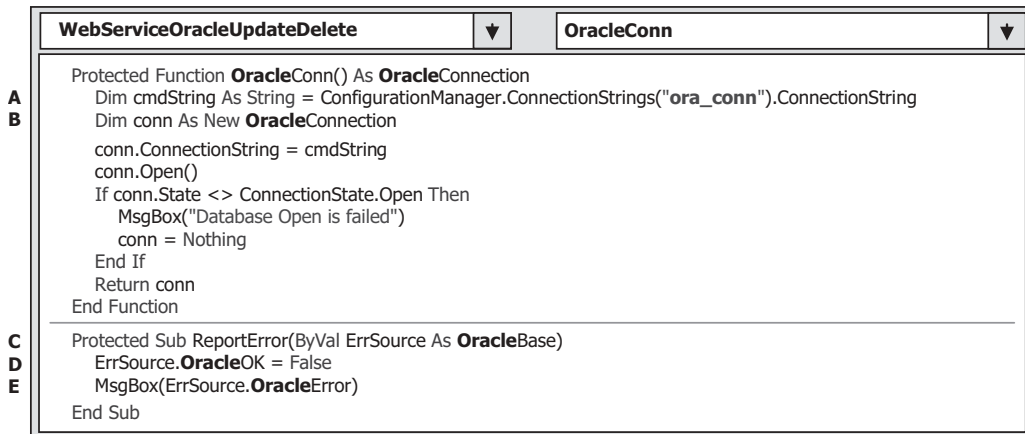
Figure 9.160. Modified subroutines OracleConn() and ReportError().
