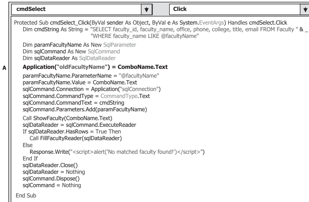
Figure 8.39. The modified Select button's event procedure.
