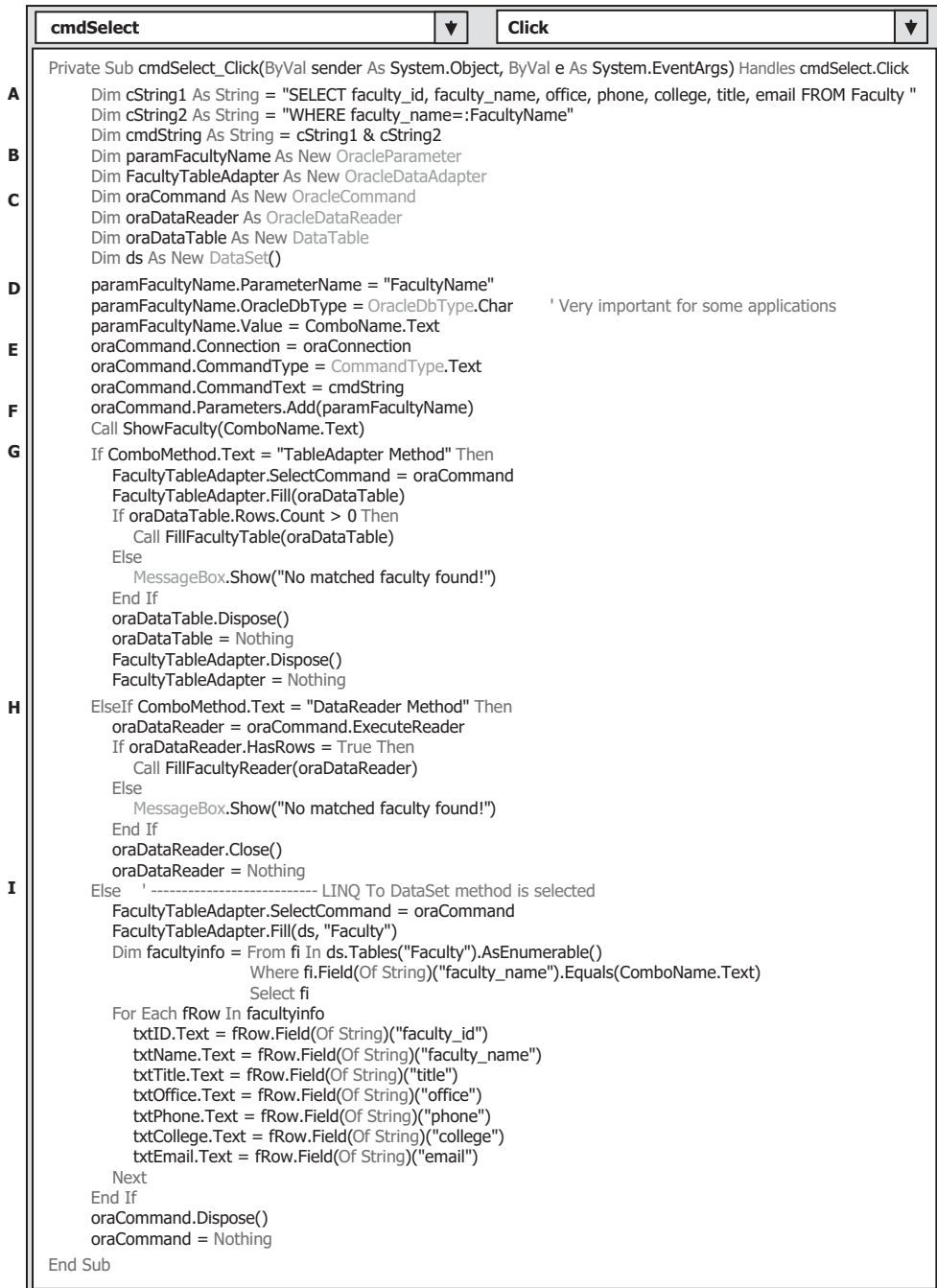
Figure 5.145. The codes for the Select button event procedure.
