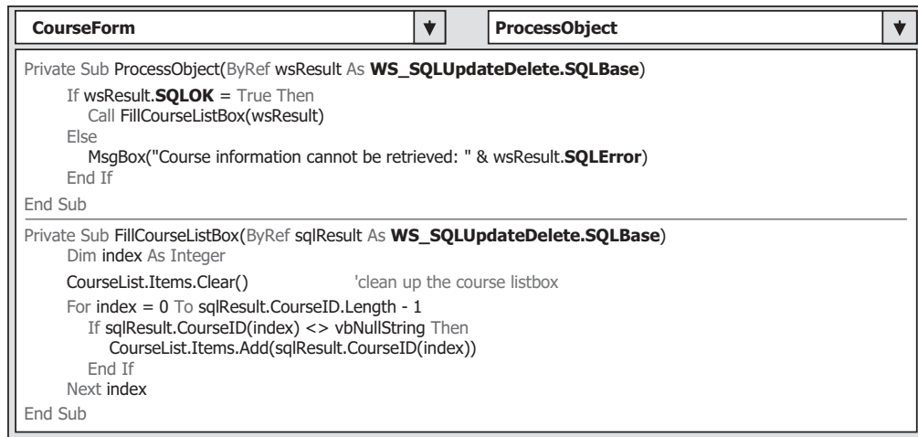
Figure 9.110. The modified subroutines ProcessObject() and FillCourseListBox() .
