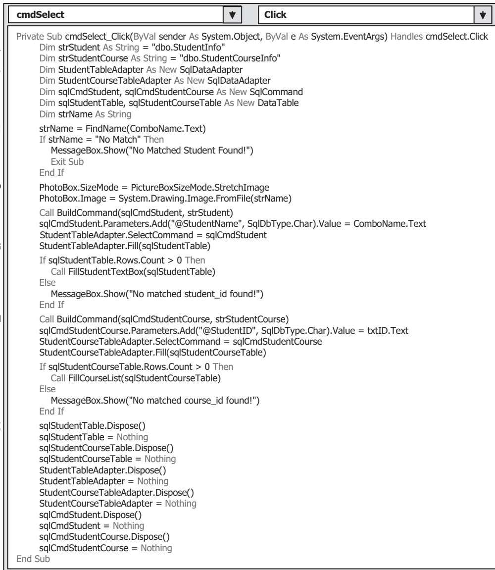
Figure 5.130. The codes for the Select button Click event procedure.
