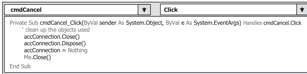
Figure 5.76. The codes for the Cancel button event procedure.
