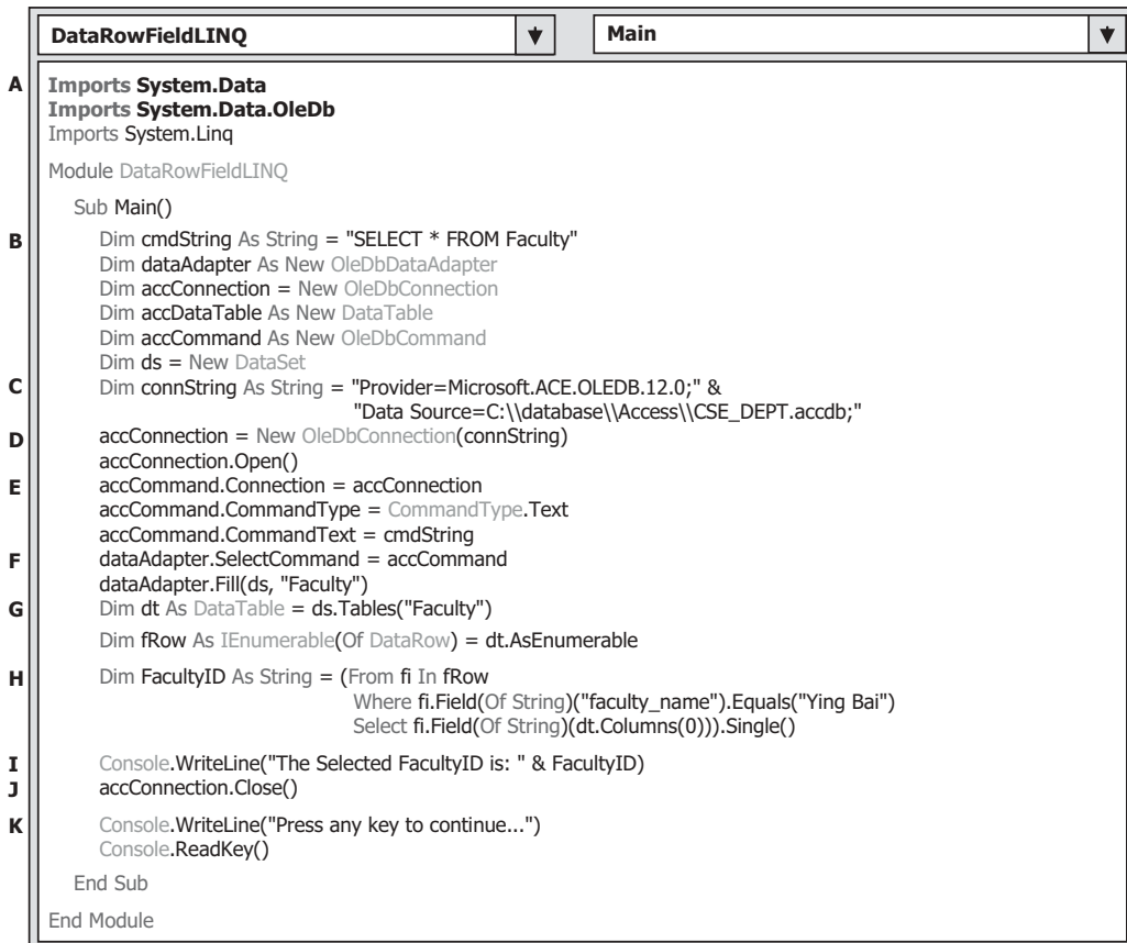
Figure 4.38. The codes for the example project DataRowFieldLINQ.
