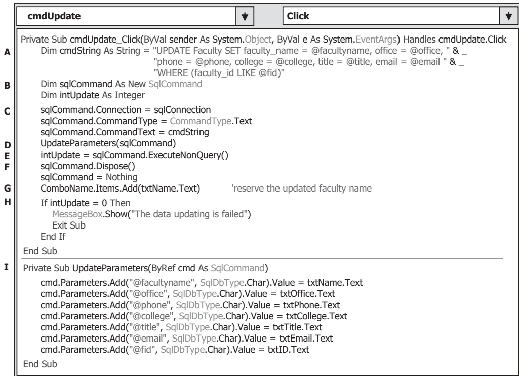
Figure 7.12. The codes for the data updating operation.
