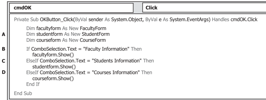
Figure 5.45. The codes for the OK button event procedure.
