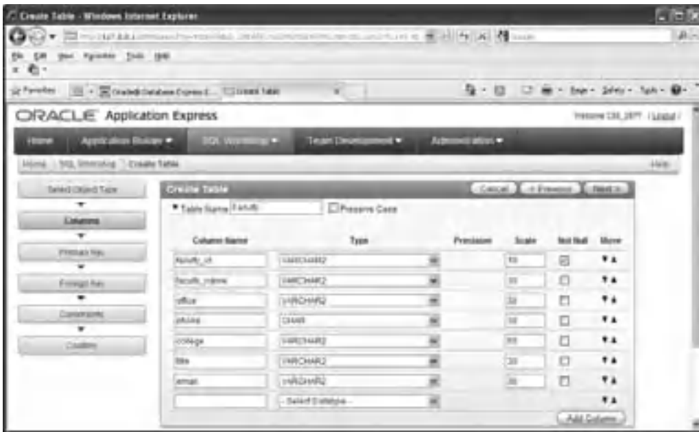
Figure 2.54. The finished design view of the faculty table.
