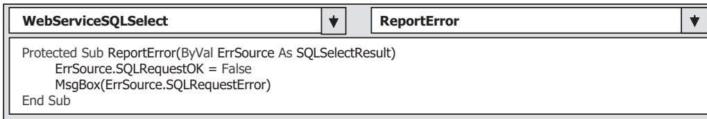
Figure 9.21. The codes for the subroutine ReportError().
