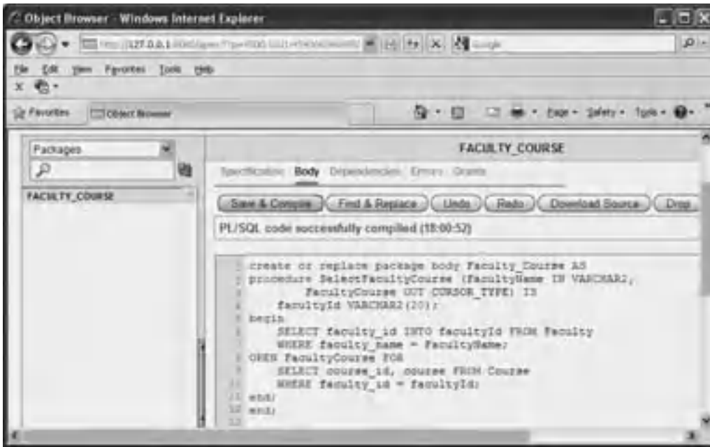
Figure 5.159. The compiled codes for the body part of the package.
