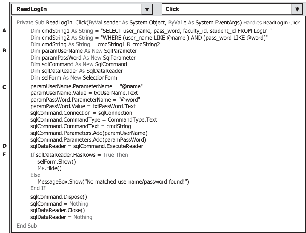
Figure 5.110. The codes for the ReadLogIn button event procedure.
