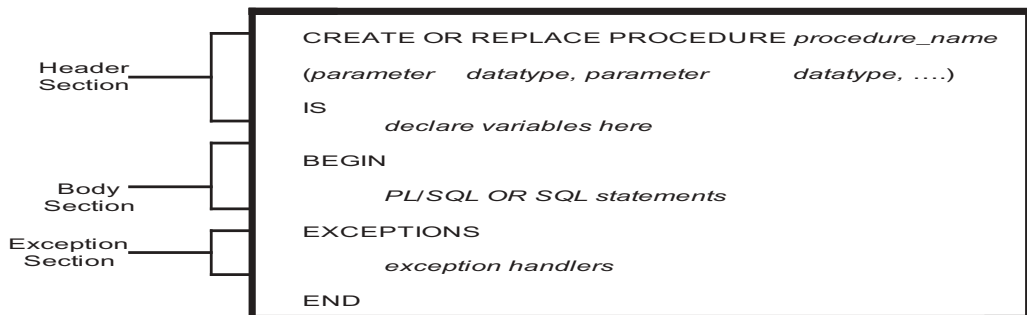
Figure 2.11. Syntax for creating a stored procedure in oracle.
