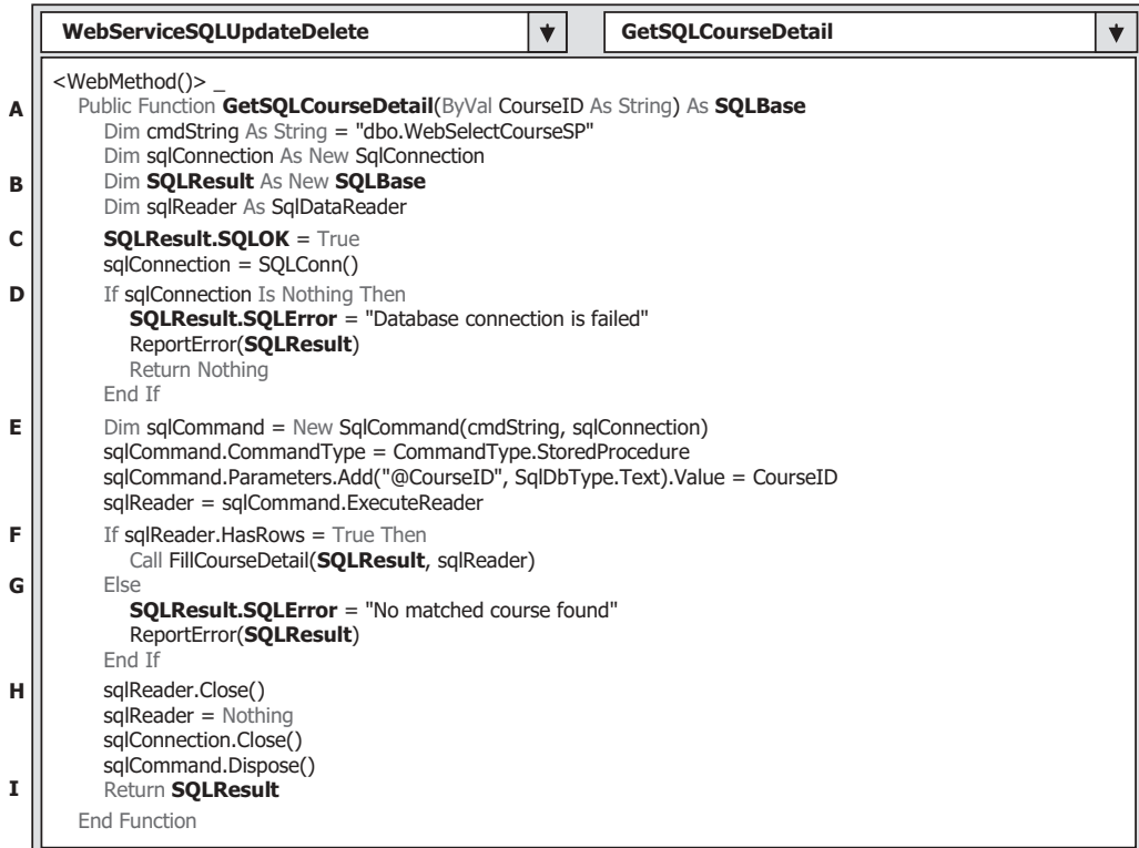
Figure 9.89. The modified codes for the Web method GetSQLCourseDetail() .
