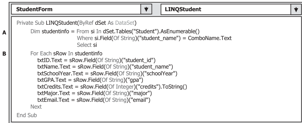
Figure 5.104. The codes for the subroutine LINQStudent.
