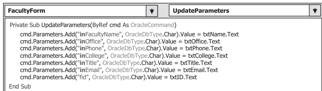
Figure 7.28. The modified codes for the subroutine UpdateParameters() .
