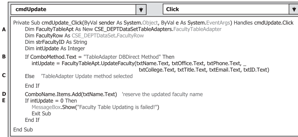
Figure 7.4. The codes for the Update command button's Click event procedure.
