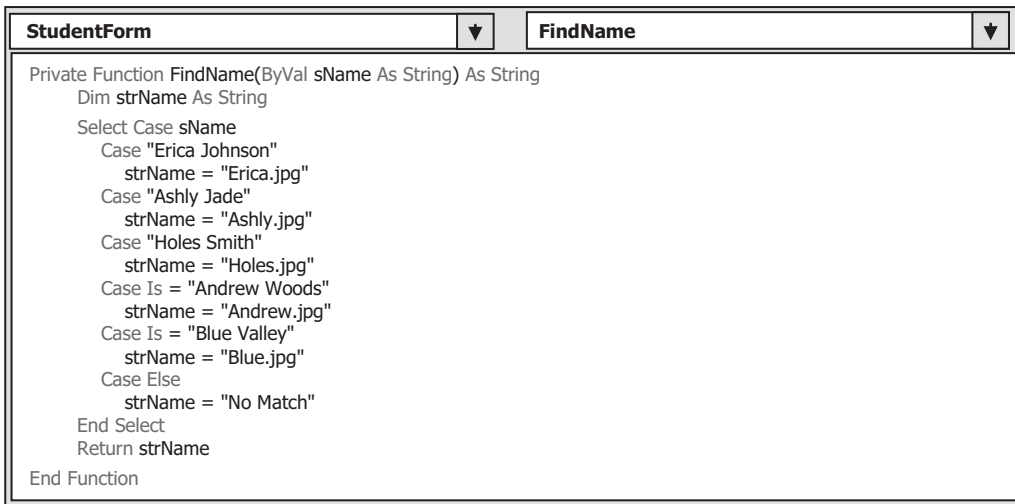
Figure 5.99. The codes for the subroutine FindName.
