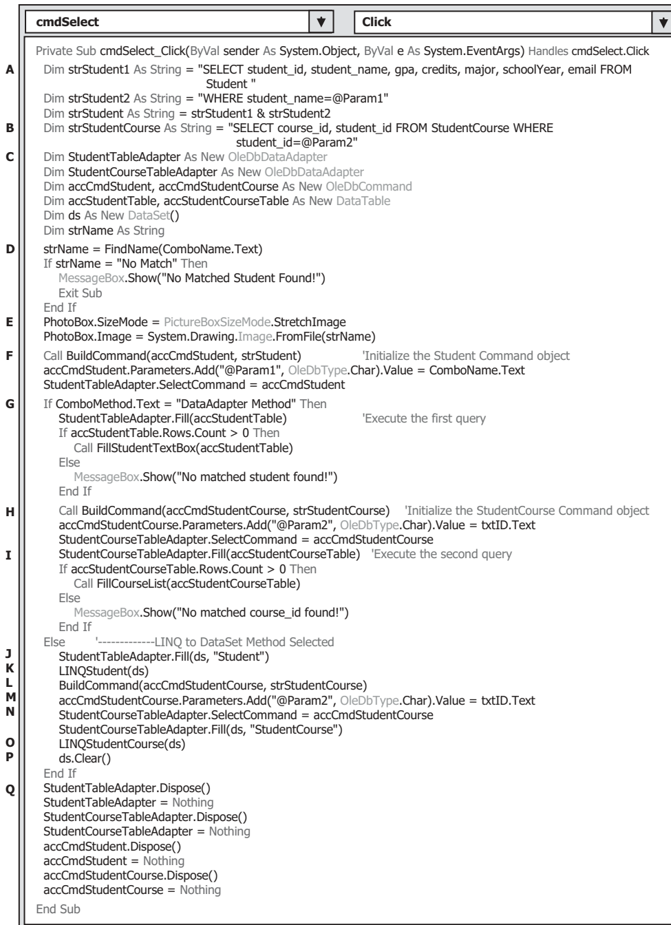
Figure 5.98. The codes for the Student Select button Click event procedure.
