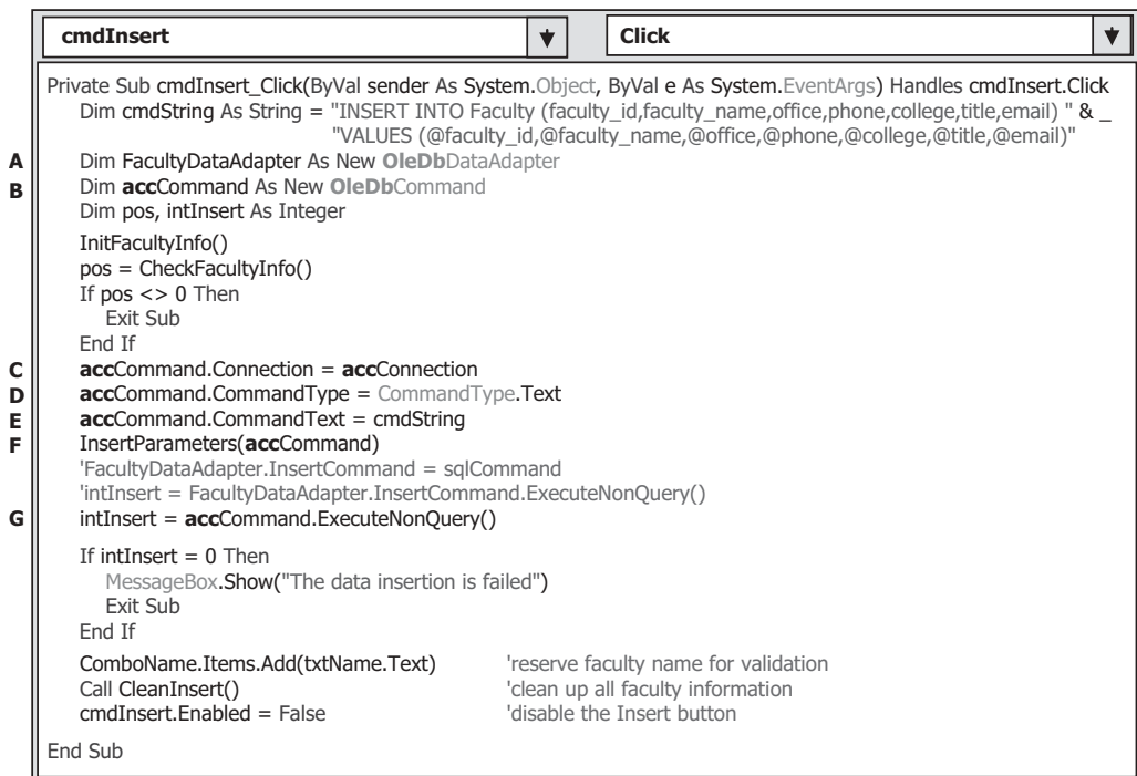
Figure 6.35. Modified codes for the Insert button Click event procedure.
