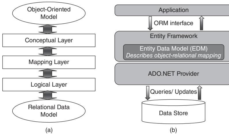
Figure 3.20. The mapping relationship between three layers.
