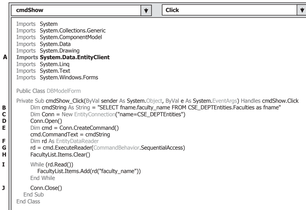
Figure 3.31. The codes for the cmdShow_Click event procedure.
