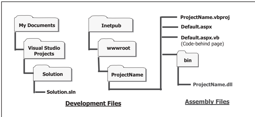
Figure 8.3. ASP.NET Web application file structure.
