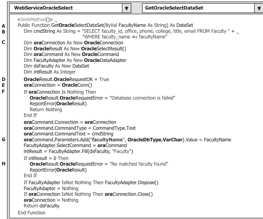
Figure 9.138. The modified Web method GetOracleSelectDataSet().
