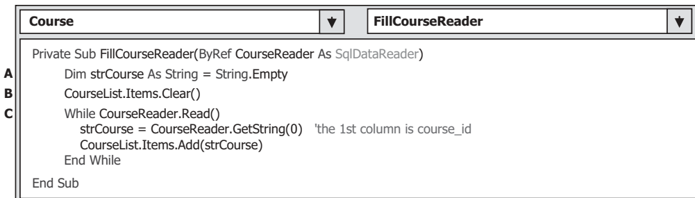
Figure 8.27. The codes for the subroutine FillCourseReader() .
