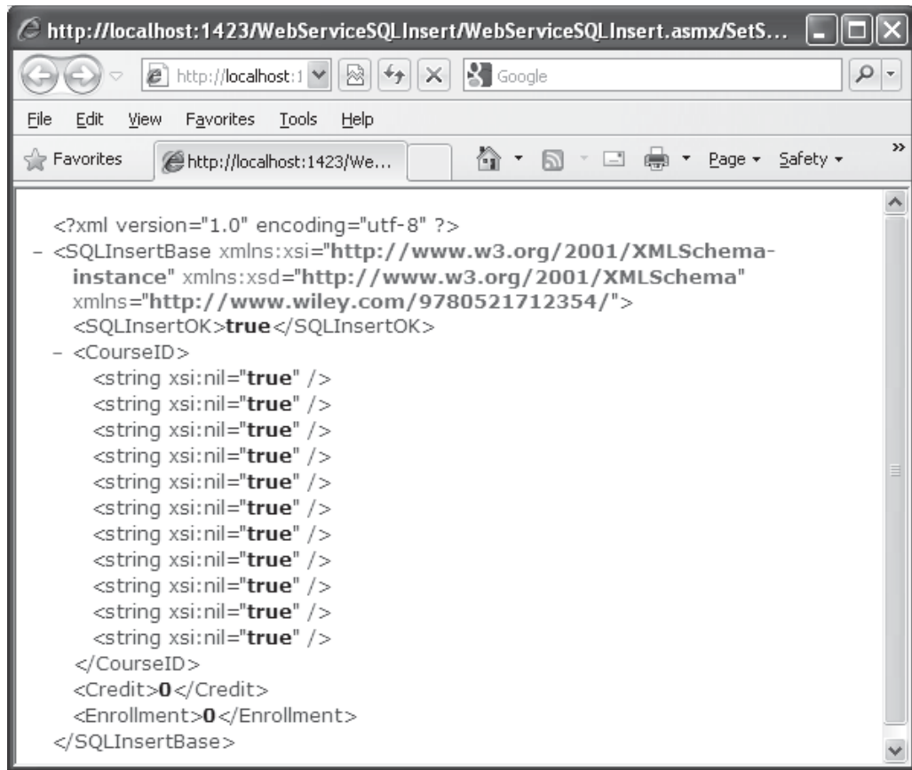
Figure 9.51. The running result of the first Web method.
