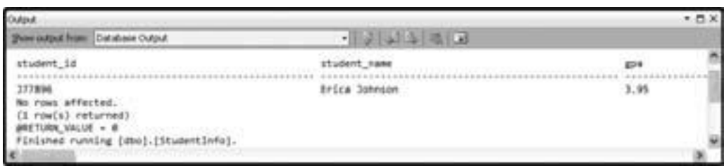
Figure 5.128. The testing result of our first stored procedure.
