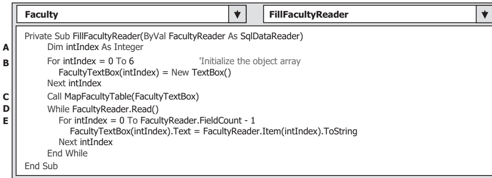
Figure 8.20. The codes for the subroutine FillFacultyReader.
