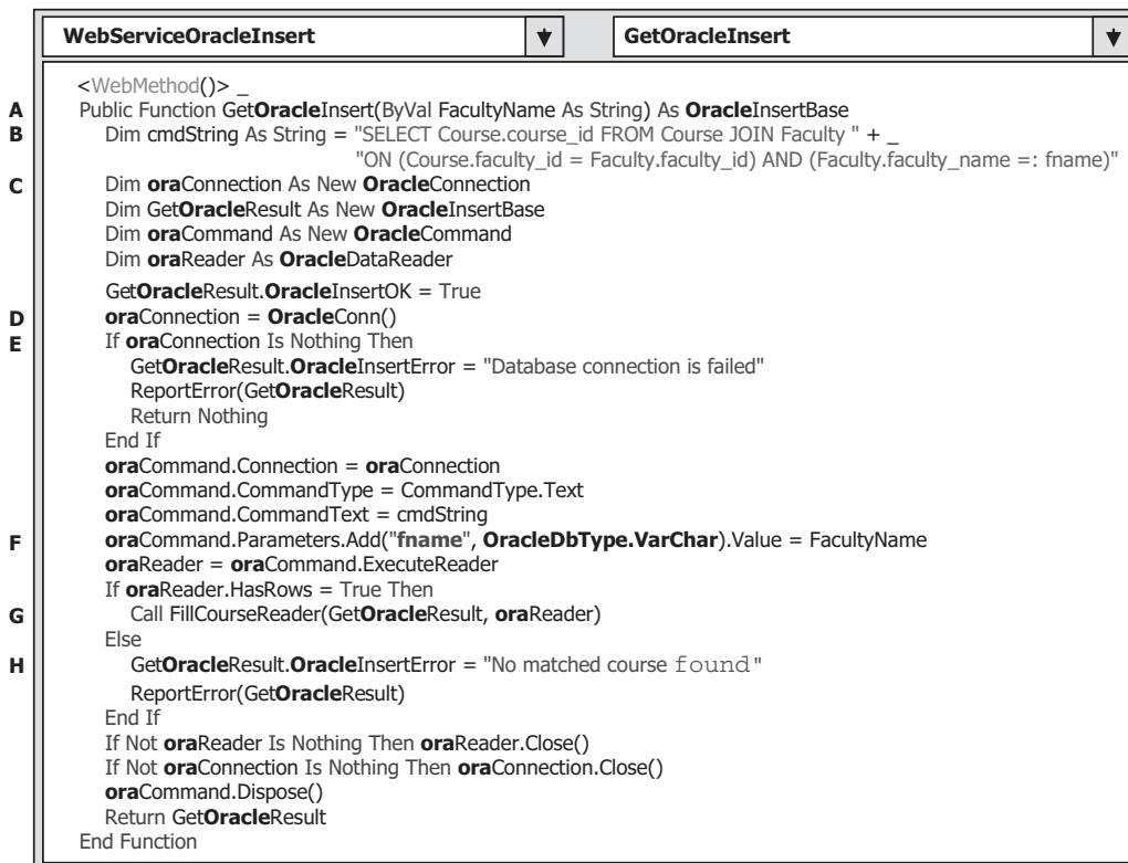
Figure 9.144. The modified Web method GetOracleInsert().
