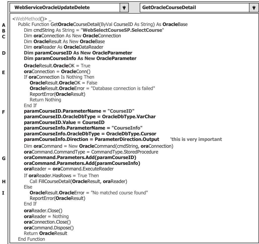
Figure 9.166. The modified Web method GetOracleCourseDetail().
