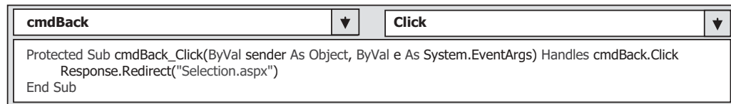
Figure 8.22. The codes for the Back button's Click event procedure.
