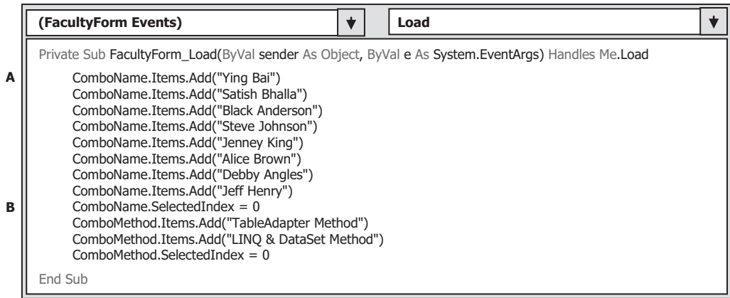
Figure 5.50. The codes for the FacultyForm_Load event procedure.
