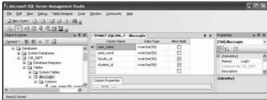
Figure 2.24. The new table window.
