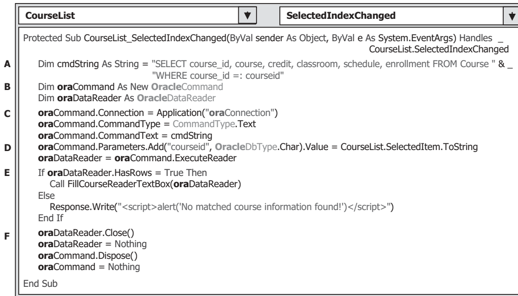
Figure 8.65. The modified SelectedIndexChanged event procedure.
