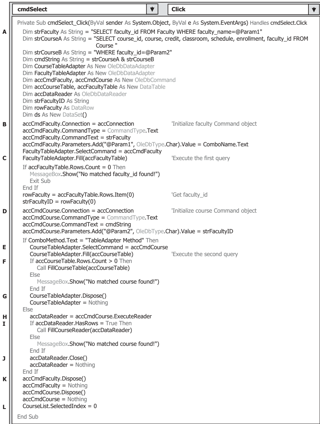
Figure 5.90. The codes for the Select button Click event procedure.
