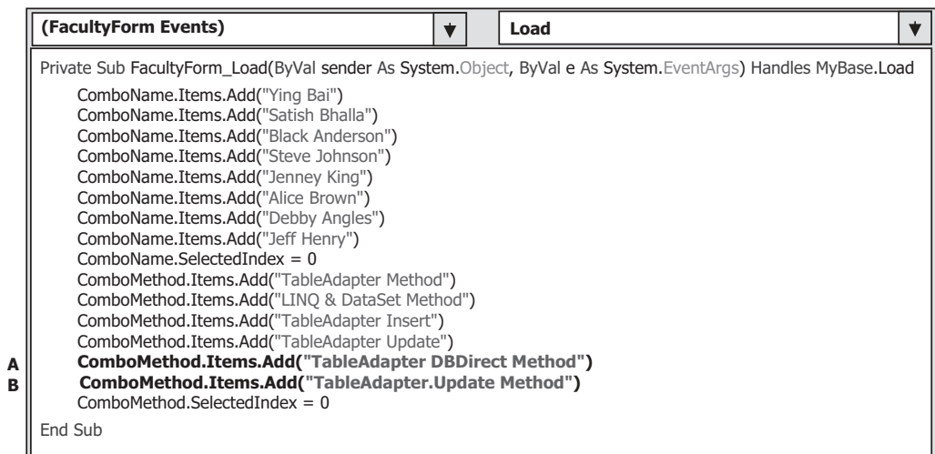
Figure 7.3. The modified codes for the Form_Load event procedure.
