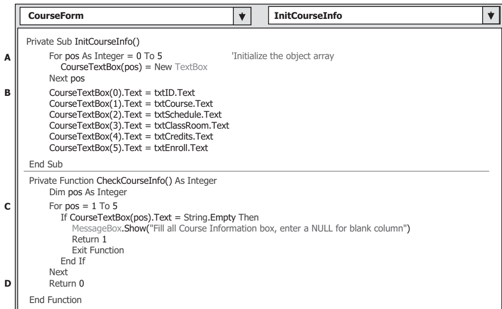
Figure 6.48. The codes for user-defined subroutine and function.
