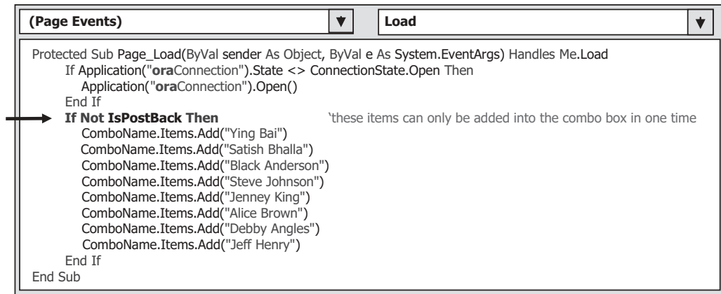
Figure 8.78. The codes for the Page_Load() event procedure.
