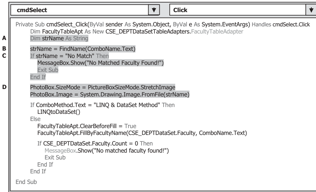
Figure 5.54. Add codes to select the faculty's image.
