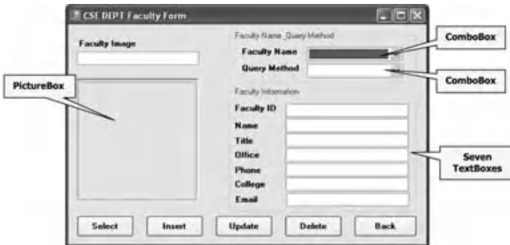
Figure 5.20. The finished Faculty form.
