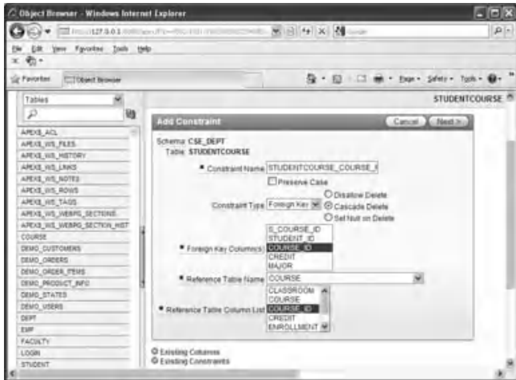
Figure 2.68. Create the foreign key between the StudentCourse and the Course table.
