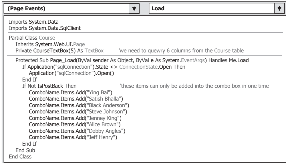
Figure 8.25. The codes for the Page_Load event procedure.
