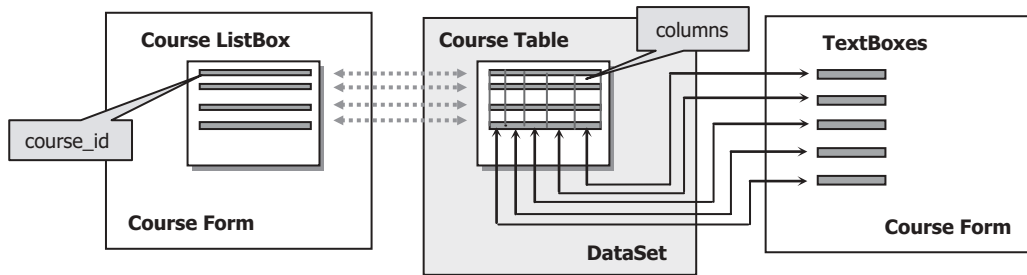
Figure 5.64. The relationships between Course ListBox, Course table and TextBox.
