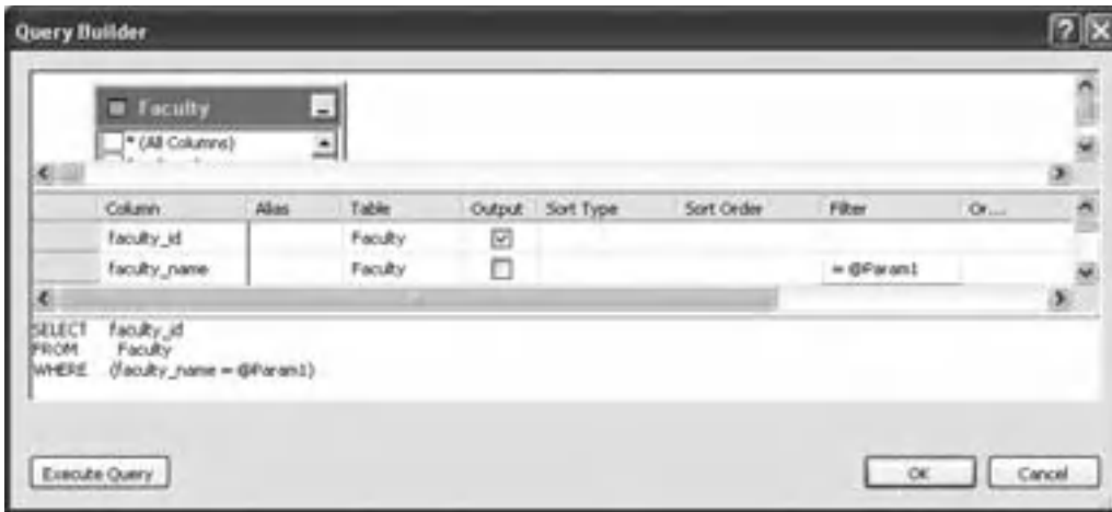
Figure 5.57. The finished query for the faculty_id.
