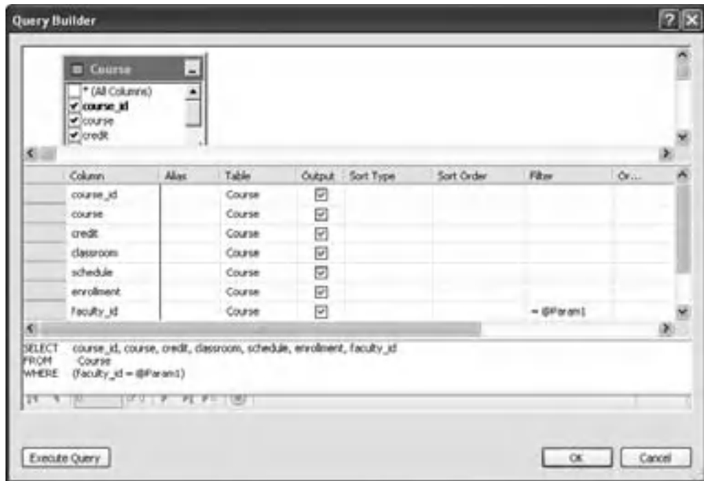
Figure 5.58. The Query Builder.
