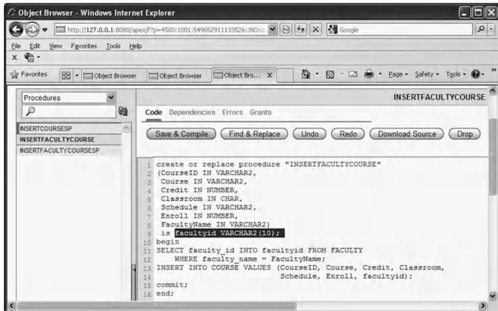
Figure 6.57. The completed stored procedure.
