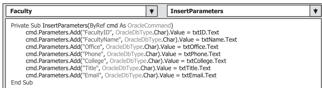
Figure 8.67. The codes for the subroutine InsertParameters() .
