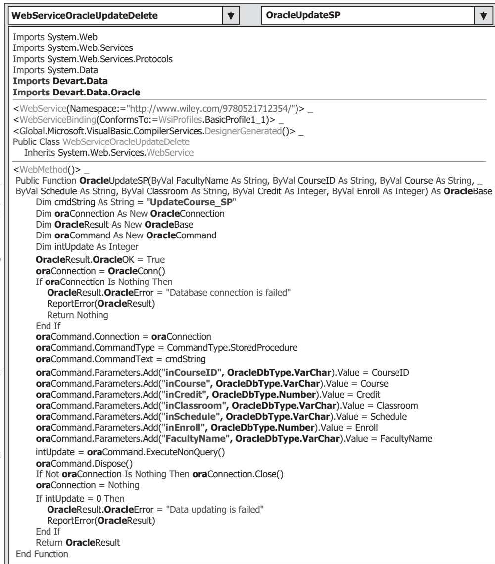
Figure 9.159. The modified Web method OracleUpdateSP().
