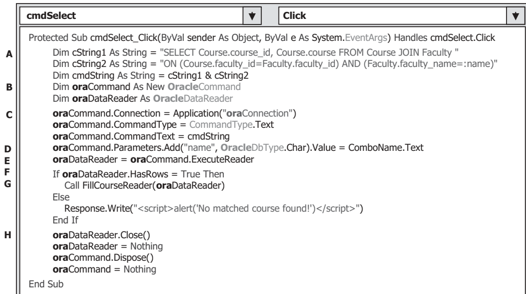
Figure 8.64. The modified Select button's Click event procedure.
