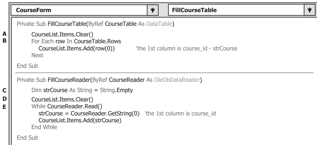
Figure 5.91. The codes for two user-defined subroutine procedures.
