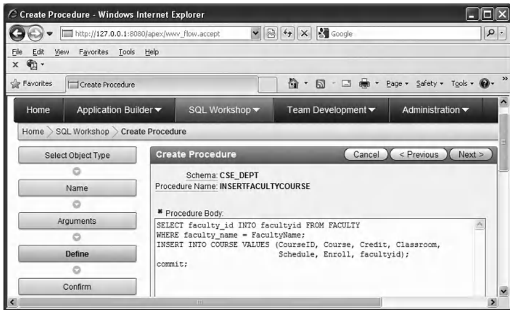
Figure 6.56. The stored procedure body.
