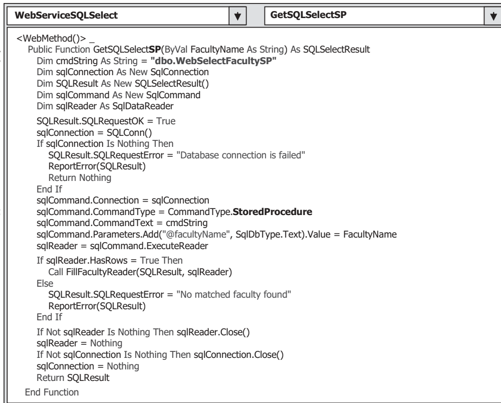
Figure 9.27. The modified Web method—GetSQLSelectSP().
