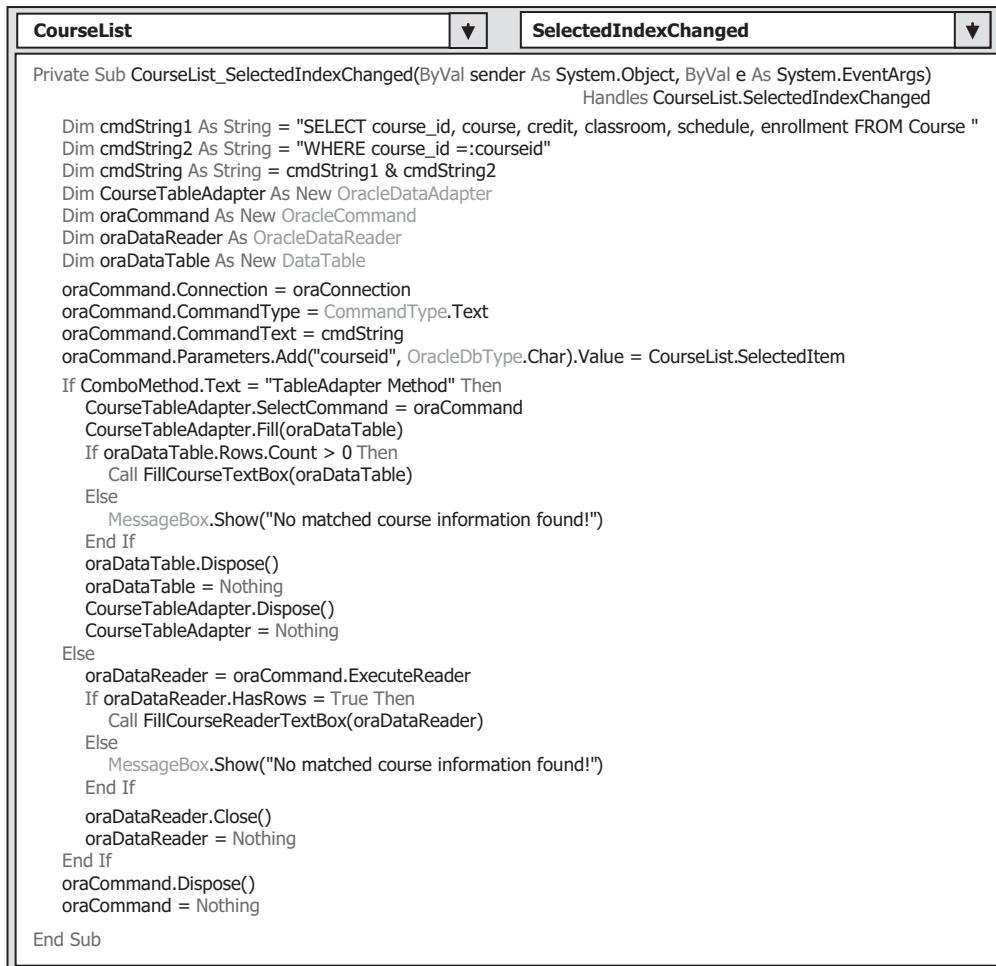
Figure 5.162. The codes for the SelectedIndexChanged event procedure.
