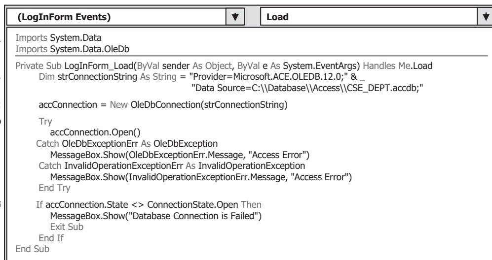
Figure 5.73. The codes for the LogInForm_Load event procedure.
