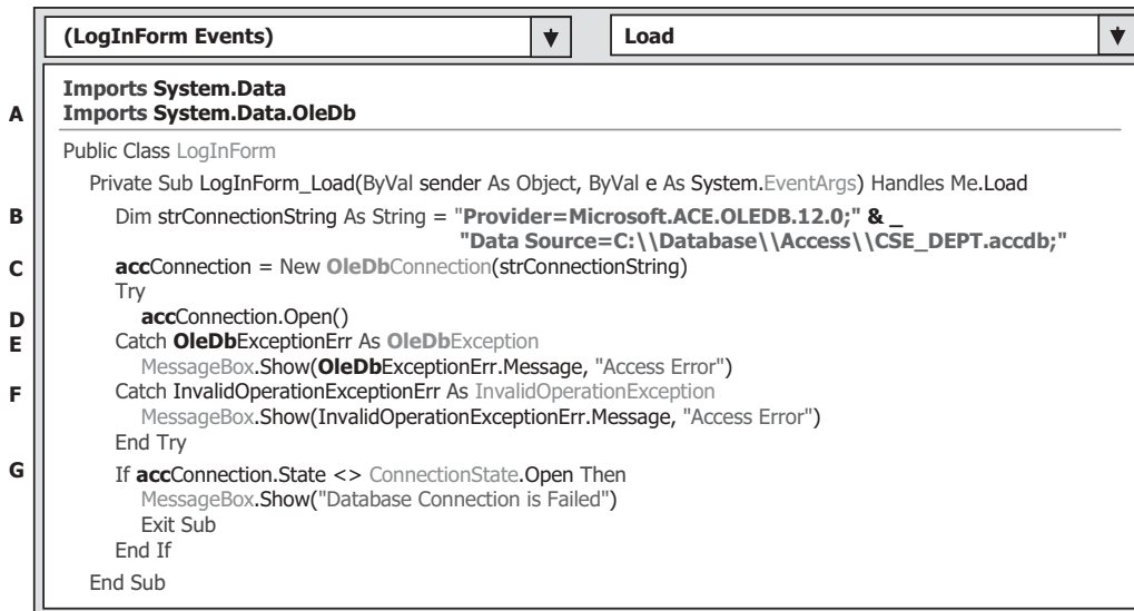
Figure 6.32. The modified codes to the Connection String.
