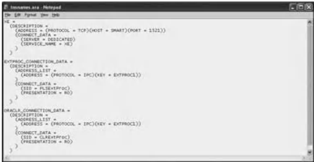
Figure 5.137. The sample of the file tnsnames.ora.
