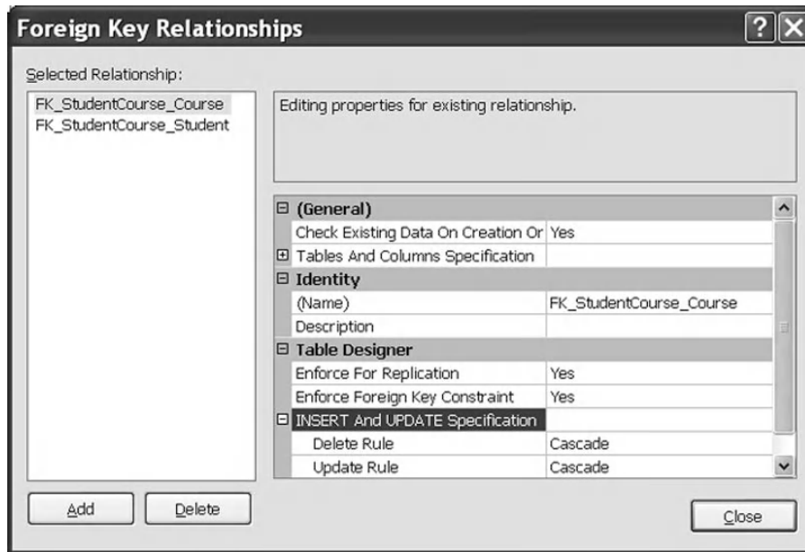
Figure 8.44. The Foreign Key Relationship wizard.
